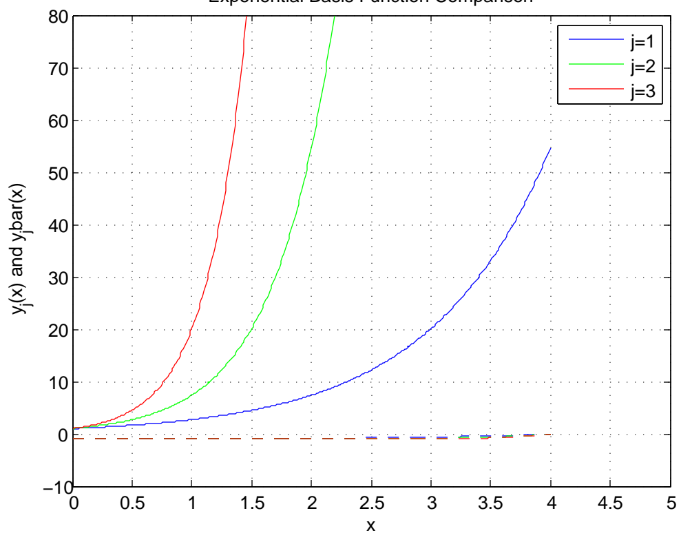
Exponential Basis Function Comparison
