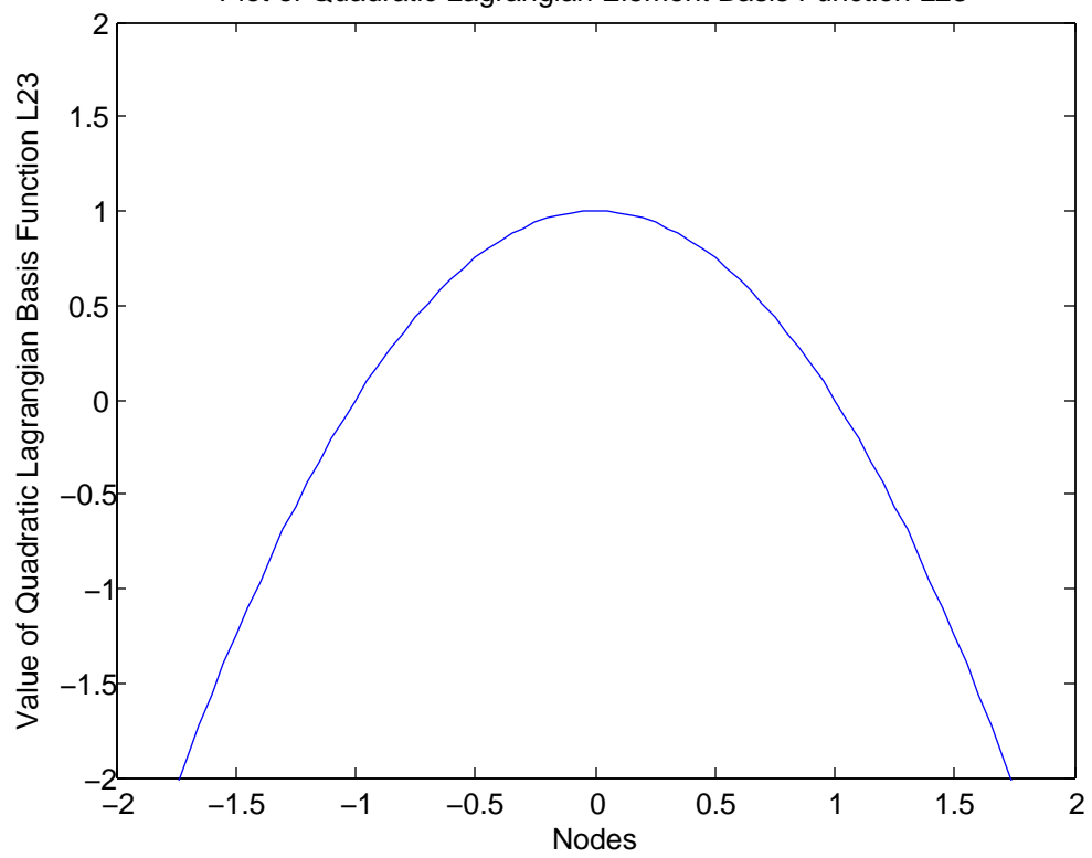
Plot of Quadratic Lagrangian Element Basis Function L23
