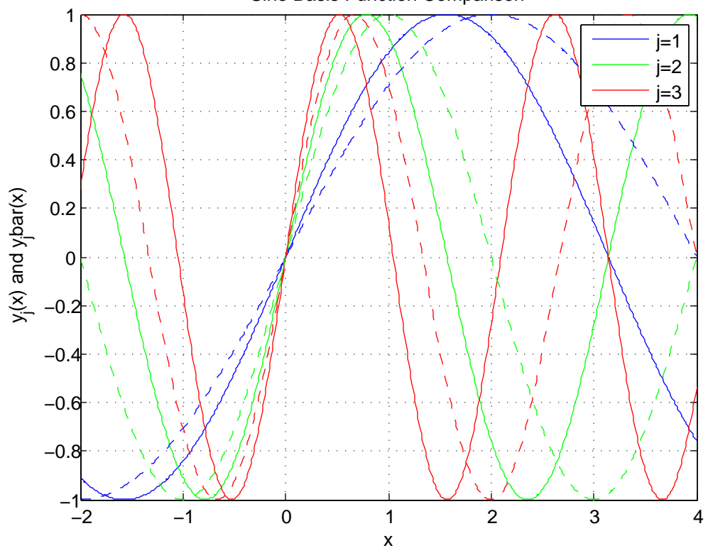
Sine Basis Function Comparison
