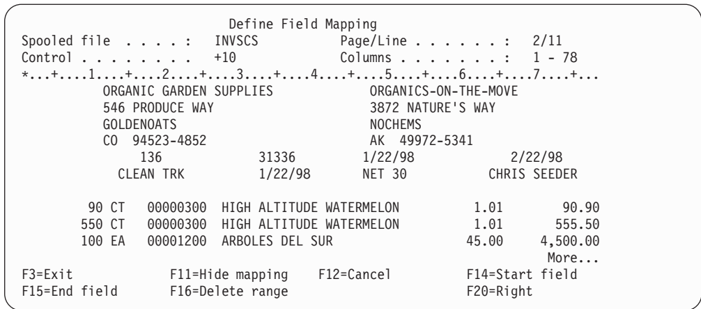
Figure 71. Define Field Mapping panel
