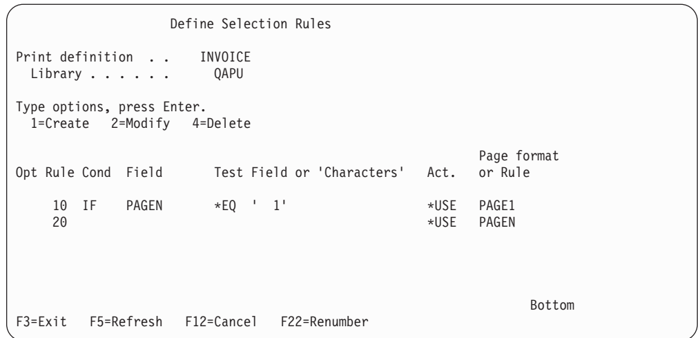
Figure 89. Define Selection Rules panel
