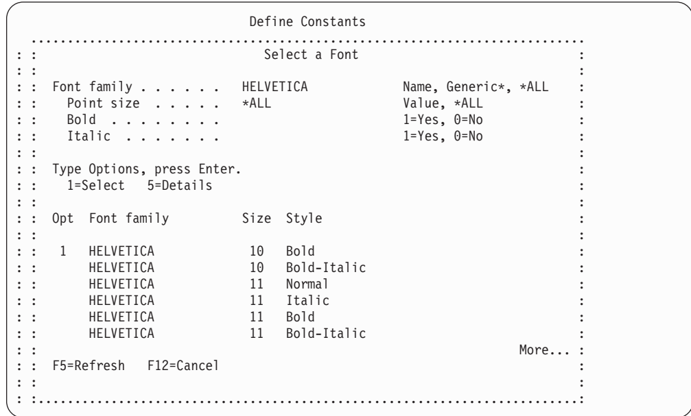
Figure 75. Select a Font panel
