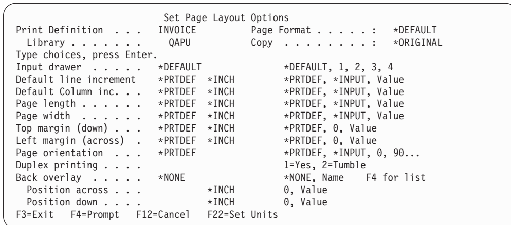
Figure 69. Set Page Layout Options panel
