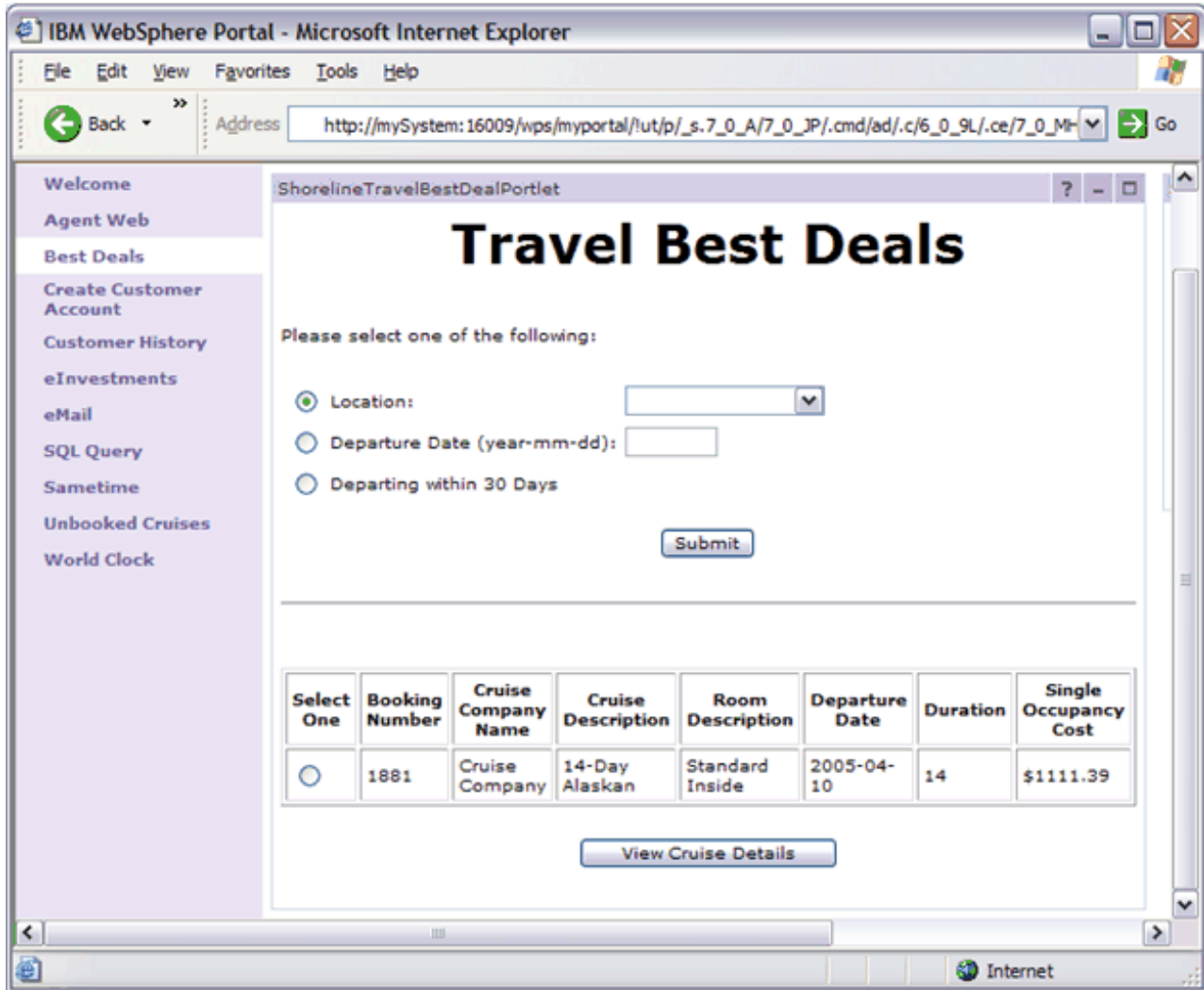
Figure 7. BestDeals portlet
