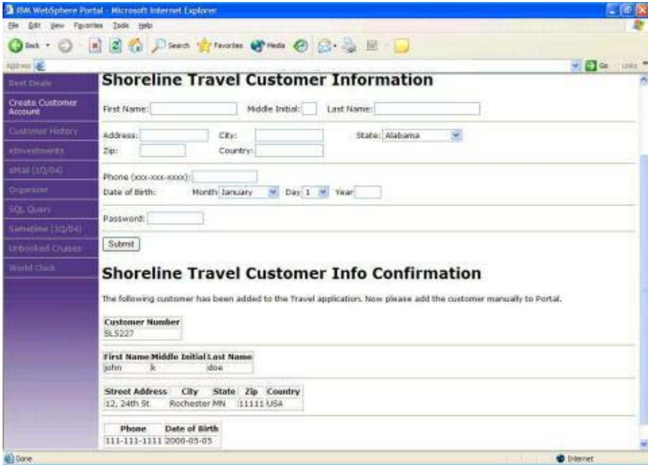
Figure 8. CreateCustomerAccount portlet
