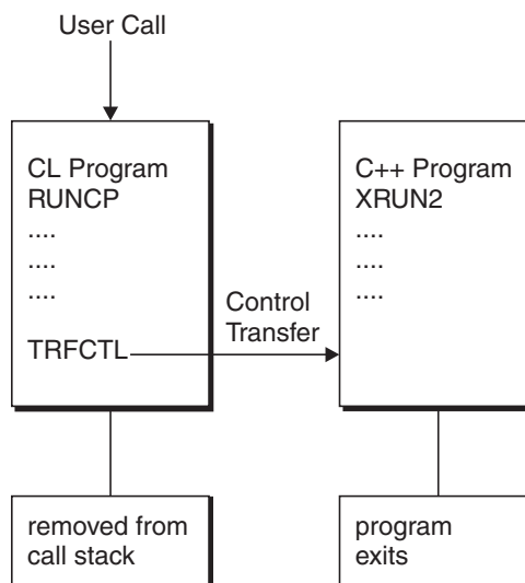
Figure 28. Calling Program XRUN2 Using the TFRCTL Command
