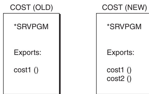
Figure 23. Exports from Service Program COST
