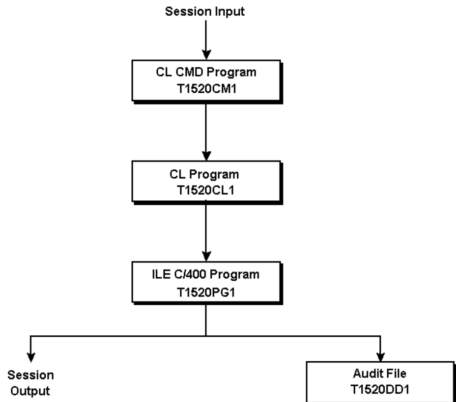
Figure 51. Sample Application: High-Level Input/Processing/Output Flow
