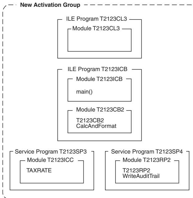
Figure 238. Basic Object Structure
