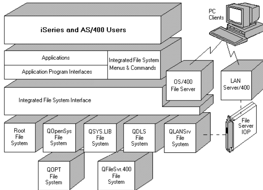
Figure 104. The Integrated File System Interface
