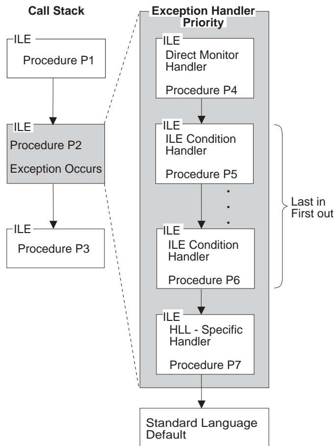
Figure 183. Exception Handler Priority
