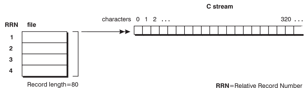
Figure 83. iSeries Data Management Records Mapping to an ILE C Stream File
