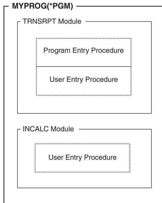
Figure 3. Structure of Program MYPROG
