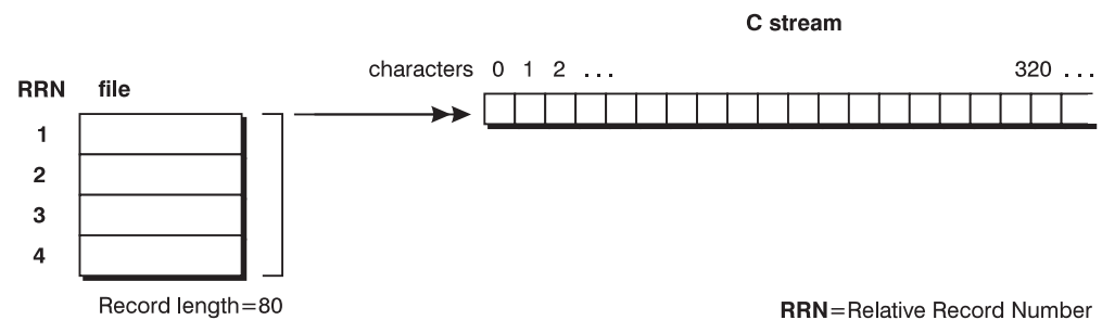
Figure 106. iSeries Records Mapping to a C/C++ Stream File
