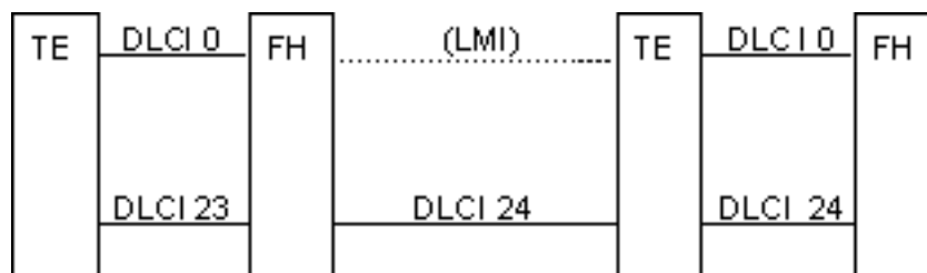
Figure 5. Example of DLCI Assignments for PVC Connections
