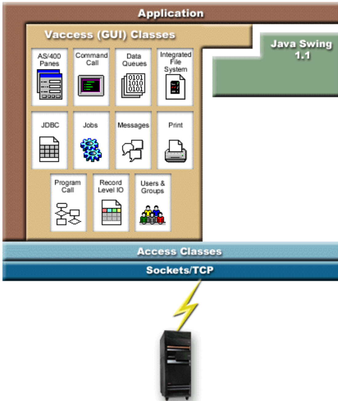
description of Figure 1: Vaccess classes (rzahh508.gif)" on page 249
