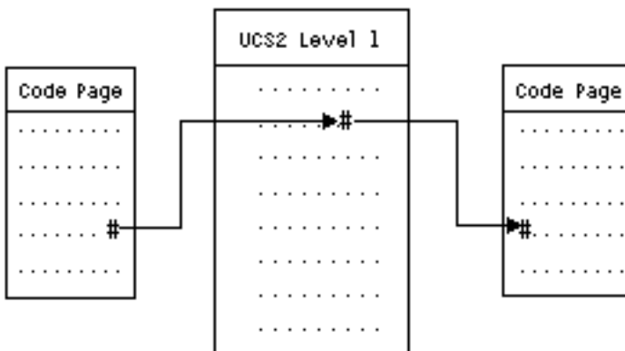
Figure 8. Keeping characters the same across encoding schemes
