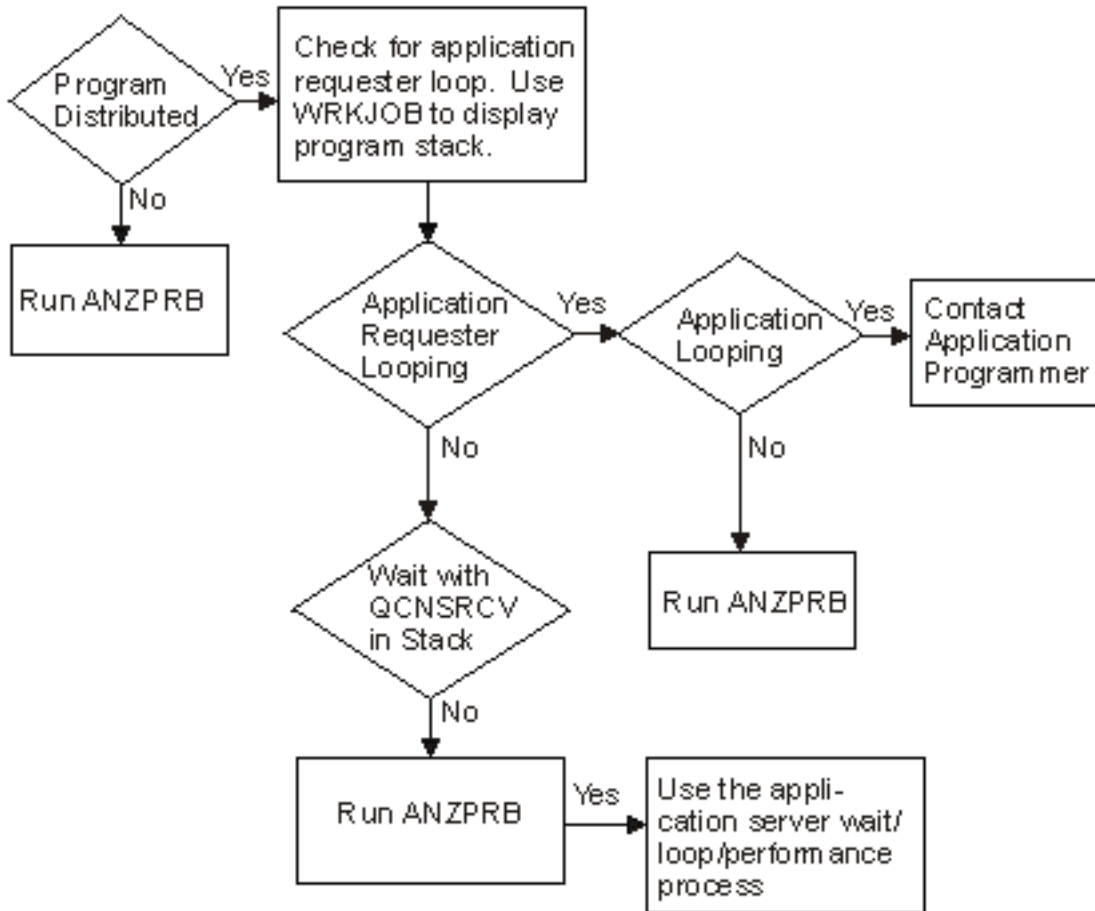
Figure 15. Resolving Wait, Loop, or Performance Problems on the Application Requester
