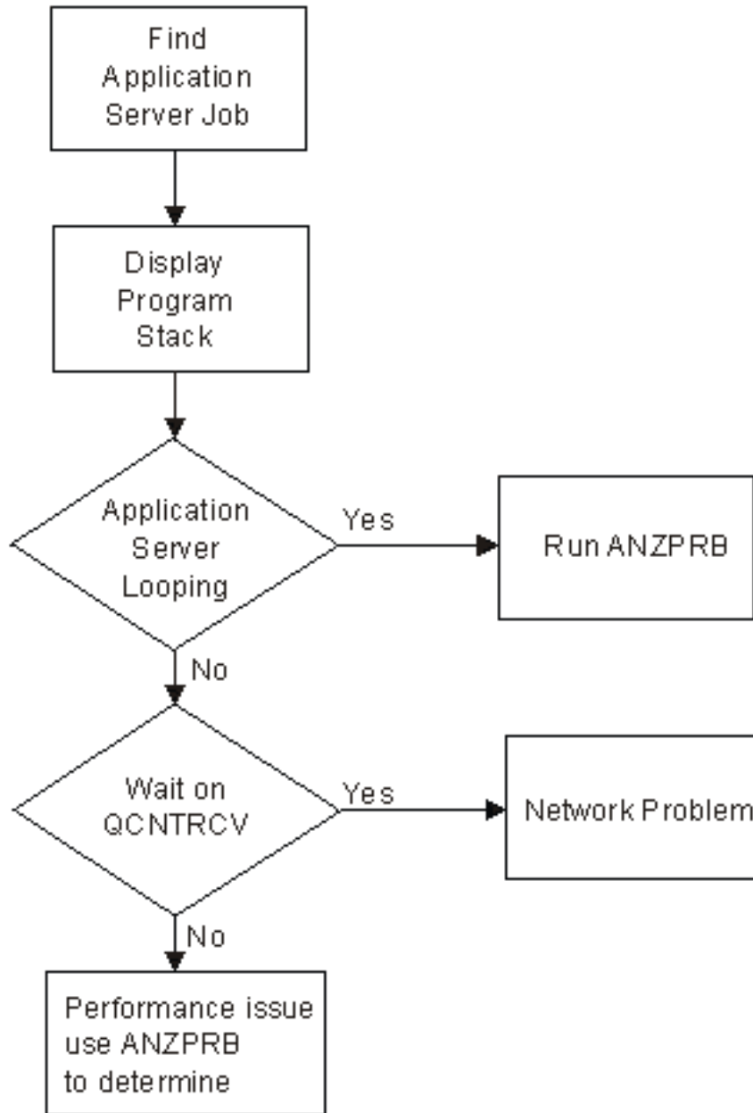
Figure 16. Resolving Wait, Loop, or Performance Problems on the Application Server
