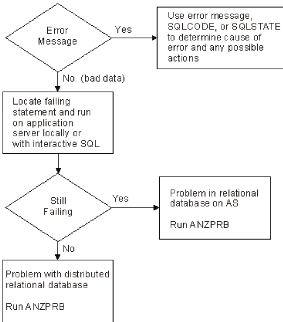
Figure 14. Resolving Incorrect Output Problem
