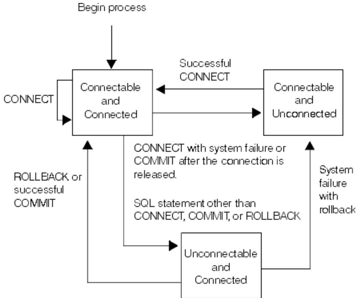
Figure 19. Remote Unit of Work Activation Group Connection State Transition
