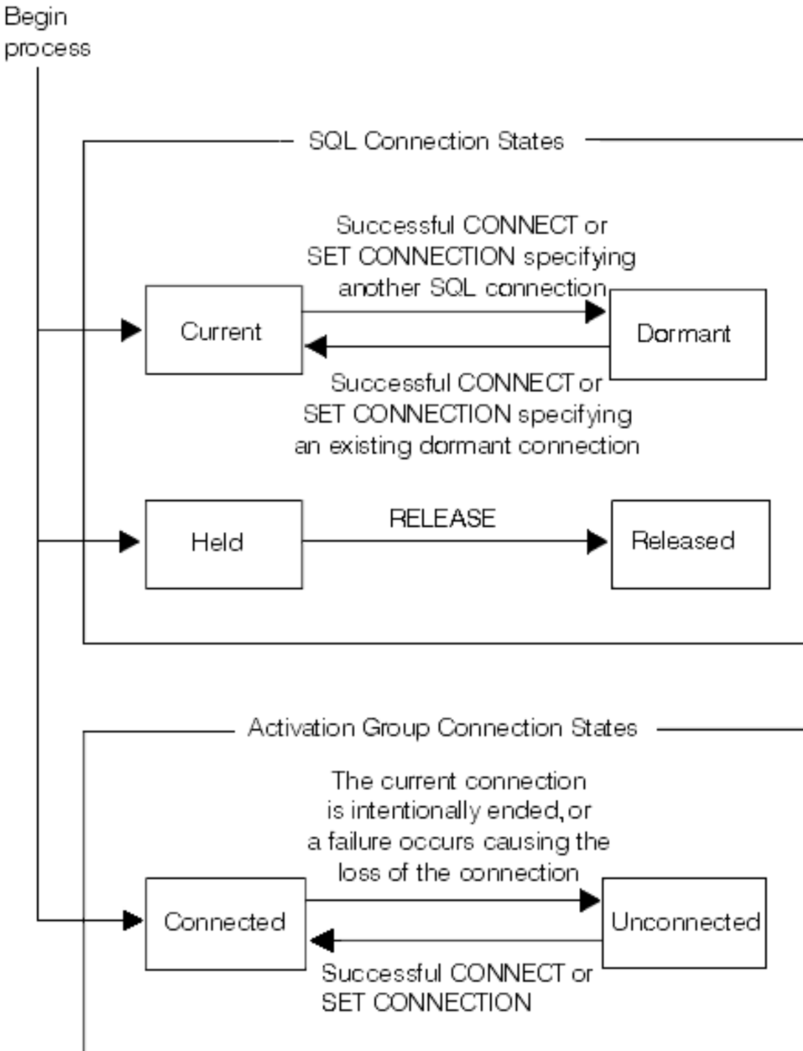
Figure 20. Application-Directed Distributed Unit of Work Connection and Activation Group Connection State Transitions
