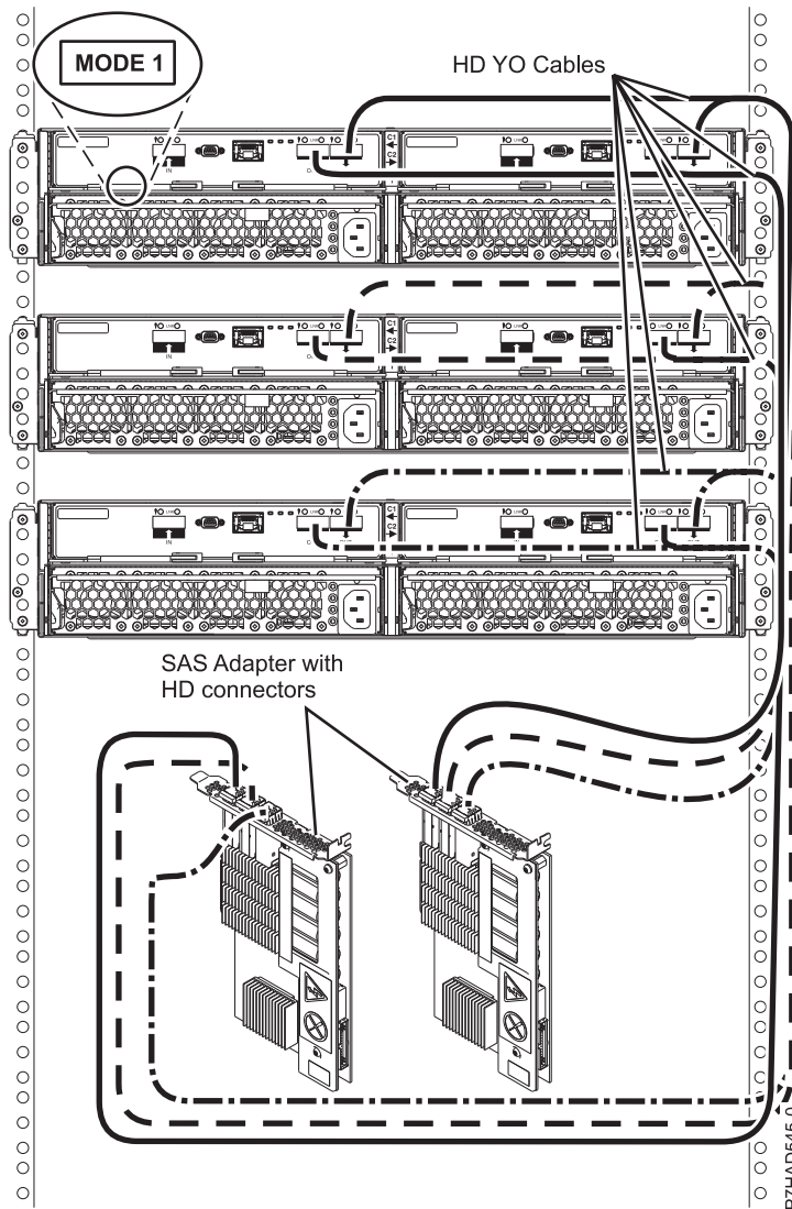
Figure 84. Mode 1 connection of three 5887 enclosures to two PCIe2 SAS adapters with HD connectors
