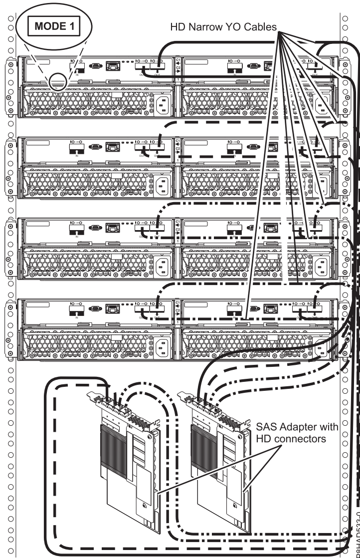
Figure 89. Mode 1 connection of four 5887 enclosures to two PCIe3 SAS adapters with HD narrow connectors.
