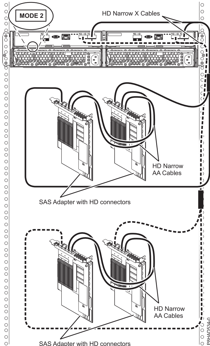
Figure 90. Mode 2 connection of a 5887 enclosure to two pairs of PCIe3 SAS adapters with HD narrow connectors.
