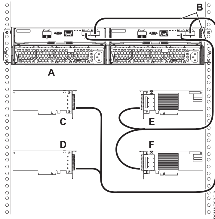
Figure 91. Mode 4 connection of a 5887 enclosure by using X cables to four single PCIe3 SAS adapters with HD narrow connectors.
