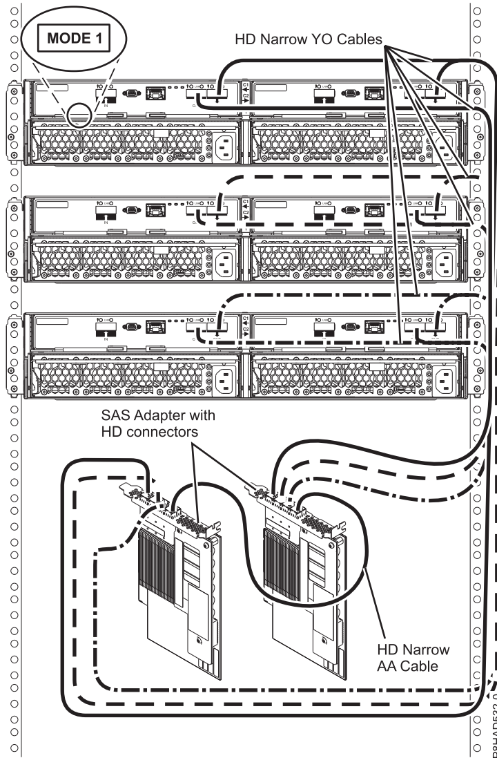
Figure 88. Mode 1 connection of three 5887 enclosures to two PCIe3 SAS adapters with HD narrow connectors.
