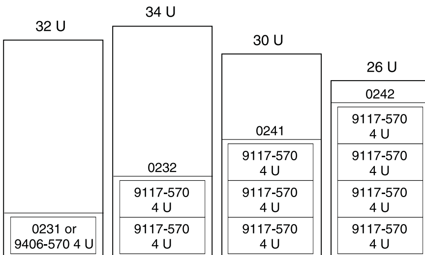
Figure 7. 570 in rack
