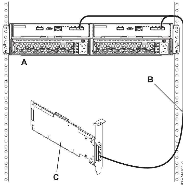
Figure 75. Mode 1 connection of a 5887 enclosure by using a YO cable to a single SAS adapter
