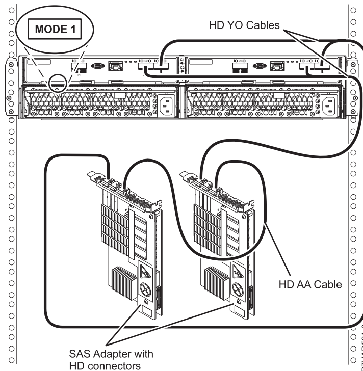
Figure 82. Mode 1 connection of a 5887 enclosure to two PCIe2 SAS adapters with HD connectors
