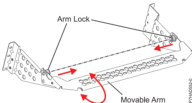
Figure 53. Cable management bracket
