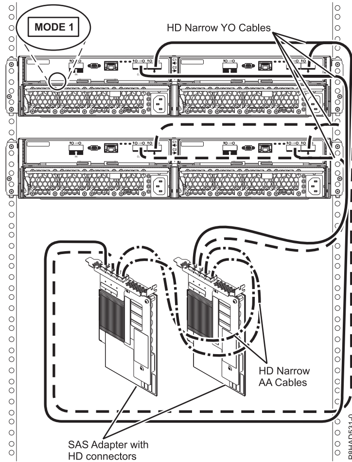
Figure 87. Mode 1 connection of two 5887 enclosures to two PCIe3 SAS adapters with HD narrow connectors.
