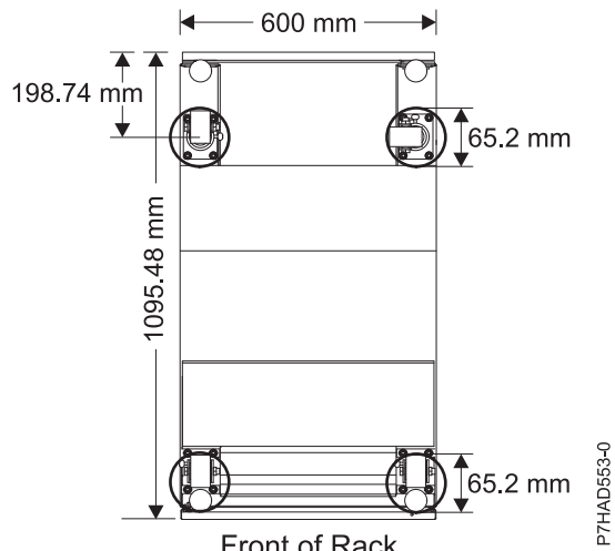
Figure 26. Caster locations
