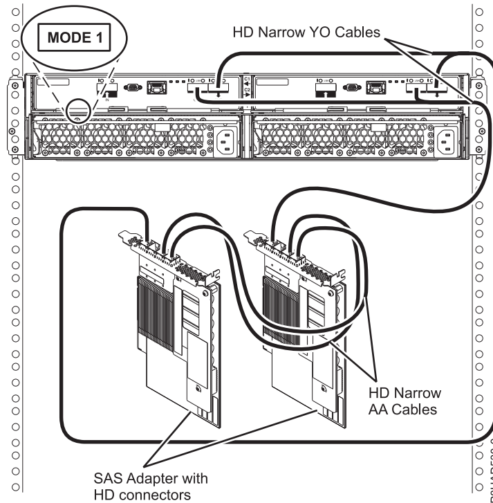
Figure 86. Mode 1 connection of a 5887 enclosure to two PCIe3 SAS adapters with HD narrow connectors.
