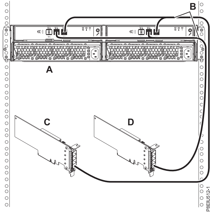
Figure 96. Mode 2 connection of ESLL or ESLS storage enclosure by using YO12 cables to two independent SAS adapters
