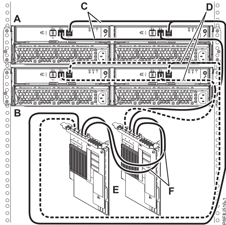
Figure 95. Mode 1 connection of two ESLL or ESLS storage enclosures by using YO12 cables to one pair of SAS adapters
