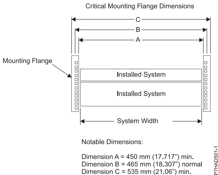
Figure 44. Critical mounting flange dimensions
