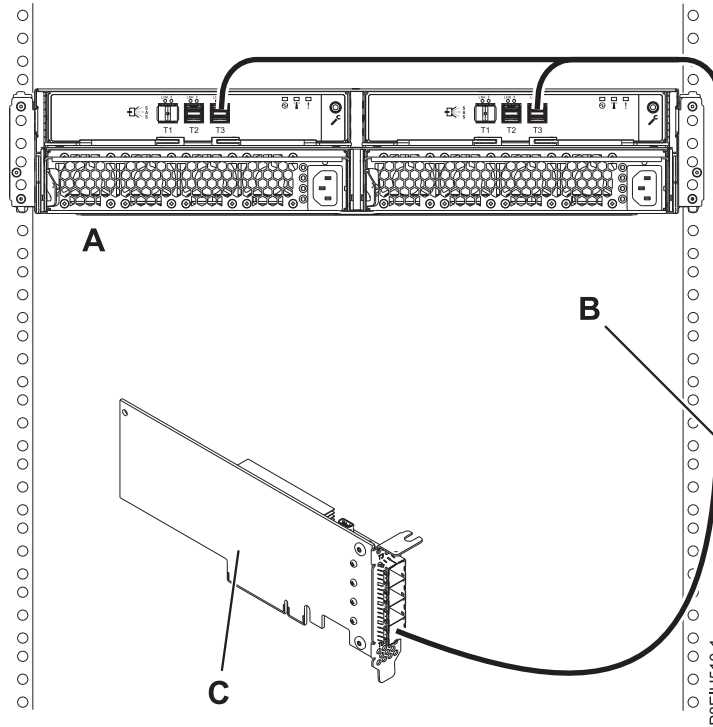
Figure 92. Mode 1 connection of one ESLL or ESLS storage enclosure by using a YO12 cable to a single SAS adapter
