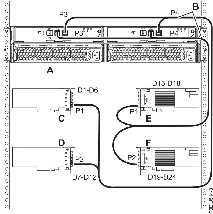
Figure 99. Mode 4 connection of one ESSL or ESLS storage enclosure by using X12 cables to four independent SAS adapters
