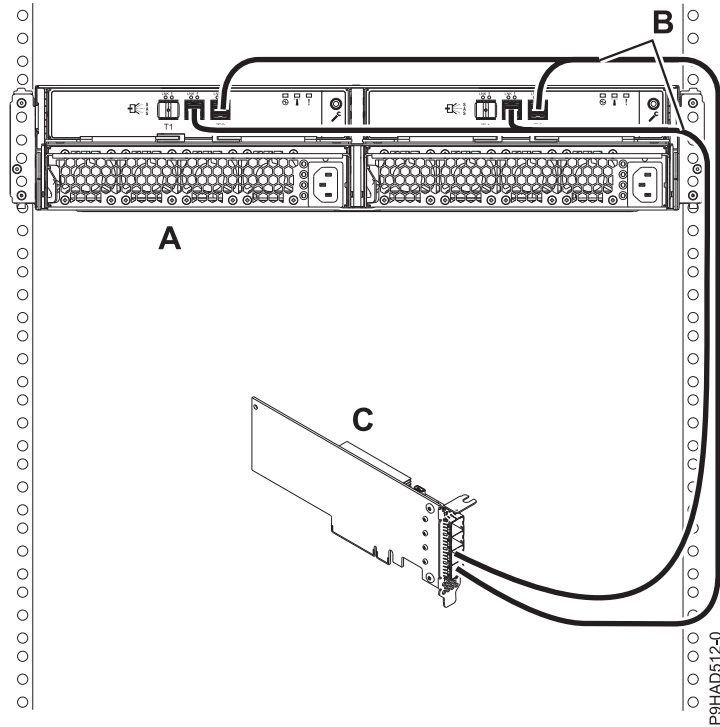
Figure 97. Mode 2 connection of ESLL or ESLS storage enclosure by using YO12 cables to a single SAS adapter
