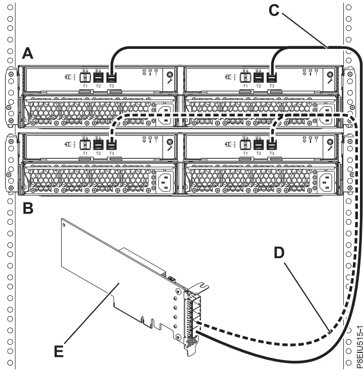
Figure 93. Mode 1 connection of two ESLL or ESLS storage enclosures by using YO12 cables to a single SAS adapter
