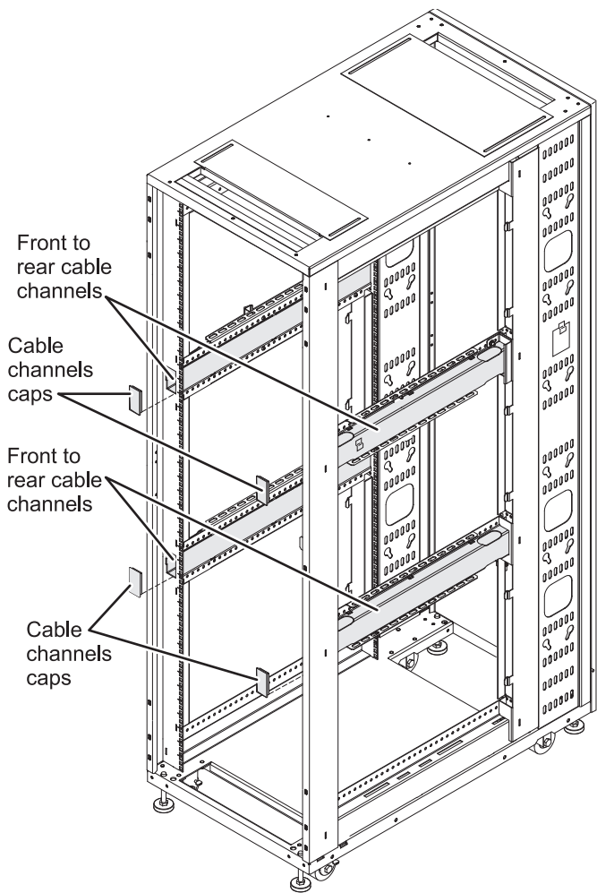
Figure 27. Cabling within the rack
