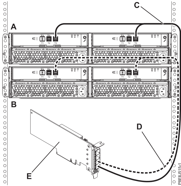
Figure 93. Mode 1 connection of two ESLL or ESLS storage enclosures by using YO12 cables to a single SAS adapter
