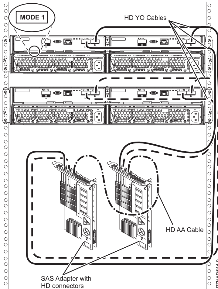
Figure 83. Mode 1 connection of two 5887 enclosures by using HD connectors to two PCIe2 SAS adapters
