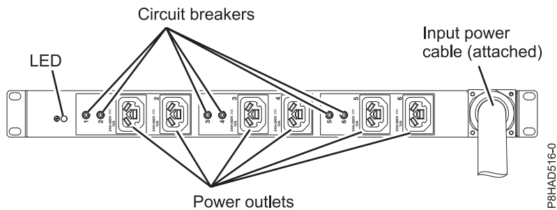
Figure 50. HVDC PDU
