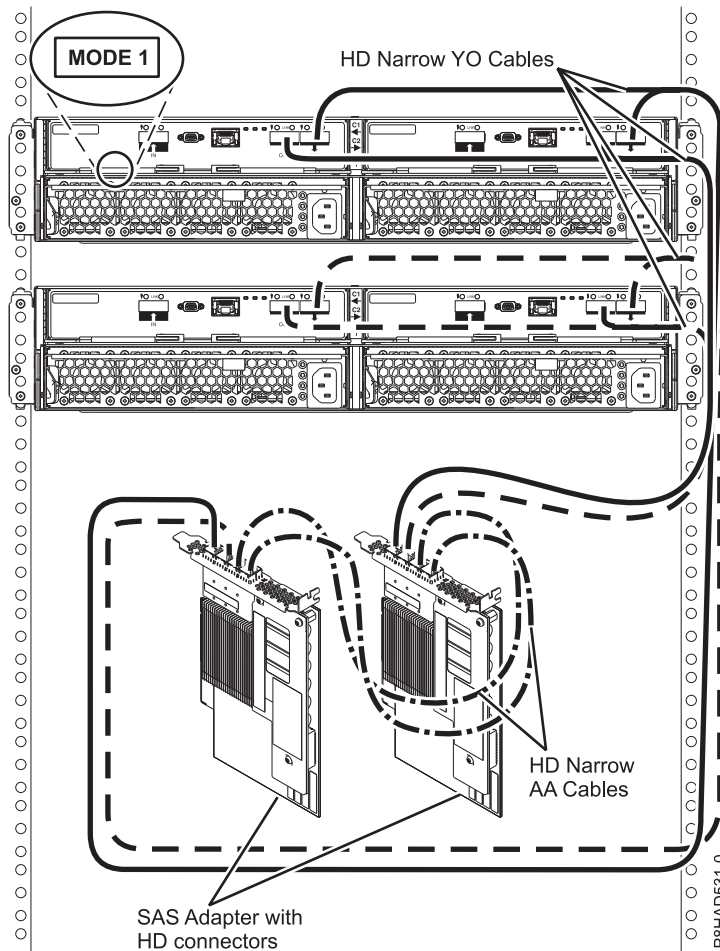
Figure 87. Mode 1 connection of two 5887 enclosures to two PCIe3 SAS adapters with HD narrow connectors.
