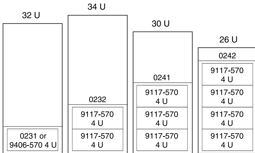
Figure 7. 570 in rack
