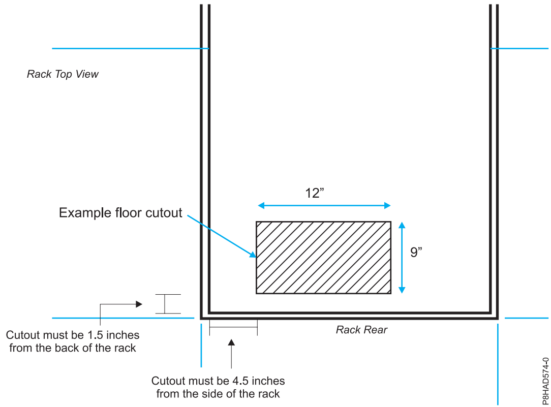
Figure 35. Floor cutout
