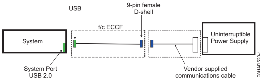
Figure 46. UPS wiring for the 5148-21L, 5148-22L, 8247-21L, 8247-21L, 8247-22L, 8247-42L, 8284-22A, 8286-41A, and 8286-42A
