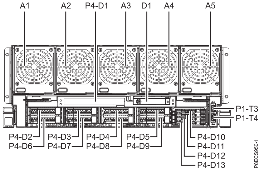
Figure 19. Front view
