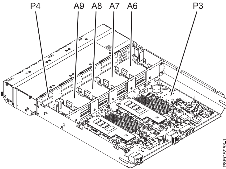
Figure 22. Assembly view
