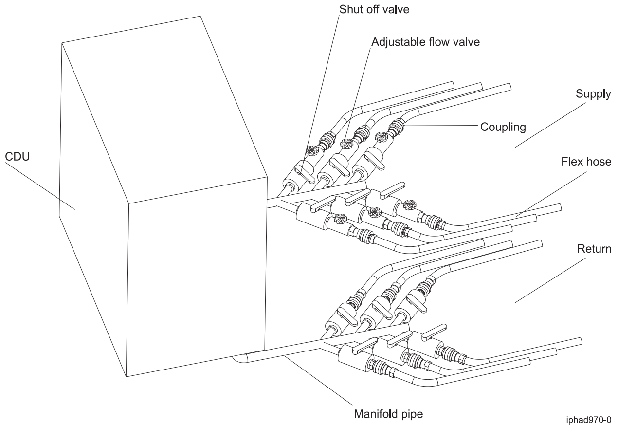
Figure 20. Typical central distribution manifold layout in a central location
