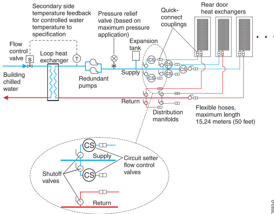
Figure 16. Coolant distribution using a facility water delivery system
