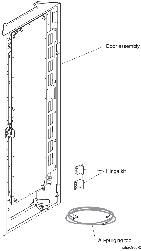
Figure 12. Components of the heat exchanger kit for 19-inch EIA-rail racks
