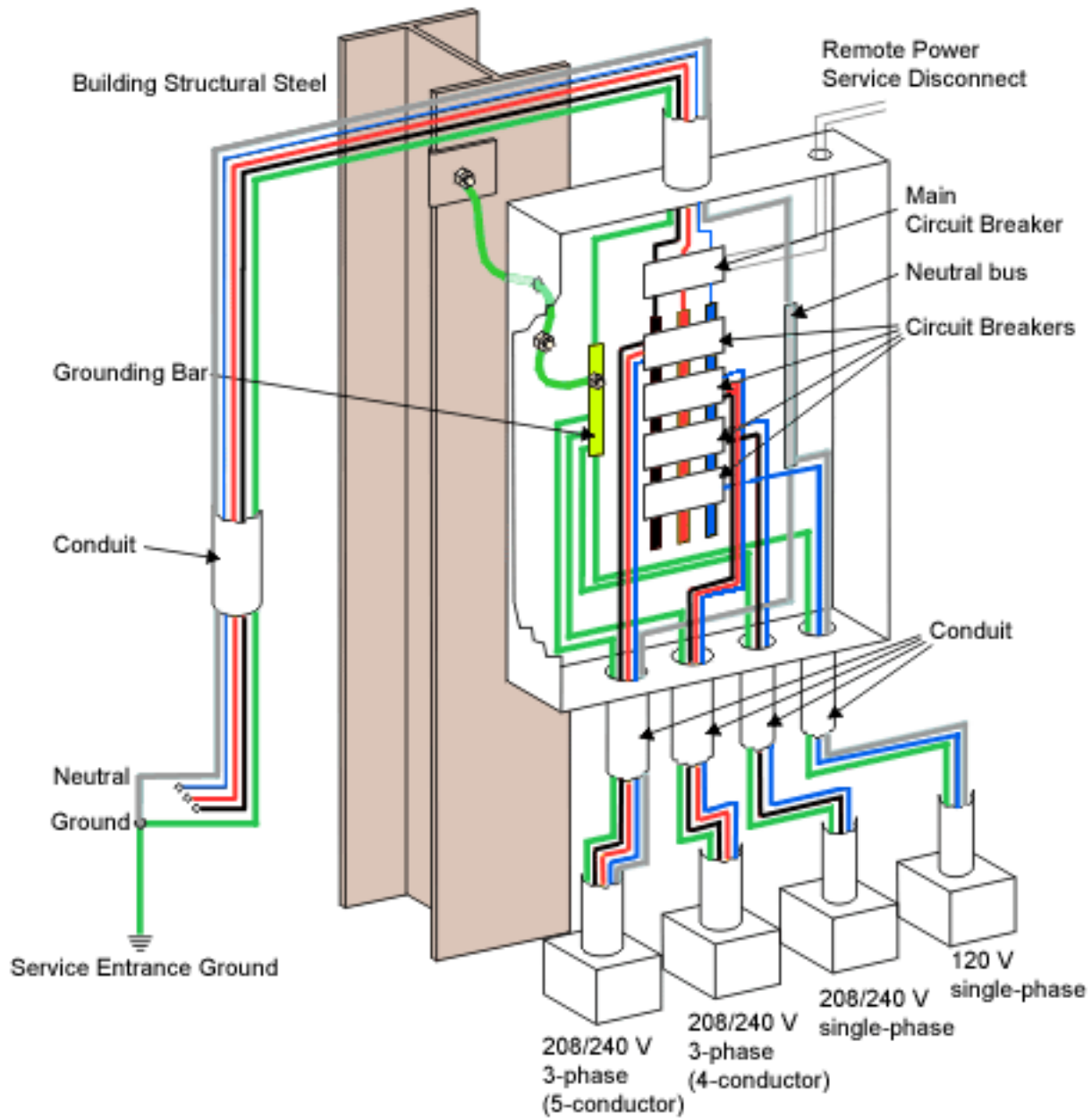
Figure 34. Transient grounding plate
