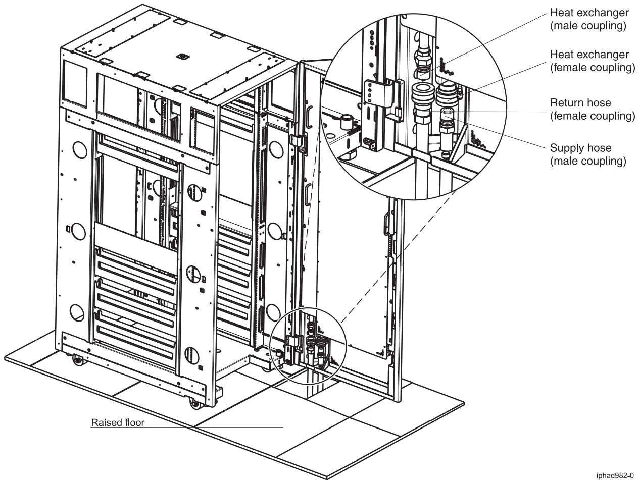
Figure 24. Raised floor hose management example 1; tile cut out size and position for 24-inch EIA-rail racks
