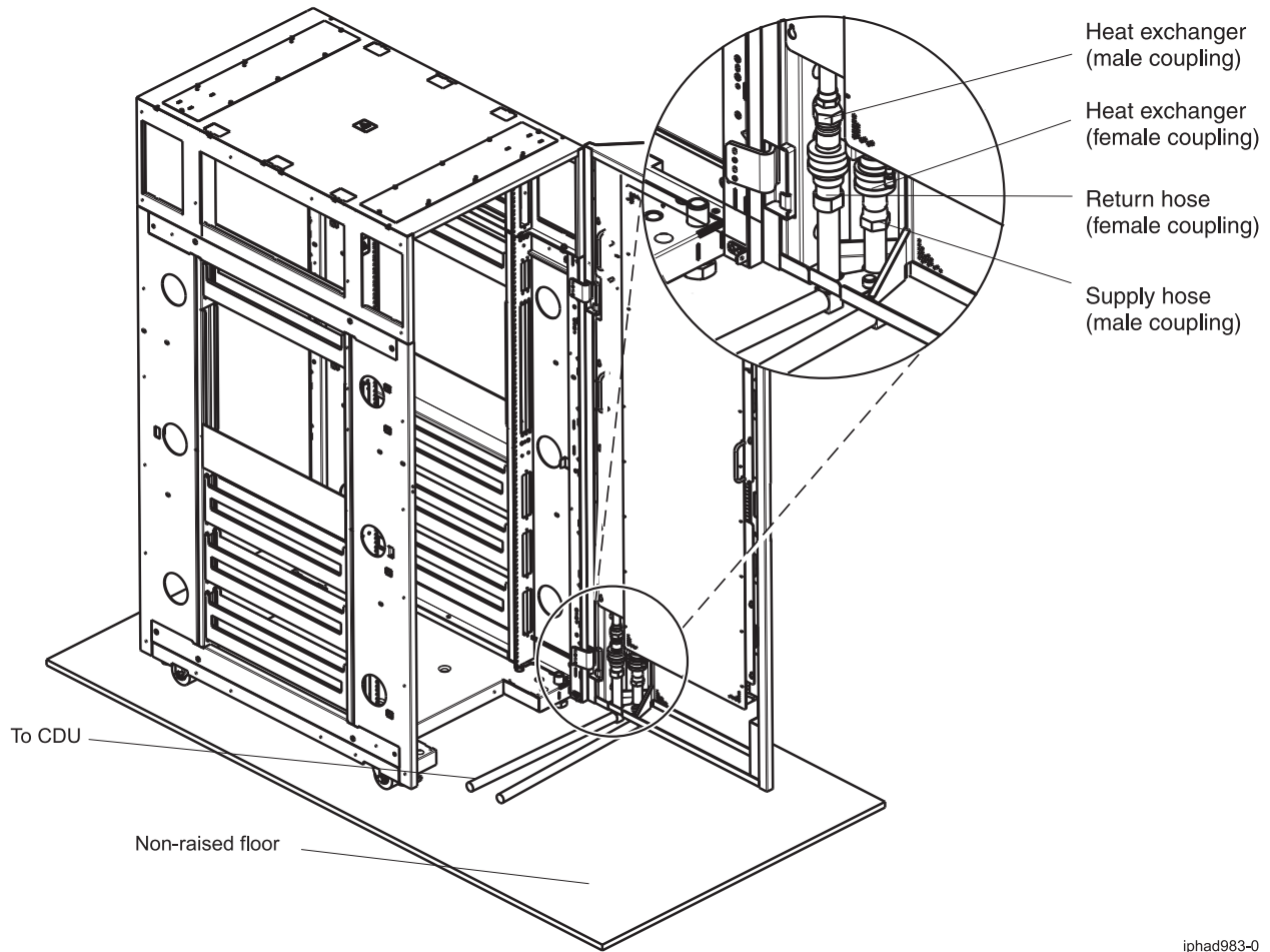
Figure 32. Non-raised floor hose requirements 24-inch EIA-rail rack
