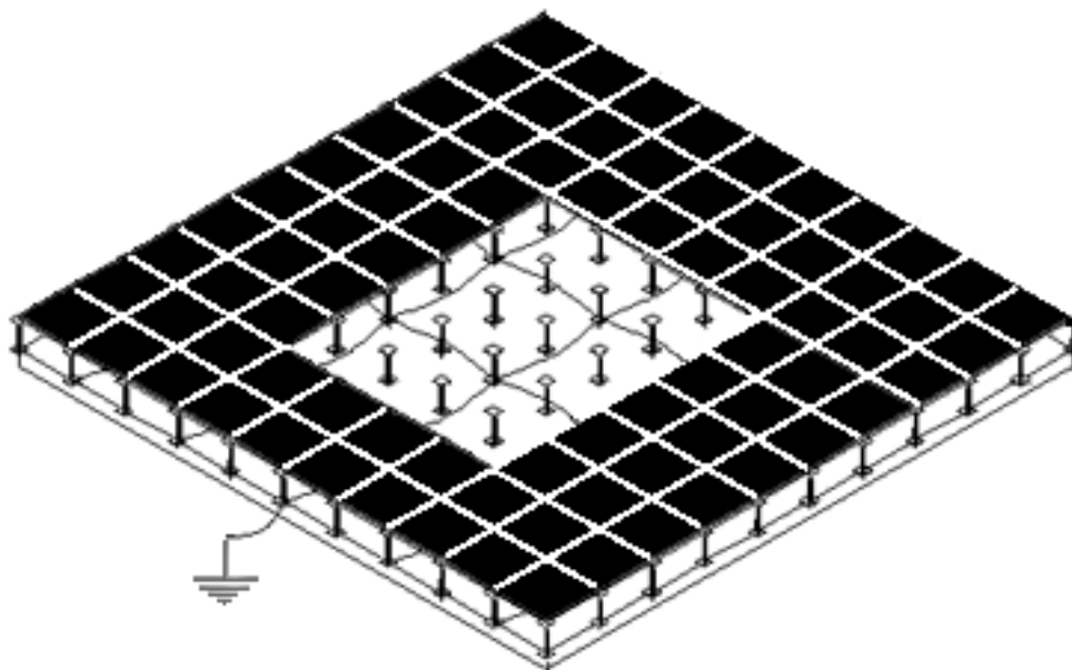
Figure 39. Signal reference ground
