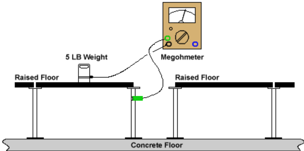
Figure 41. Typical test connection to measure floor conductivity
