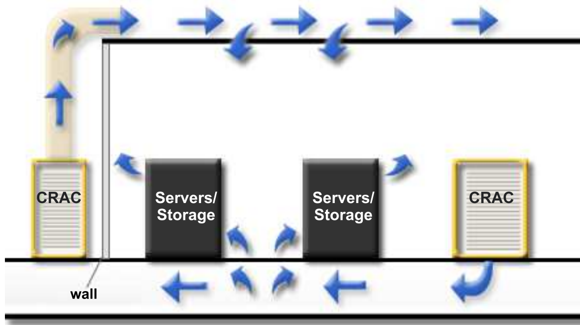
Figure 43. Combination overhead and underfloor air conditioning system
