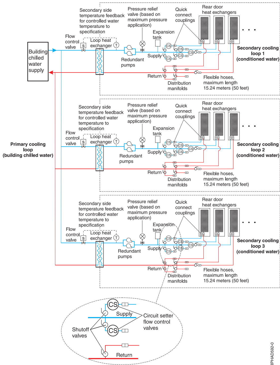
Figure 19. Primary and secondary cooling loops
