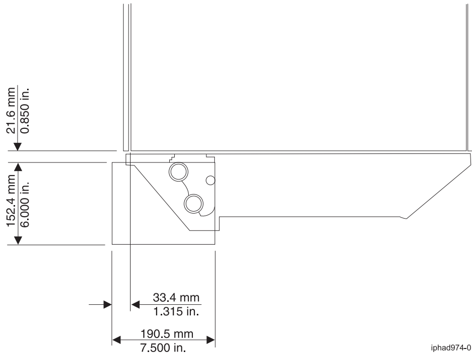
Figure 25. Raised floor hose management example 1; tile cut out definition and location for 19-inch EIA-rail racks
