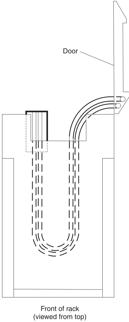
Figure 29. Raised floor and non-raised floor hose management example 2; loop under the 19-inch EIA-rail rack with door open
