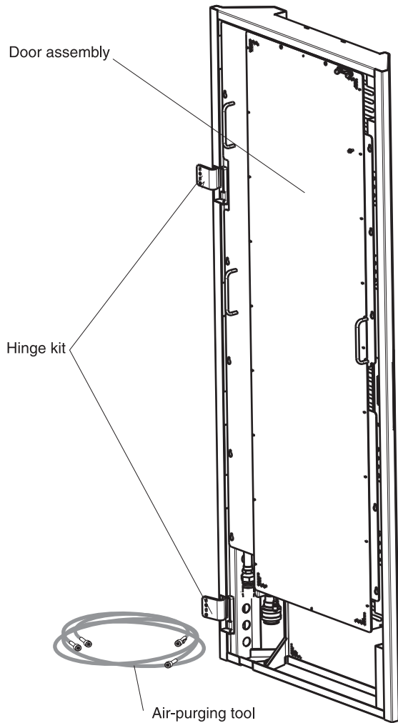
Figure 13. Components of the heat exchanger kit for 24-inch EIA-rail racks
