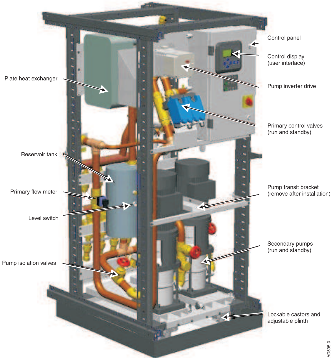
Figure 33. Cooling distribution unit
