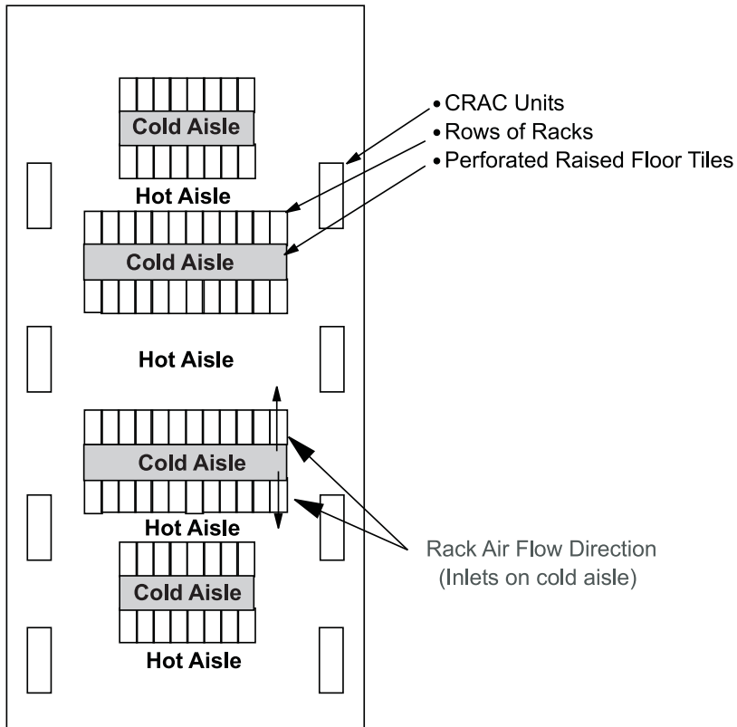
Figure 2. Hot aisle and cold aisle arrangement
