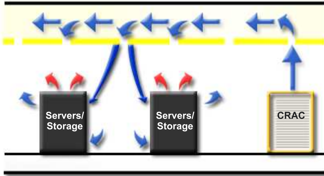
Figure 44. Overhead air distribution system
