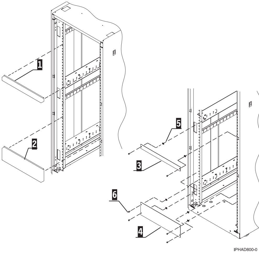
Figure 1. 1U and 3U filler panel figure and part numbers.
