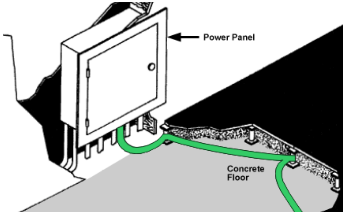
Figure 36. Transient grounding using the raised floor support structure
