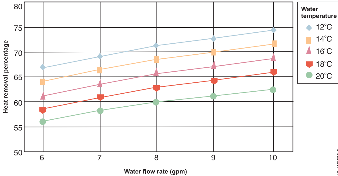
Figure 14. Typical performance of a rear door heat exchanger, 32 kW heat load. Percentage heat removal as function of water temperature and flow rate. (24°C rack inlet air, 32 kW rack load, 1530 cfm air through the rear door heat exchanger)
