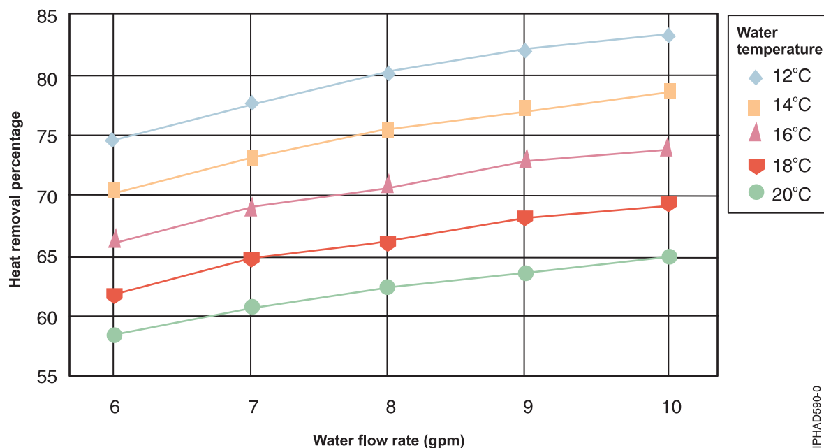
Figure 15. Typical performance of a rear door heat exchanger, 20 kW heat load. Percentage heat removal as function of water temperature and flow rate. (24°C rack inlet air, 20 kW rack load, 1530 cfm air through the rear door heat exchanger)
