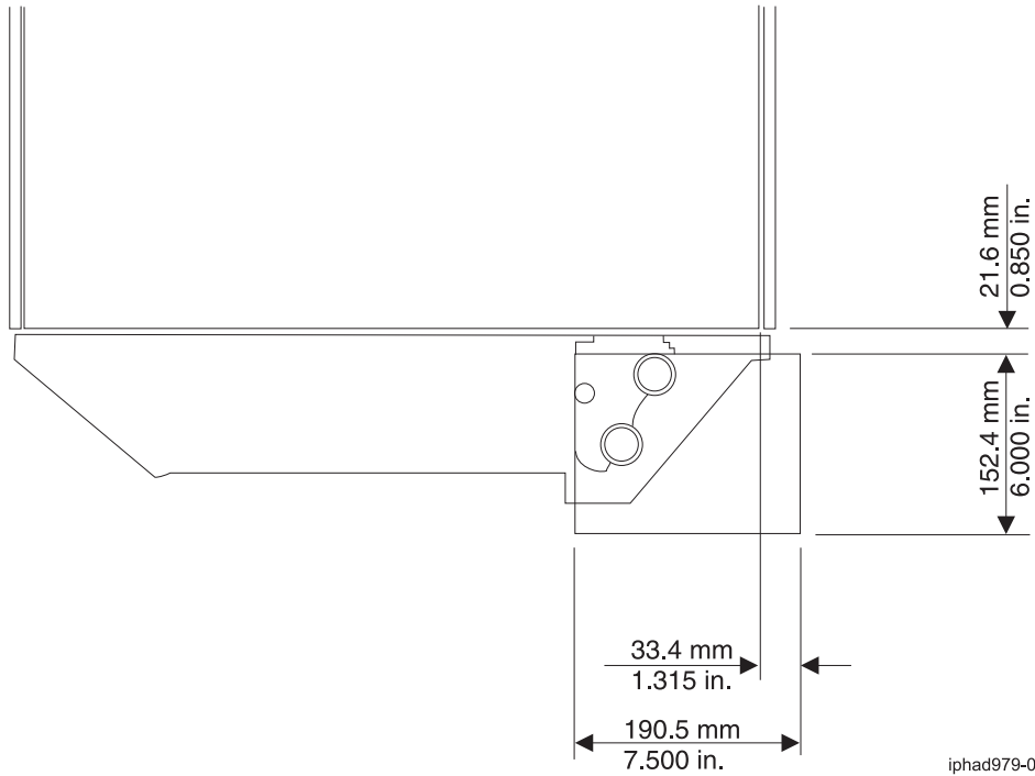
Figure 26. Raised floor hose management example 1; tile cut out definition and location for 24-inch EIA-rail racks
