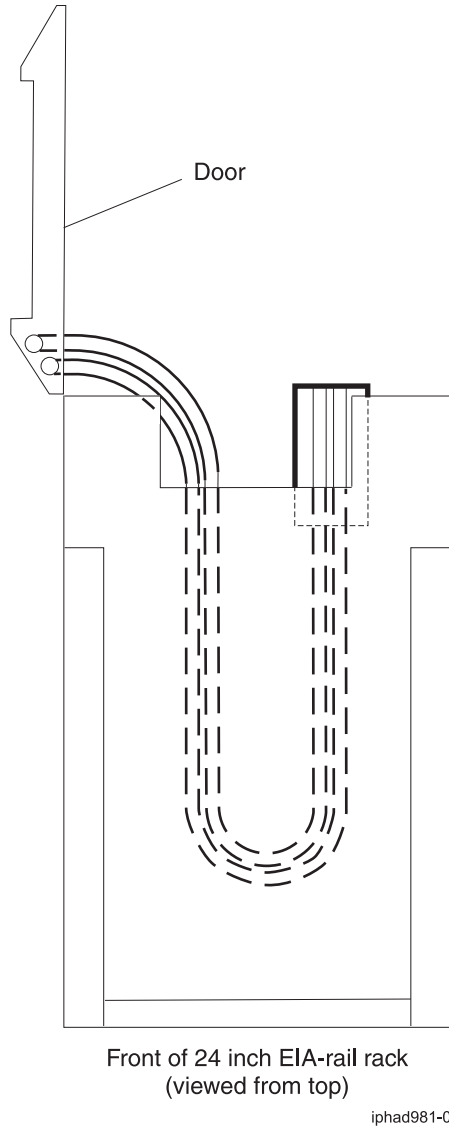
Figure 30. Raised floor and non-raised floor hose management example 2; loop under the 24-inch EIA-rail rack with door open
