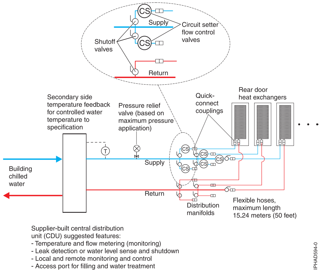
Figure 17. Coolant distribution using off-the-shelf supplier solutions
