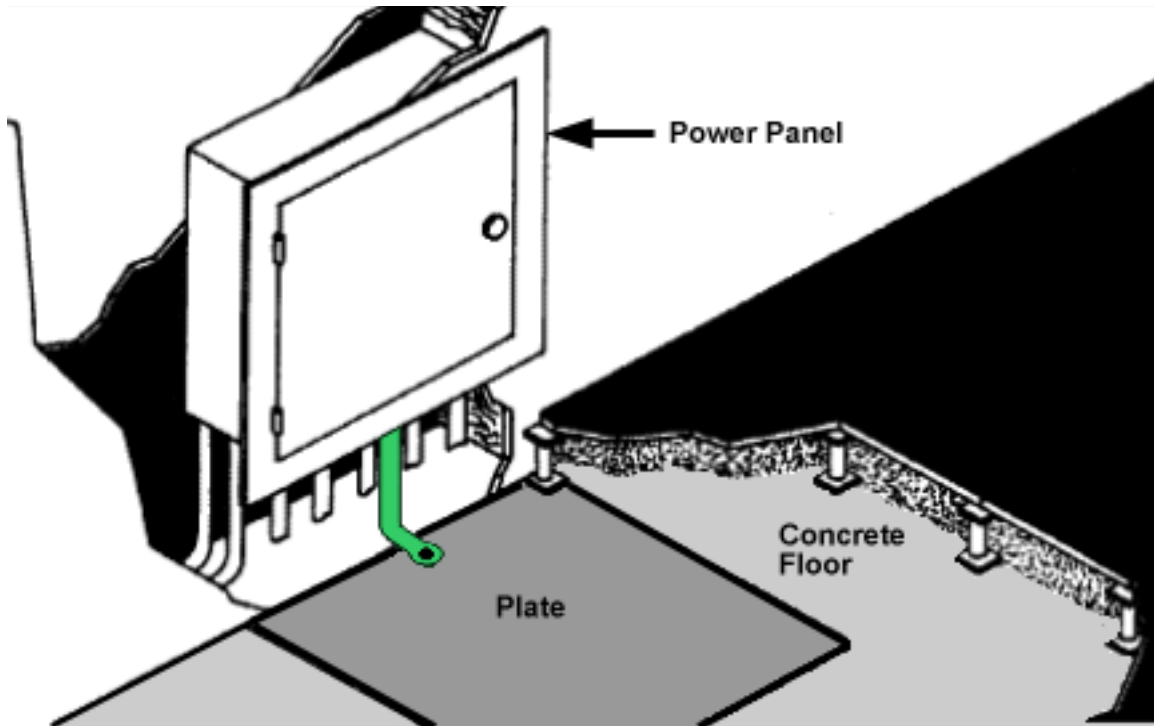
Figure 35. Transient grounding plate
