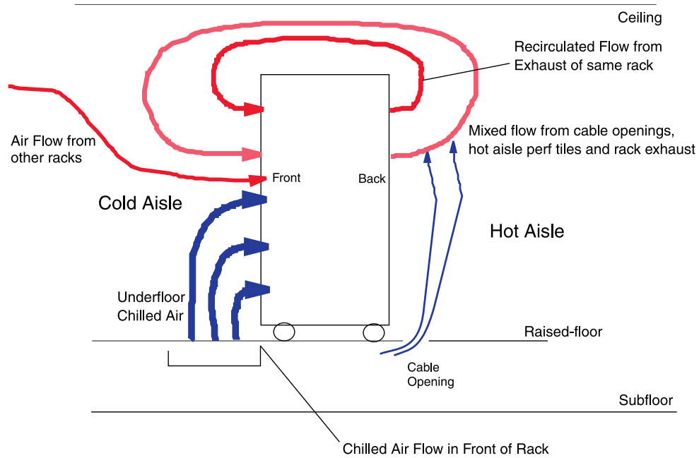
Figure 3. Possible rack airflow patterns
