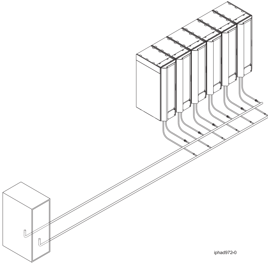
Figure 22. Typical extended manifold (located along aisles between racks)
