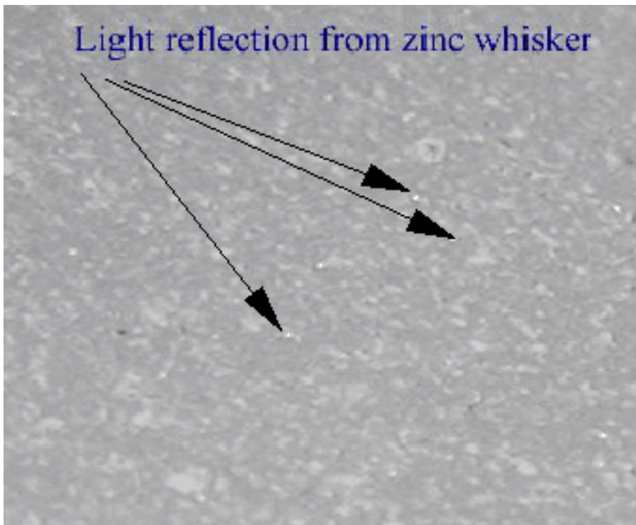
Figure 40. Light reflection from zinc whiskers
