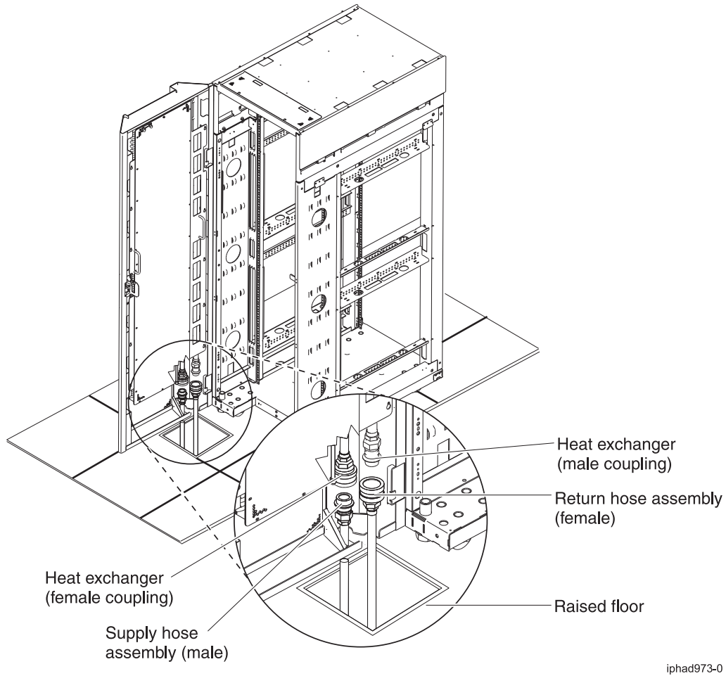
Figure 23. Raised floor hose management example 1; tile cut out size and position for 19-inch EIA-rail racks
