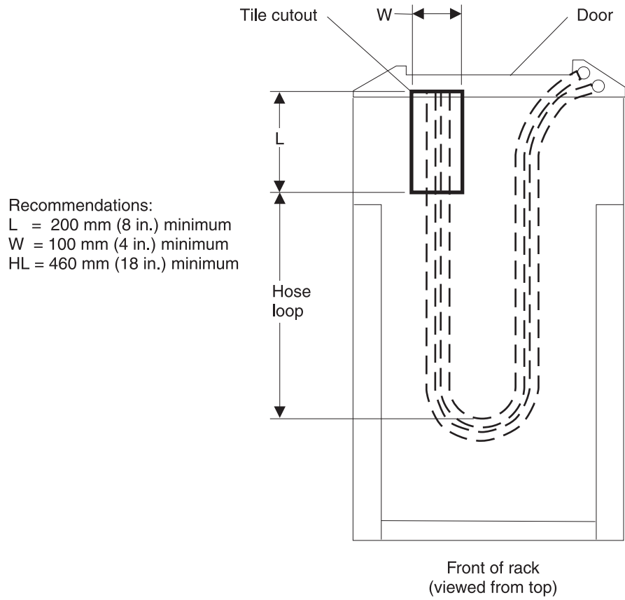
Figure 27. Raised floor and non-raised floor hose management example 2; loop under the 19-inch EIA-rail rack with door closed
