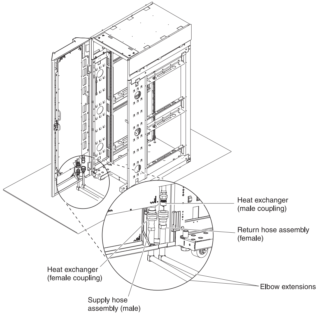
Figure 31. Non-raised floor hose requirements for 19-inch EIA-rail rack
