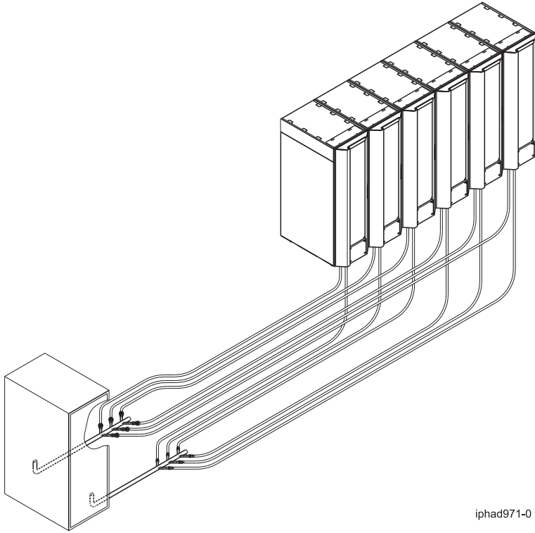
Figure 21. Typical central manifold (located at a central location for multiple water circuits)
