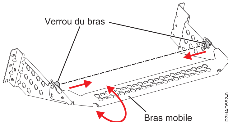
Figure 52. Passe-câbles
