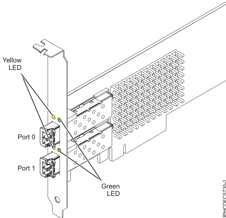
Figure 9. ENOB adapter
