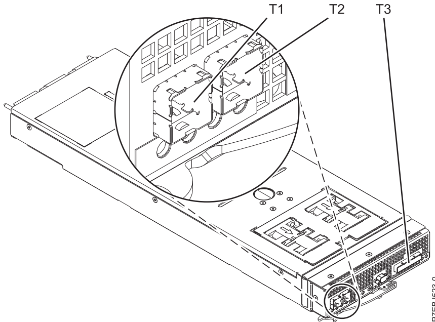
Figure 63. CCIN 57C3 PCIe2 3.1GB Cache RAID SAS Enclosure 6Gb x8
