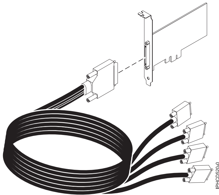
Figure 3. Cable
