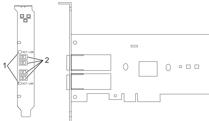
Figure 44. 2-Port Gigabit Ethernet-SX PCI Express Adapter
