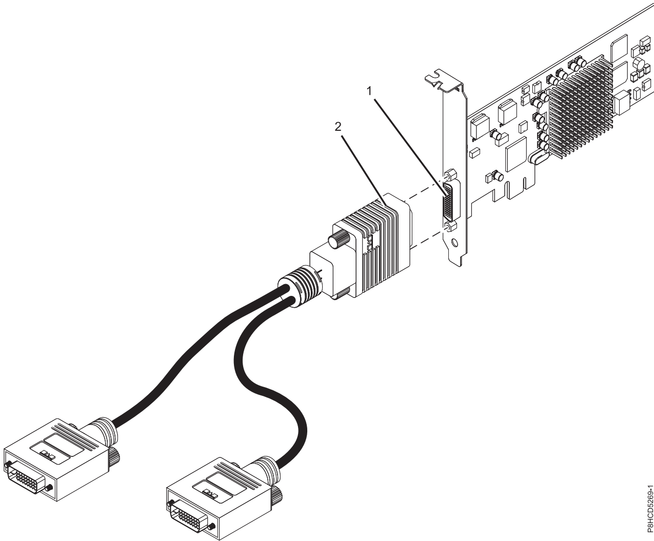
Figure 16. PCIe LP POWER GXT145 Graphics Accelerator adapter and converter cable
