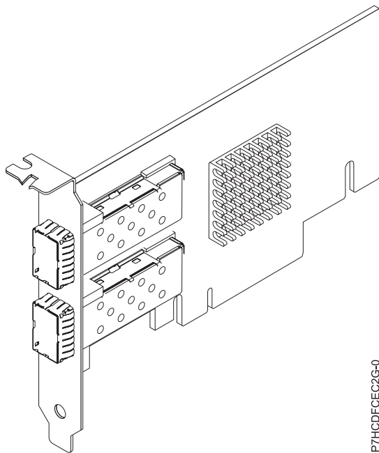
Figure 52. FC EC2G adapter
