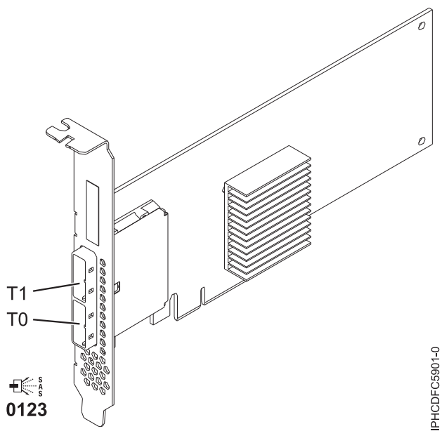
Figure 58. PCIe Dual - x4 SAS adapter
