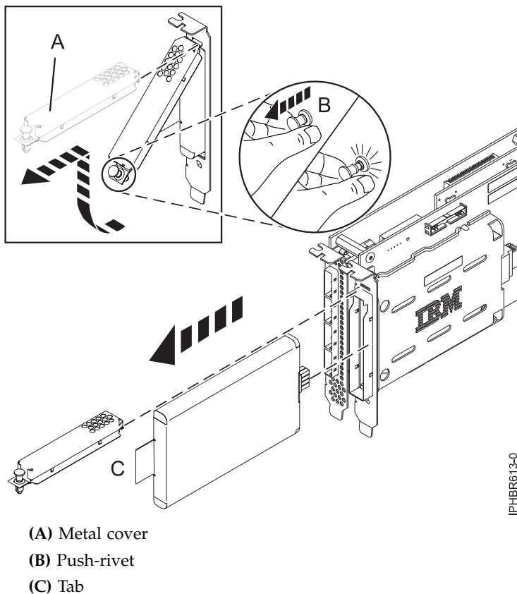
Figure 66. Replacing the 572F/575C cache battery
