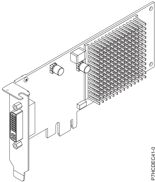
Figure 17. PCIe2 LP 3D Graphics Adapter
