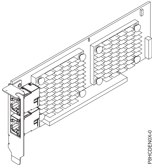
Figure 22. FC EN0X adapter
