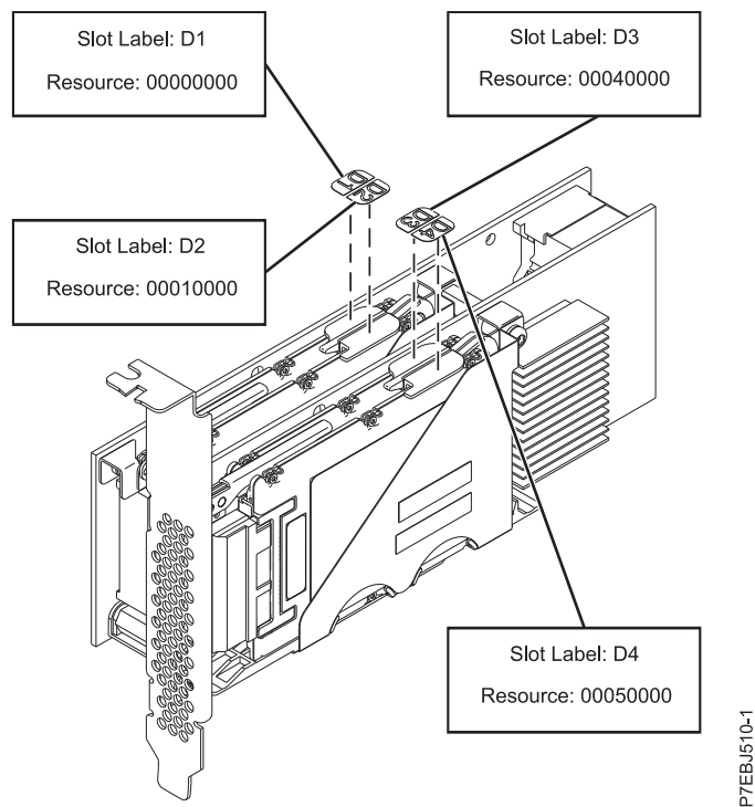
Figure 57. PCIe Dual - x4 3 Gb SAS RAID Adapter
