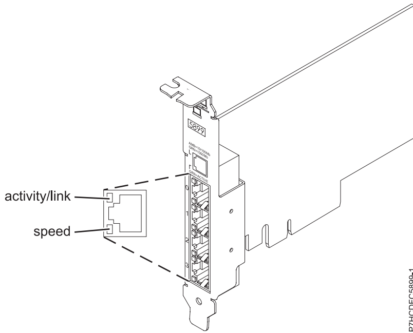
Figure 47. Adapter
