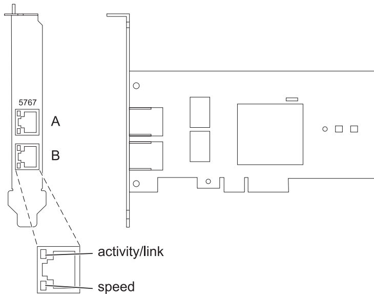
Figure 48. PCIe LP 2-Port 1GbE TX adapter
