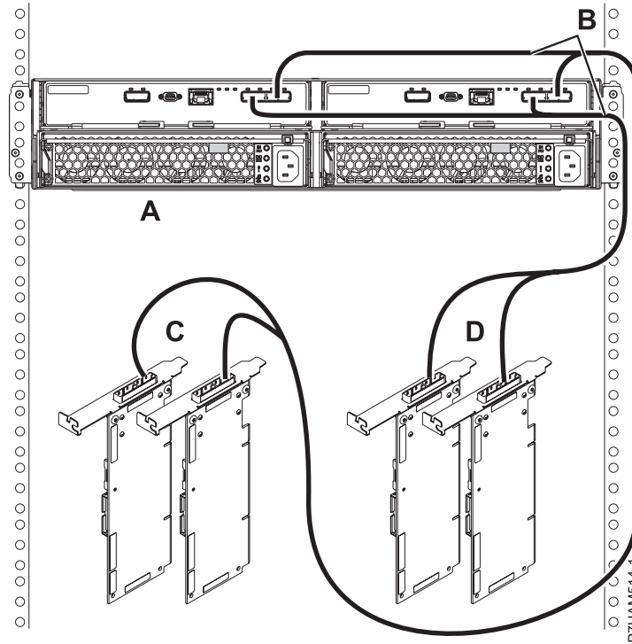
Figure 167. Mode 2 connection of a 5887 drawer by using X cables to two pairs of SAS adapters
