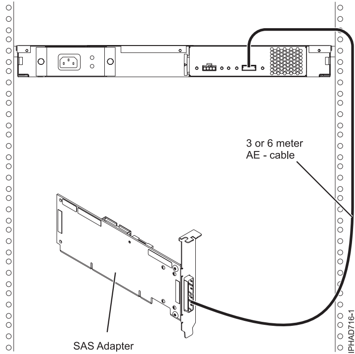
Figure 149. SAS adapter to a media expansion drawer
