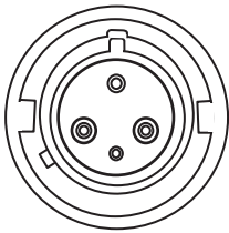
Figure 42. Receptacle type 60309 P+N+E
