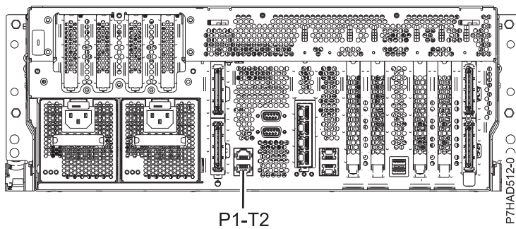
Figure 137. 8202-E4B, 8202-E4C, 8202-E4D, 8205-E6B, 8205-E6C, and 8205-E6D rear view with cable installation location
