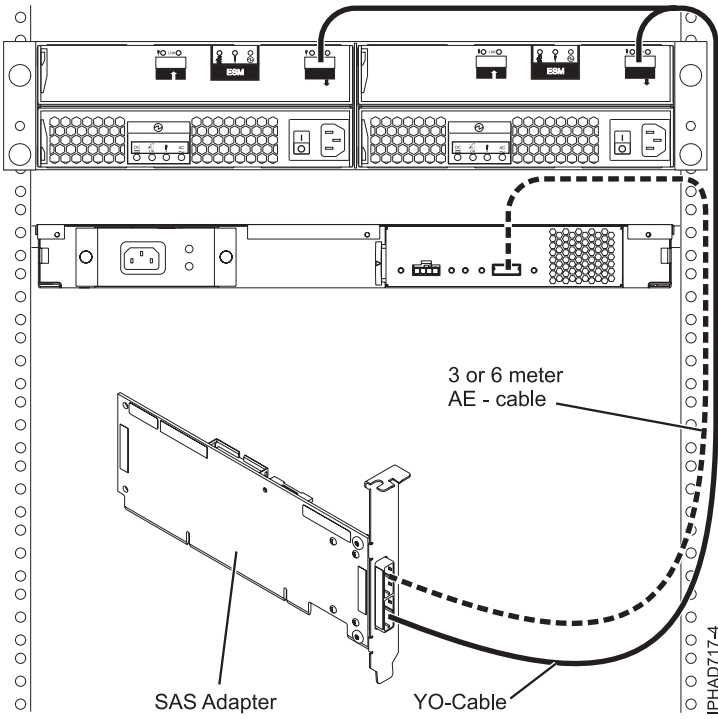
Figure 150. SAS adapter to both a disk expansion drawer and a media expansion drawer
