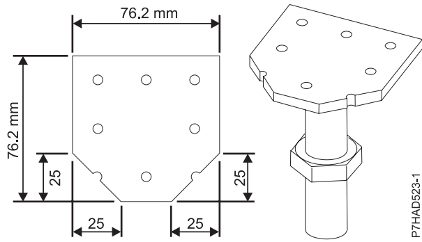
Figure 4. Cut pedestal dimensions
