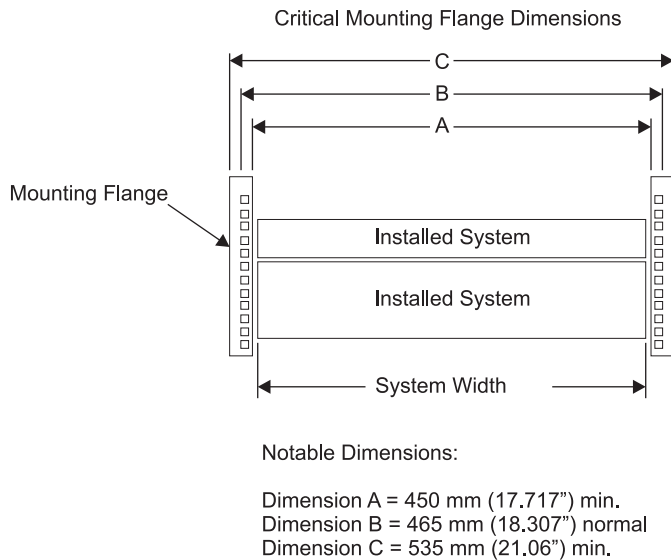
Figure 179. Critical mounting flange dimensions
