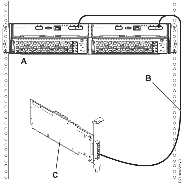
Figure 171. Mode 1 connection of a 5887 drawer by using a YO cable to a single SAS adapter
