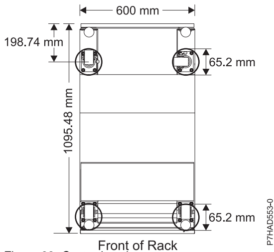
Figure 28. Caster locations
