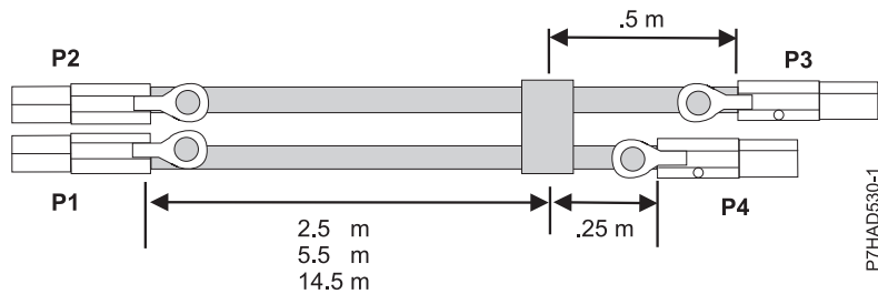
Figure 142. SAS external X cable assembly cable lengths
