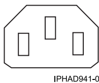
Figure 129. Plug type 26
