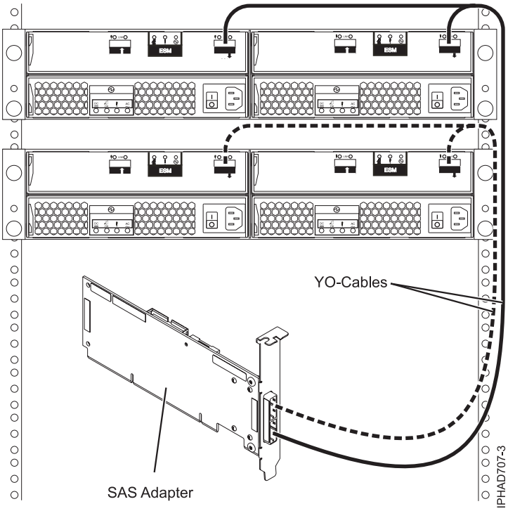
Figure 146. SAS adapter to two disk expansion drawers
