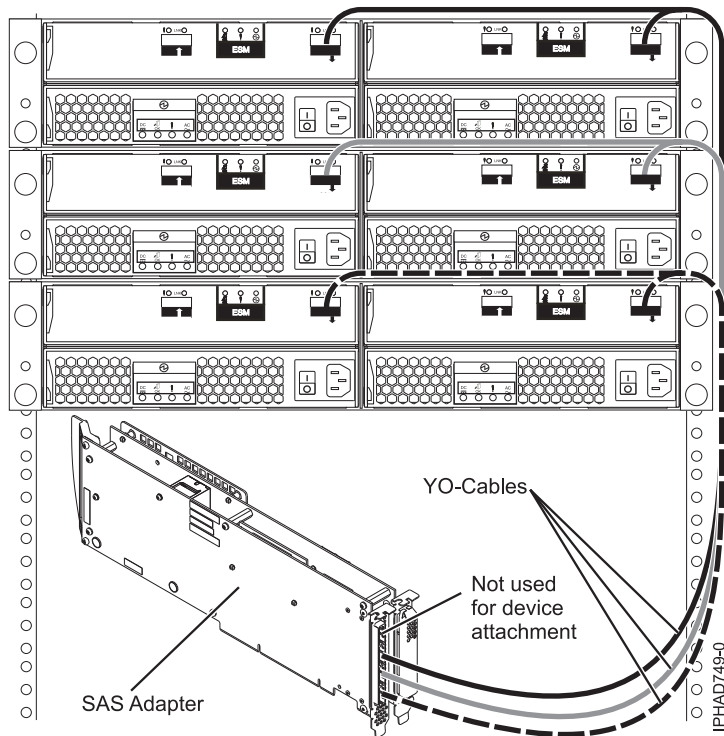
Figure 148. Tri-port SAS adapter to disk expansion drawers
