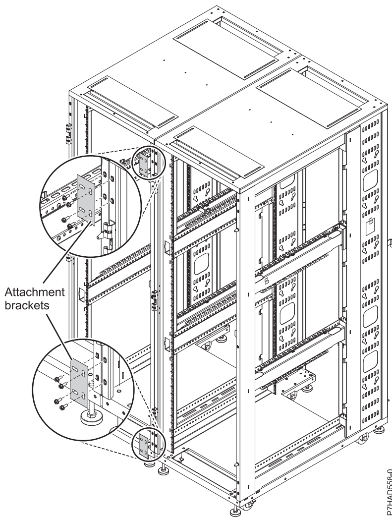
Figure 33. Attachment brackets
