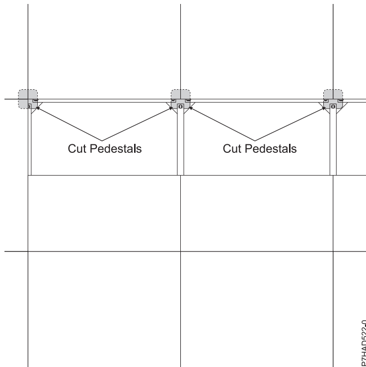
Figure 5. Cut pedestals
