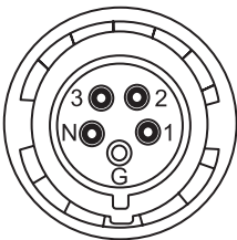
Figure 36. Plug pinout
