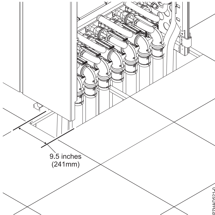
Figure 3. Floor cutout
