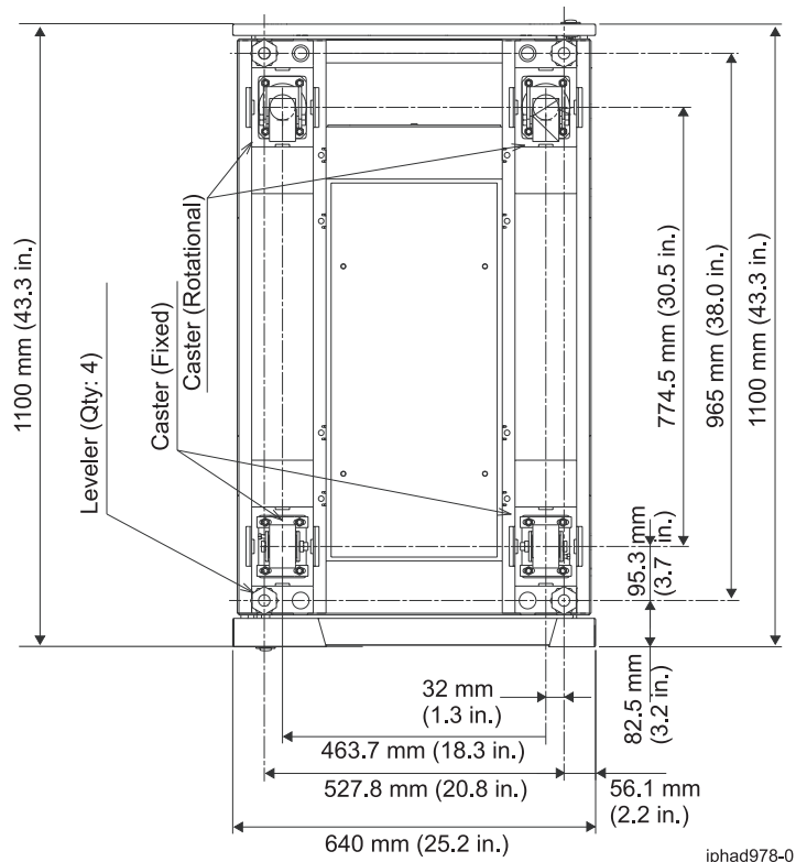
Figure 26. Caster and leveler locations
