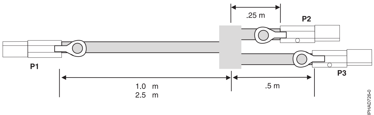
Figure 144. SAS external YI-cable assembly cable lengths
