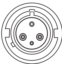
Figure 38. Receptacle type IEC 60309 P+N+E
