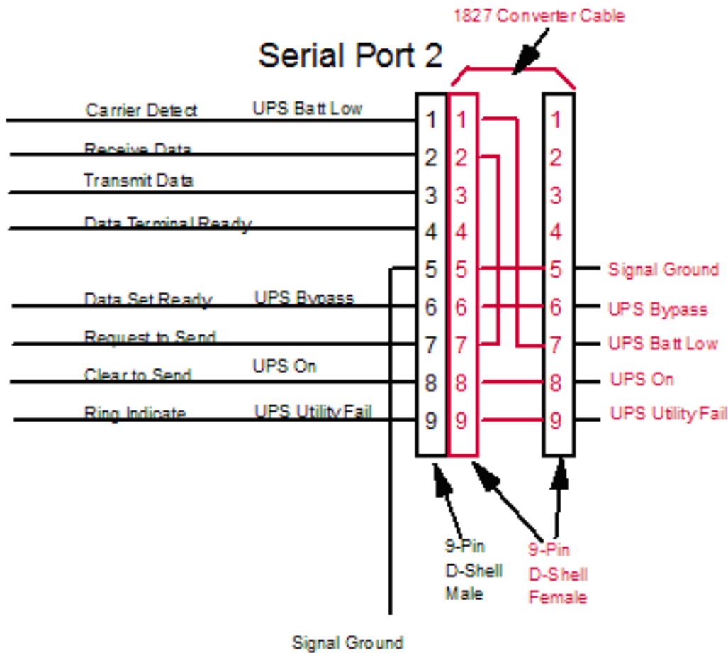
Figure 132. 1827 cable wiring
