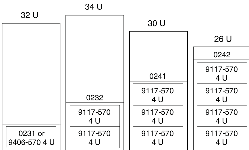
Figure 12. 570 in rack
