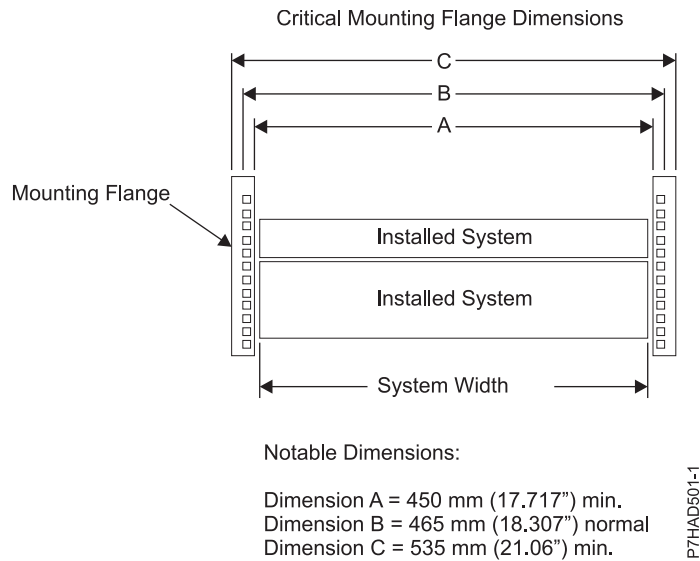
Figure 34. Critical mounting flange dimensions
