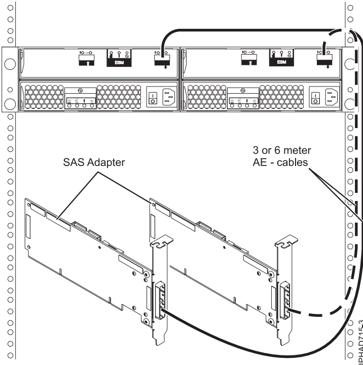
Figure 162. Two RAID SAS adapters to a disk expansion drawer in a multi-initiator HA JBOD configuration
