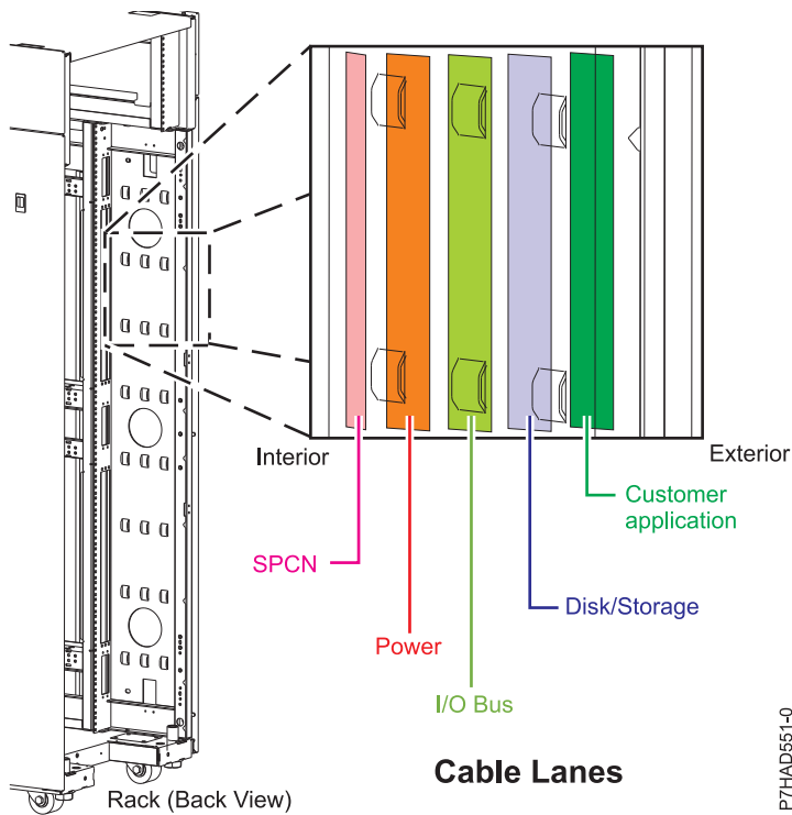
Figure 139. Cable management bridge lances
