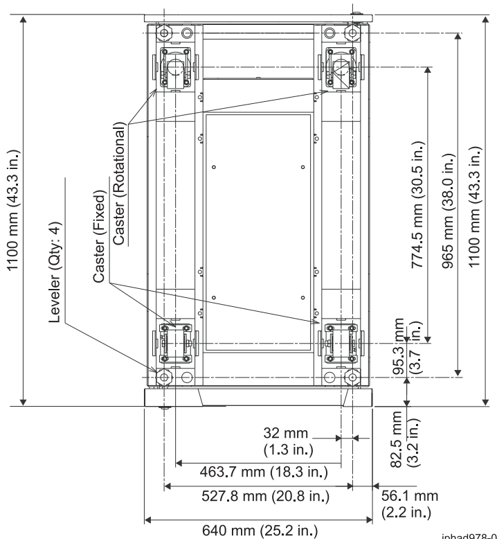
Figure 9. Caster and leveler locations
