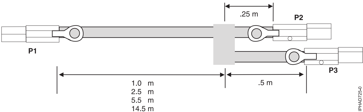
Figure 143. SAS external YO-cable assembly cable lengths
