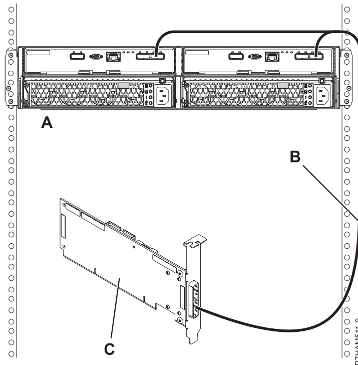
Figure 164. Mode 1 connection of a 5887 drawer by using a YO cable to a single SAS adapter
