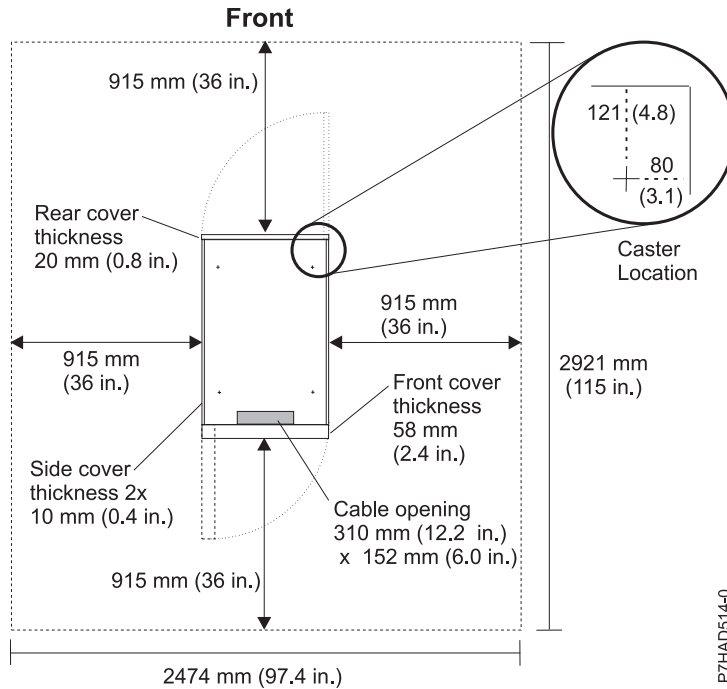
Figure 27. Service clearances and caster location for 7014-T00, 7014-T42, and 0553 racks
