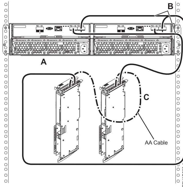
Figure 172. Mode 1 connection of a 5887 drawer by using YO cables to dual SAS adapters
