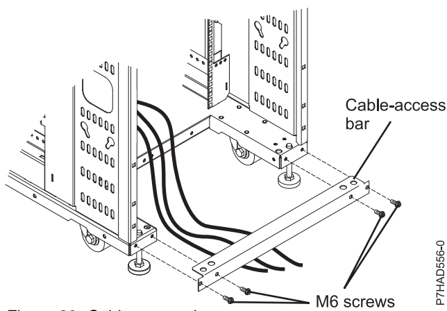
Figure 30. Cable access bar
