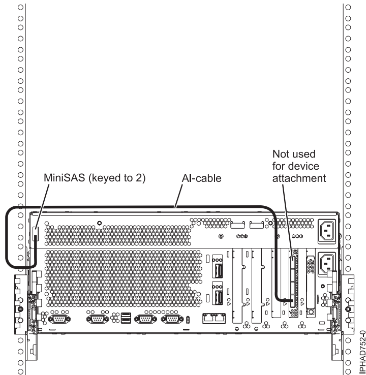
Figure 153. FC5904 or FC5908 adapter attached to disk expansion drawers
