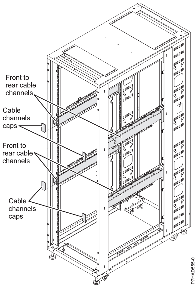
Figure 29. Cabling within the rack
