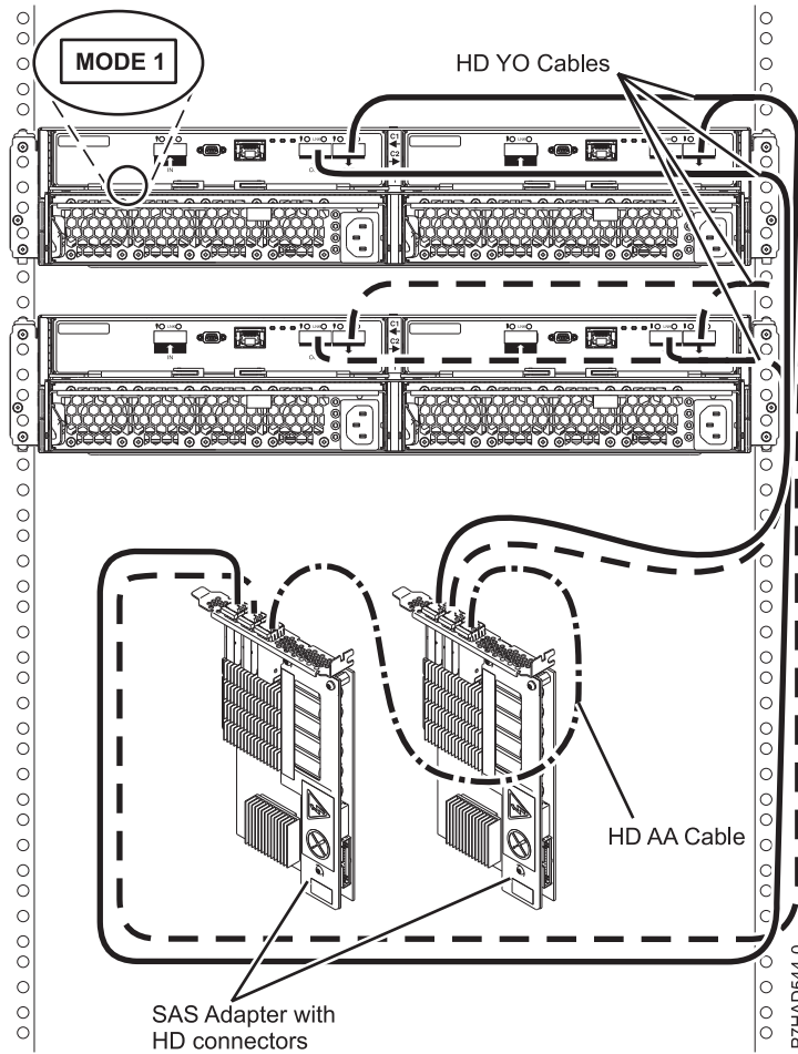
Figure 174. Mode 1 connection of two 5887 drawers by using HD connectors to two SAS adapters
