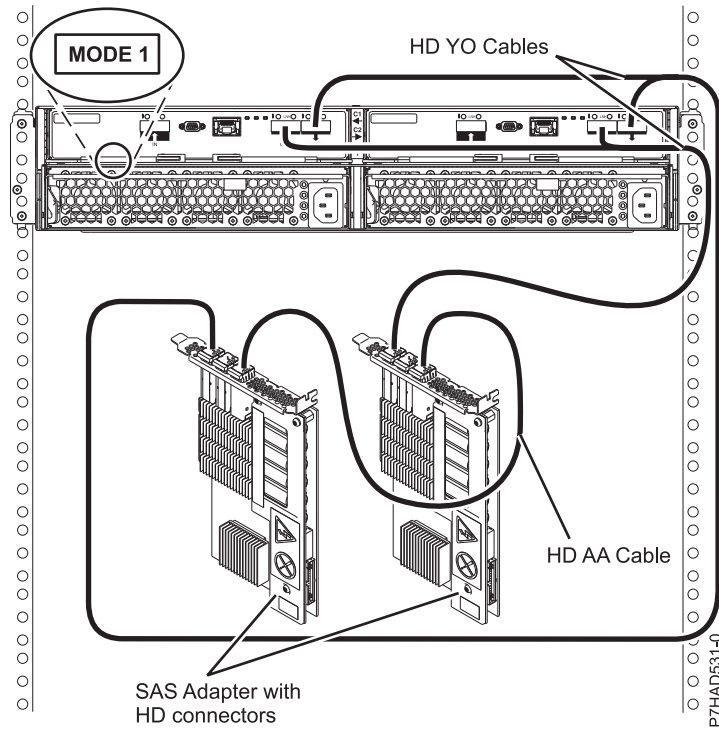
Figure 173. Mode 1 connection of a 5887 drawer to two SAS adapters with HD connectors
