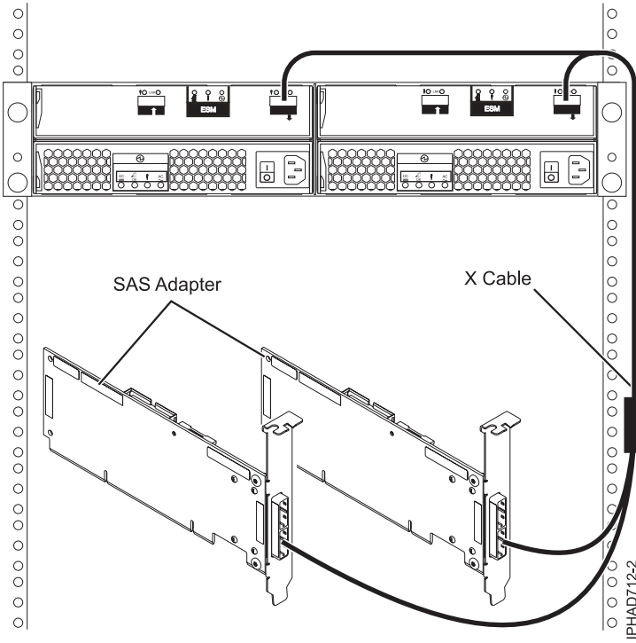
Figure 154. Two SAS RAID adapters to a disk expansion drawer in a multi-initiator HA RAID configuration
