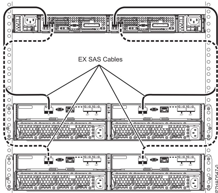
Figure 178. Connection of two 5887 drawers by using HD EX cables to one EDR1
