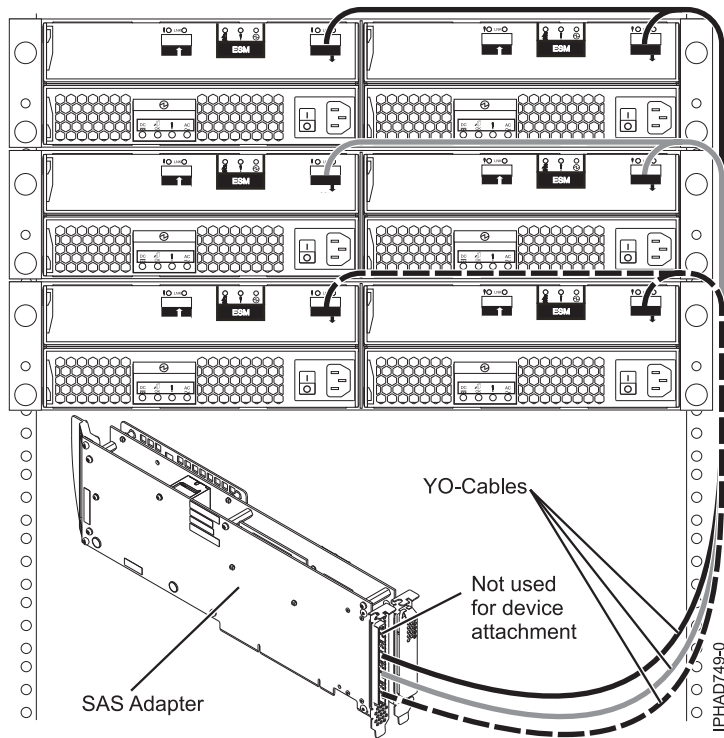
Figure 143. Tri-port SAS adapter to disk expansion drawers
