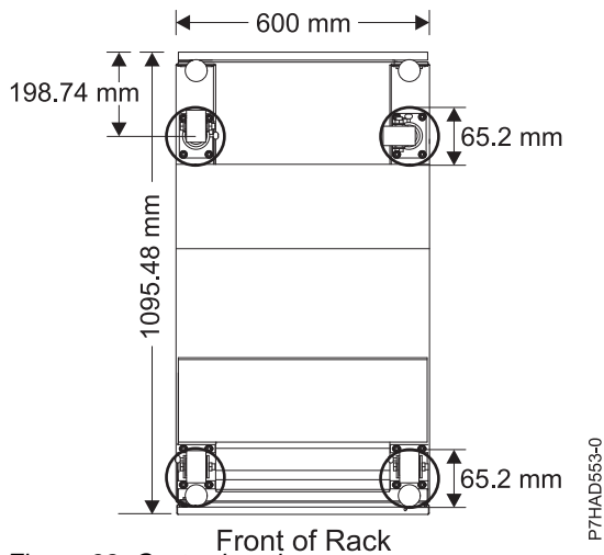
Figure 23. Caster locations
