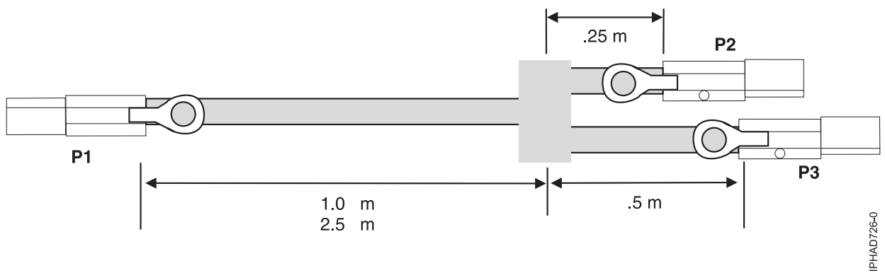
Figure 139. SAS external YI-cable assembly cable lengths
