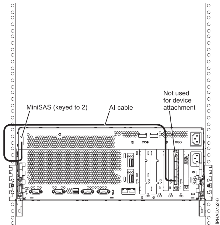
Figure 149. FC5904 or FC5908 adapter attached to disk expansion drawers
