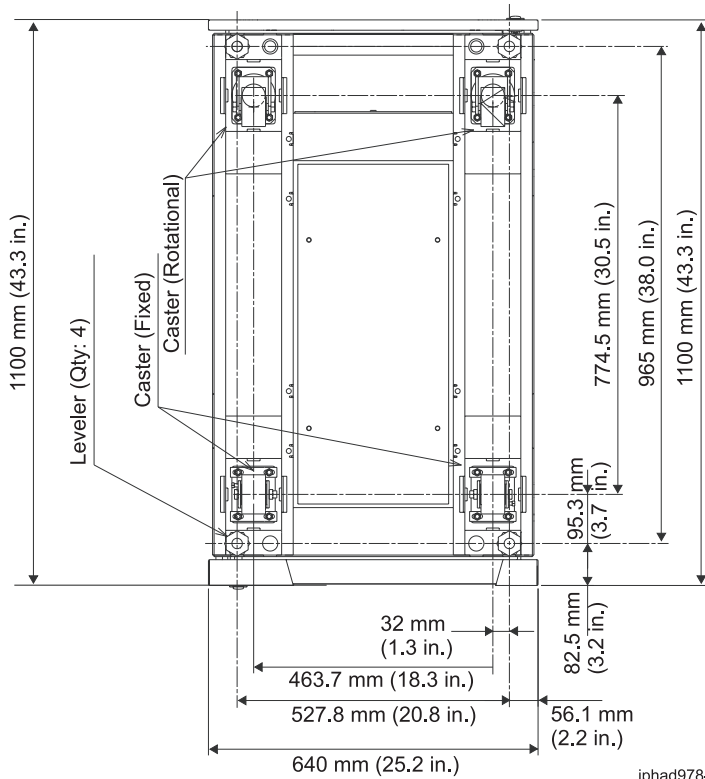
Figure 22. Caster and leveler locations
