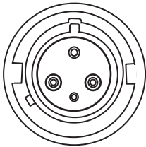
Figure 50. Receptacle type IEC 60309 2P+E
