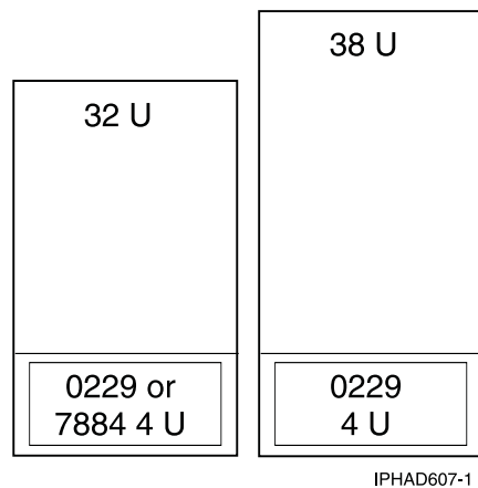
Figure 6. Feature code 7884: 9406-520 and 9111-520 in a rack
