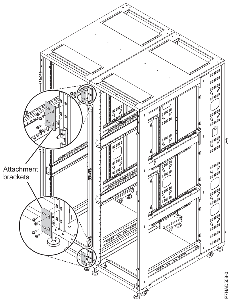
Figure 29. Attachment brackets
