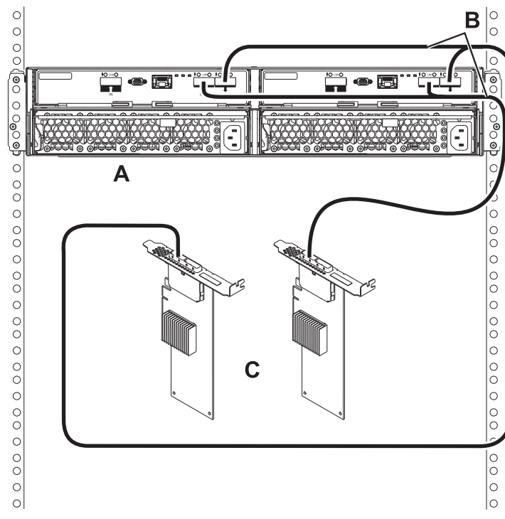
Figure 161. Mode 1 connection of a 5887 drawer by using YO cables to dual SAS adapters
