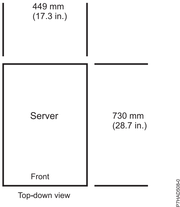
Figure 1. Model 8202-E4B, 8202-E4C, 8202-E4D, 8205-E6B, 8205-E6C, and 8205-E6D plan view (rack-mounted servers)
