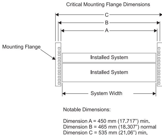
Figure 175. Critical mounting flange dimensions
