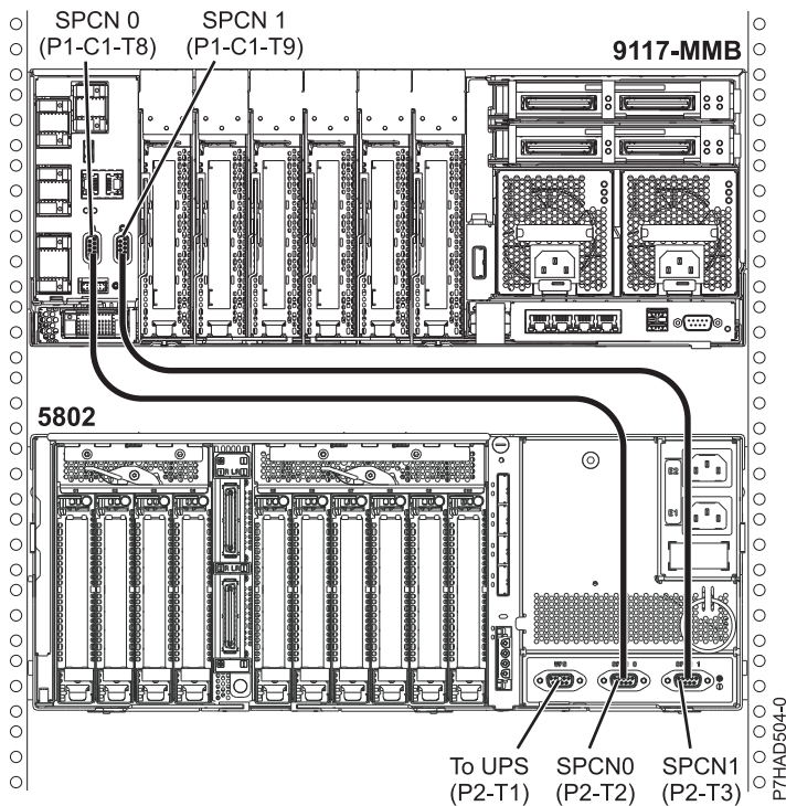
Figure 131. 8412-EAD, 9117-MMB, 9117-MMC, 9117-MMD, 9179-MHB, 9179-MHC, 9179-MHD, and 5208 or 5877 rear view cable installation location
