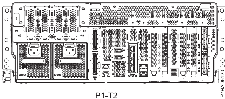
Figure 133. 8202-E4B, 8202-E4C, 8202-E4D, 8205-E6B, 8205-E6C, and 8205-E6D rear view with cable installation location
