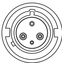
Figure 34. Receptacle type IEC 60309 P+N+E
