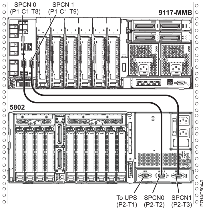
Figure 131. 8412-EAD, 9117-MMB, 9117-MMC, 9117-MMD, 9179-MHB, 9179-MHC, 9179-MHD, and 5208 or 5877 rear view cable installation location
