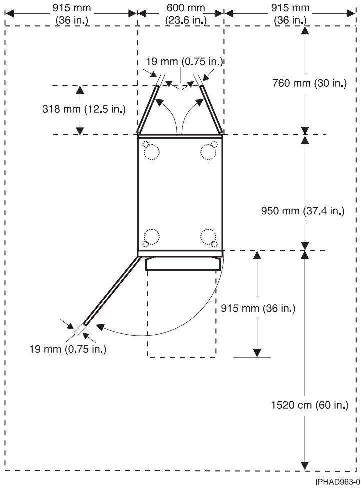
Figure 20. Model 0555 and 7014-S25 plan view
