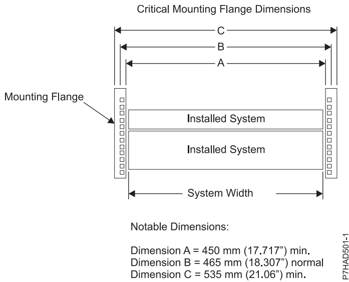
Figure 30. Critical mounting flange dimensions
