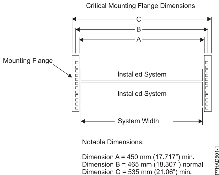
Figure 175. Critical mounting flange dimensions
