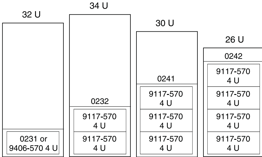
Figure 8. 570 in rack
