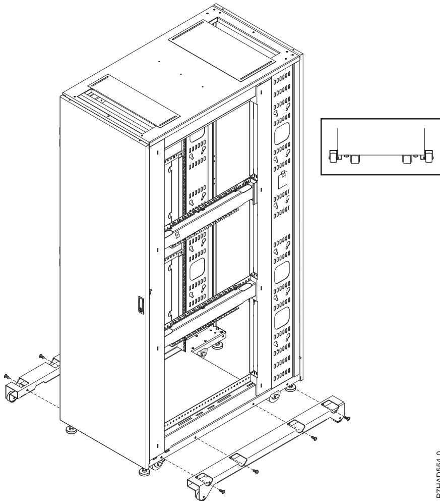
Figure 28. Outrigger locations
