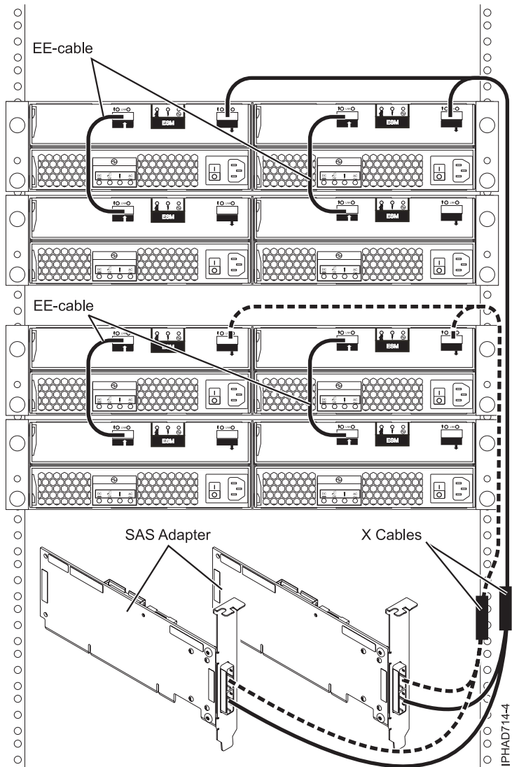
Figure 152. Two SAS RAID adapters to four disk expansion drawers in a multi-initiator HA RAID configuration
