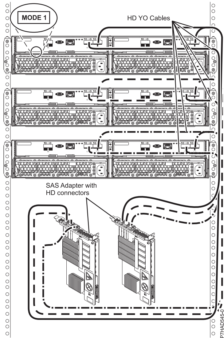
Figure 171. Mode 1 connection of three 5887 drawers to two SAS adapters with HD connectors
