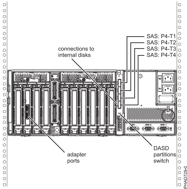
Figure 159. Two RAID SAS adapters to a disk expansion drawer in a multi-initiator HA JBOD configuration
