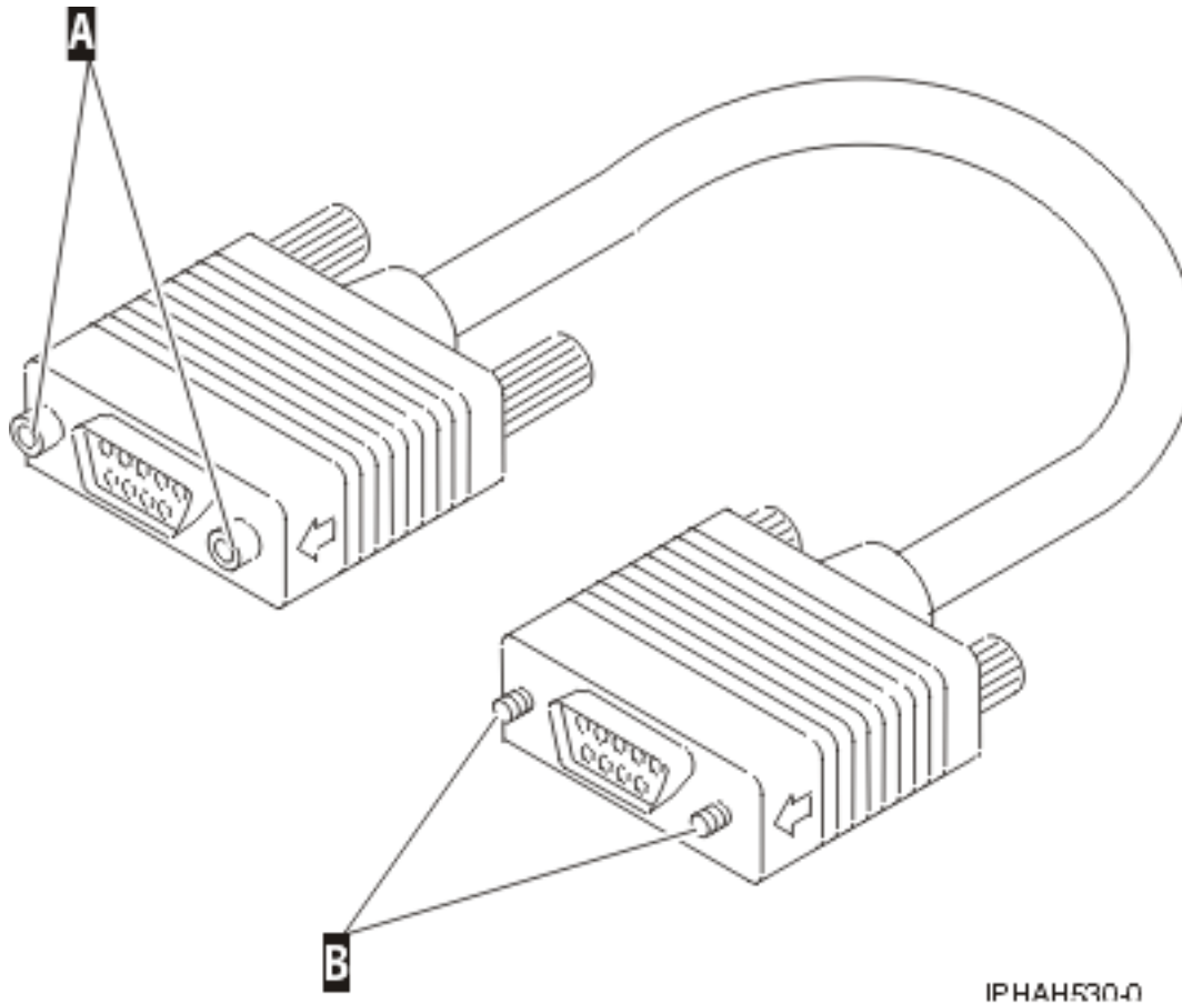
Figure 127. Uninterruptible power supply connector for the uninterruptible power supply communications cable
