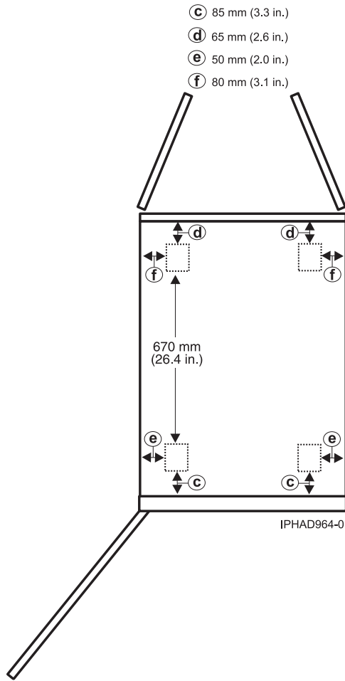
Figure 21. Model 0555 and 7014-S25 caster locations
