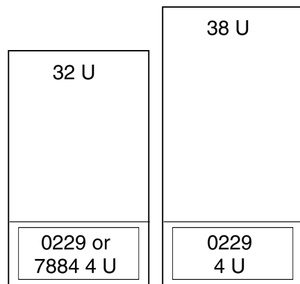
Figure 6. Feature code 7884: 9406-520 and 9111-520 in a rack
