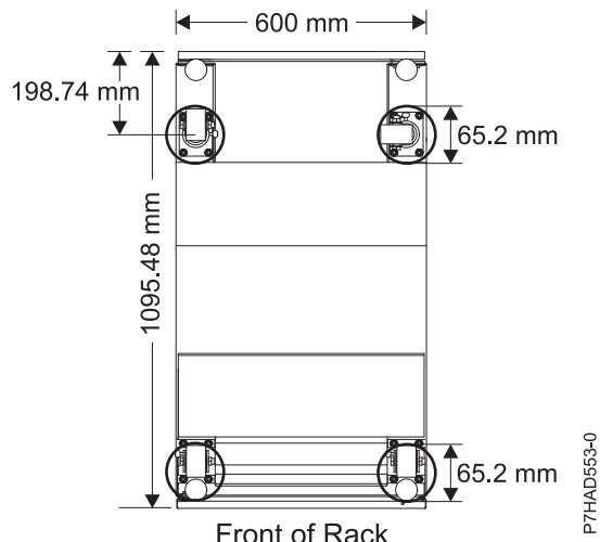
Figure 24. Caster locations
