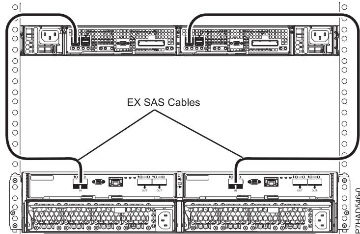
Figure 173. Connection of one 5887 drawer by using HD EX cables to one EDR1
