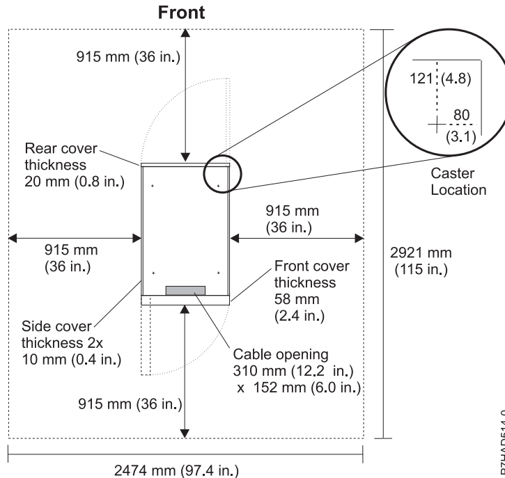
Figure 23. Service clearances and caster location for 7014-T00, 7014-T42, and 0553 racks
