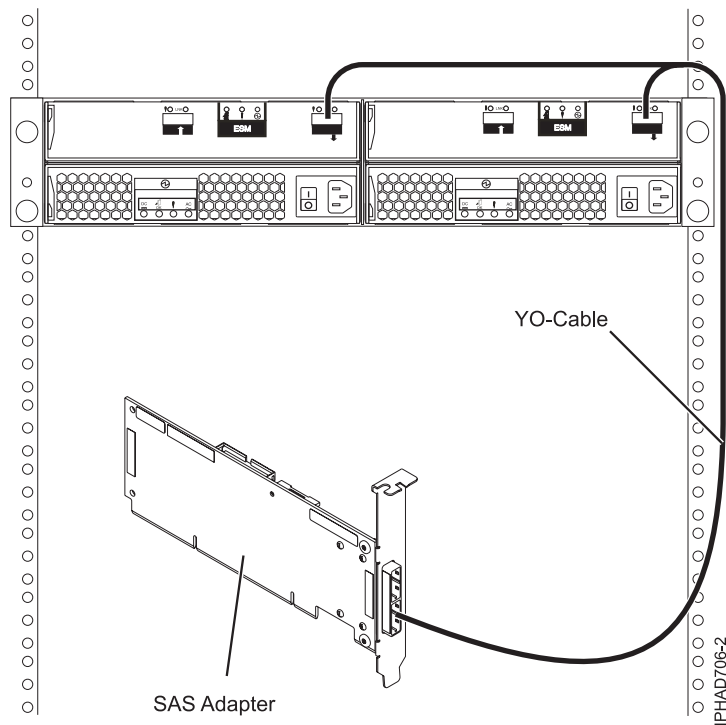
Figure 141. SAS adapter to a disk expansion drawer
