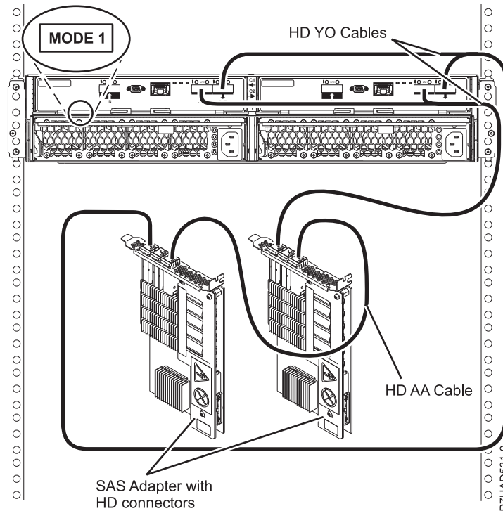
Figure 169. Mode 1 connection of a 5887 drawer to two SAS adapters with HD connectors
