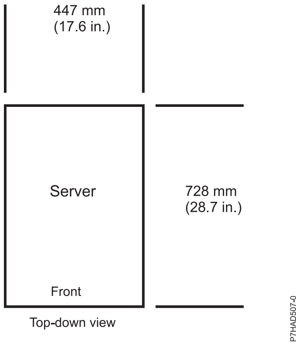
Figure 1. Model 8231-E2B, 8231-E1C, 8231-E1D, 8231-E2C, 8231-E2D, and 8268-E1D plan view (rack-mounted server)
