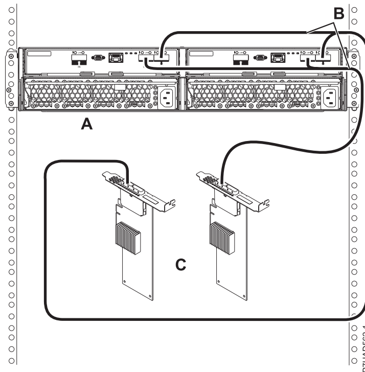
Figure 161. Mode 1 connection of a 5887 drawer by using YO cables to dual SAS adapters
