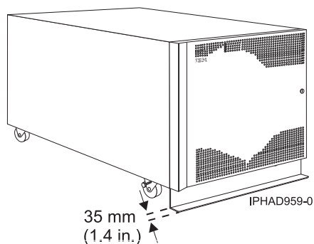
Figure 16. Model 0554 and 7014-S11 with stabilizer bar
