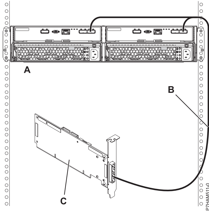
Figure 167. Mode 1 connection of a 5887 drawer by using a YO cable to a single SAS adapter
