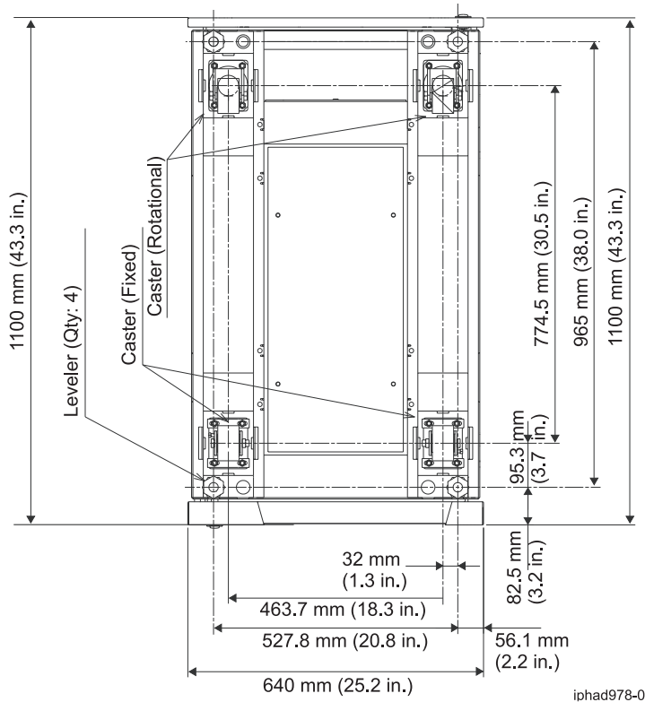
Figure 5. Caster and leveler locations
