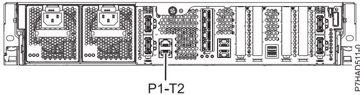
Figure 132. 8231-E2B, 8231-E1C, 8231-E1D, 8231-E2C, 8231-E2D, and 8268-E1D rear view with cable installation location
