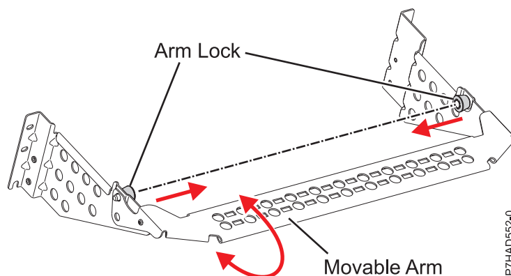
Figure 137. Cable management bracket
