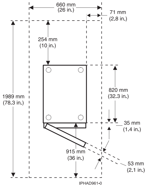
Figure 17. Model 0554 and 7014-S11 plan view
