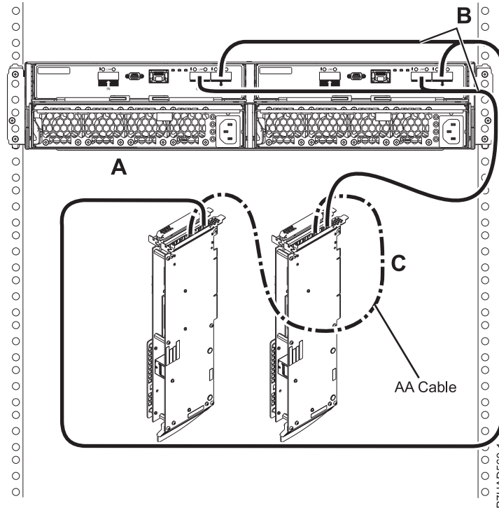
Figure 168. Mode 1 connection of a 5887 drawer by using YO cables to dual SAS adapters
