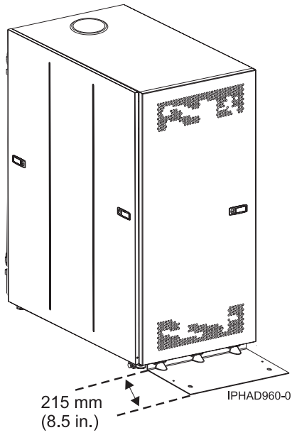
Figure 19. Model 0555 and 7014-S25 with stabilizer foot
