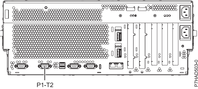
Figure 130. 8233-E8B and 8236-E8C rear view with cable installation location
