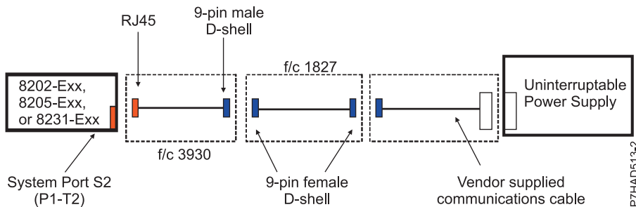
Figure 134. Uninterruptible power supply wiring for the 8202-E4B, 8202-E4C, 8205-E6B, 8205-E6C, 8231-E2B, 8231-E1C, 8231-E1D, 8231-E2C, 8231-E2D, and 8268-E1D
