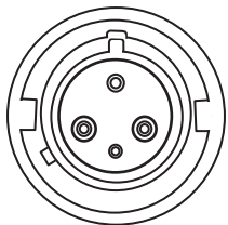
Figure 109. Receptacle type IEC 60309 2P+E
