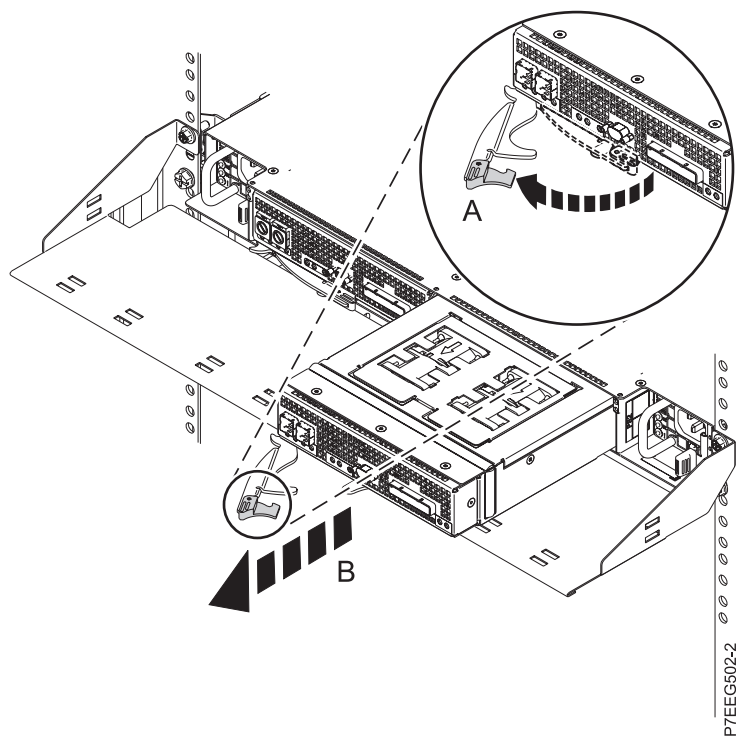
Figure 20. Removing an ERM assembly from the enclosure
