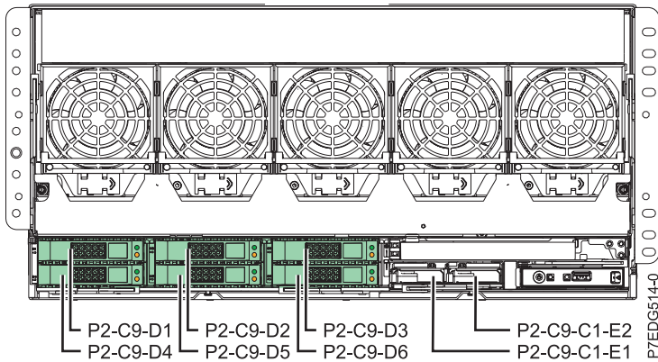
Figure 6. Disk bays controlled by both embedded SAS adapters that have dual storage IOA with internal and external drives
