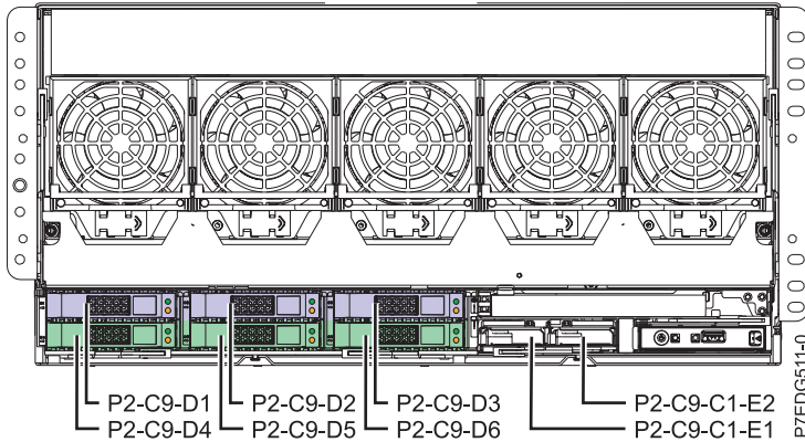
Figure 2. Disk bays controlled by each embedded SAS adapter in a two-way split backplane
