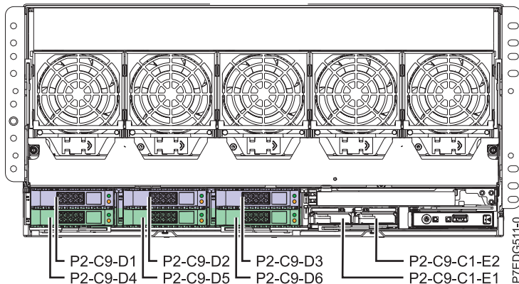
Figure 8. Disk bays controlled by each embedded SAS adapter in a two-way split backplane
