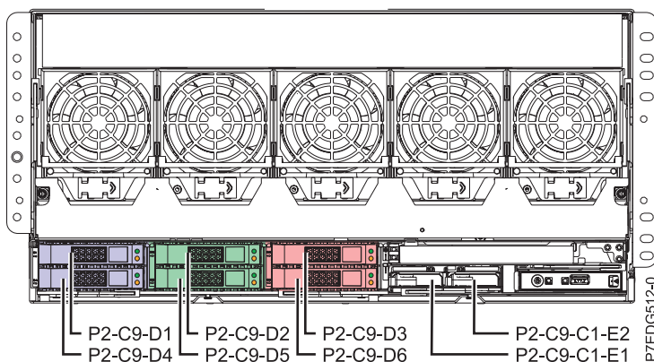
Figure 9. Disk bays controlled by adapters in a three-way split backplane
