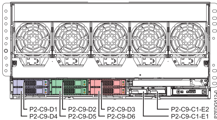
Figure 3. Disk bays controlled by each embedded SAS adapter in a three-way split backplane
