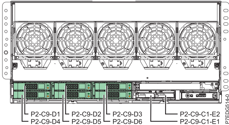
Figure 11. Disk bays controlled by both embedded SAS adapters that have dual storage IOA with internal drives
