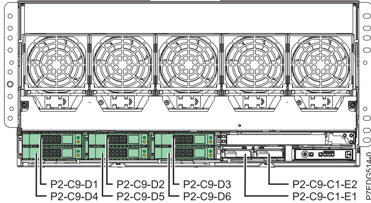
Figure 5. Disk bays controlled by both embedded SAS adapters that have dual storage IOA with internal drives
