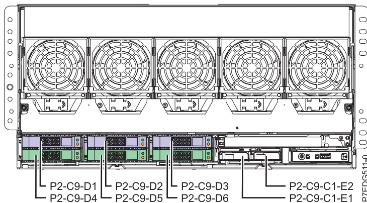
Figure 10. Disk bays controlled by each embedded SAS adapter in a two-way split backplane
