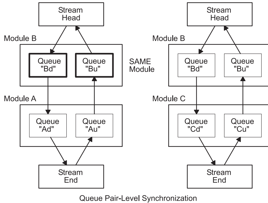
Figure 33. Queue Pair-Level Synchronization
