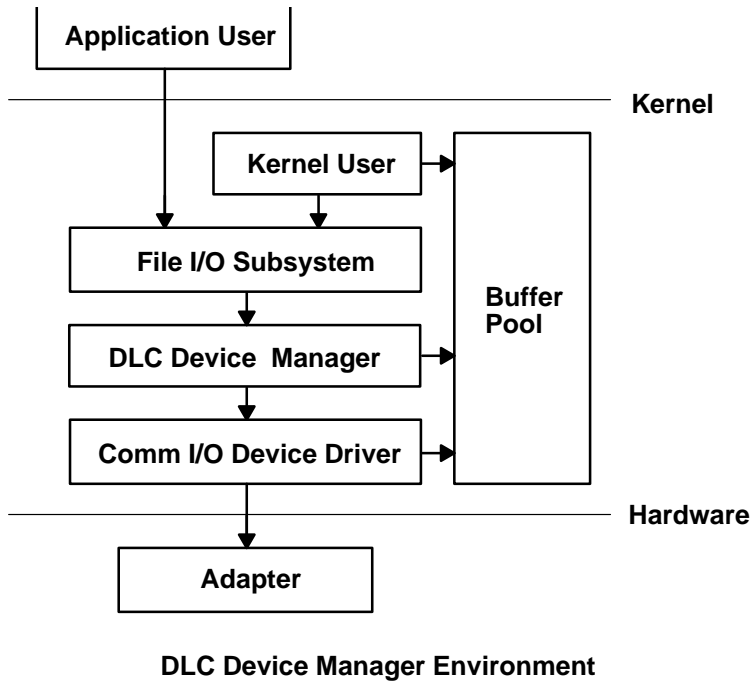
Figure 1. DLC Device Manager Environment
