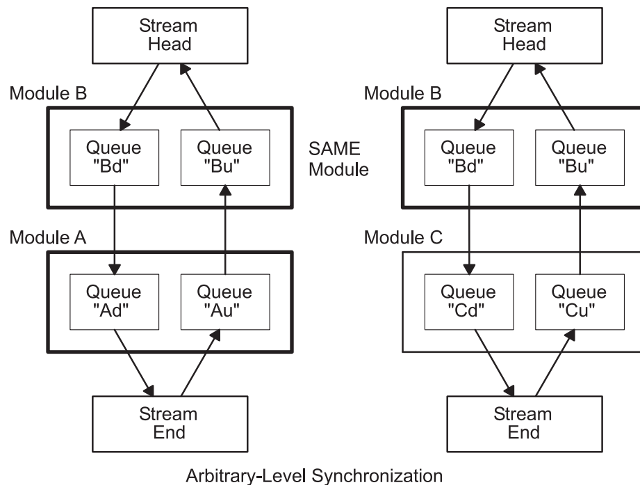
Figure 35. Arbitrary-Level Synchronization. This diagram shows two streams, with two modules each, where the first module in each stream is an instance of the same module (Module B). Each instance of Module B in each of the two streams is protected. Module A, the other module in the first stream, is also protected by the arbitrary-level synchronization.
