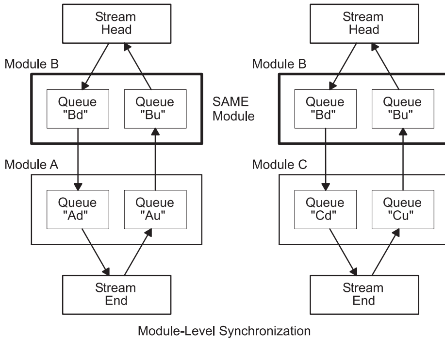
Figure 34. Module-Level Synchronization
