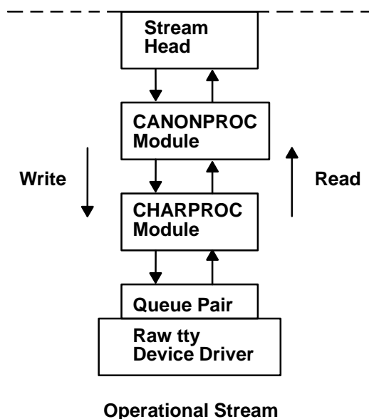
Figure 44. Operational Stream
