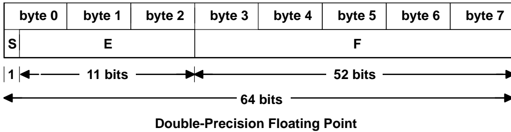
Figure 13. Double-Precision Floating-Point
