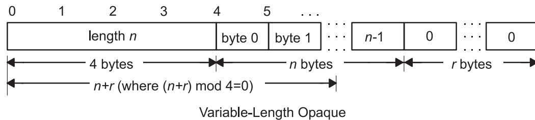
Figure 15. Variable-Length Opaque
