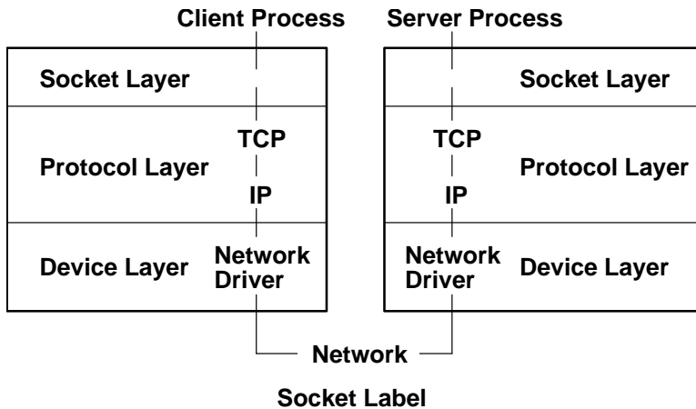
Figure 26. Socket Label
