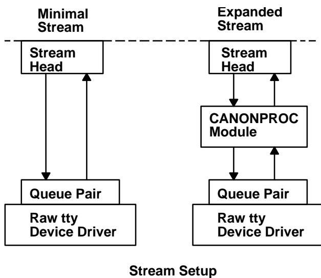
Figure 38. Stream Setup
