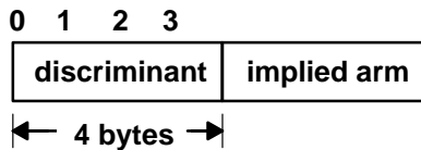
Discriminated Union
