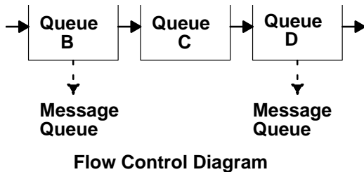
Figure 31. Flow Control
