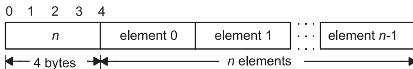
Variable-Length Array
