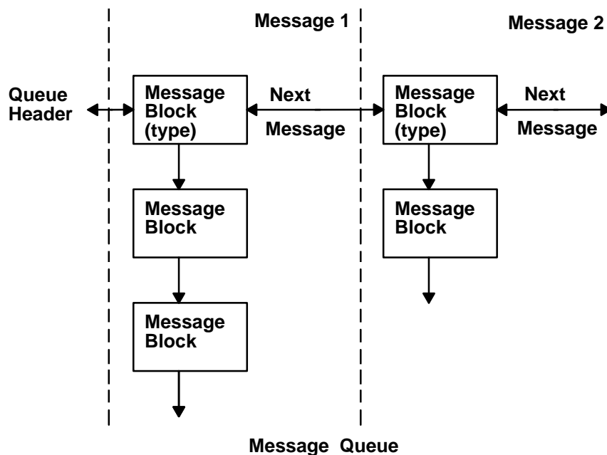
Figure 40. Message Queue
