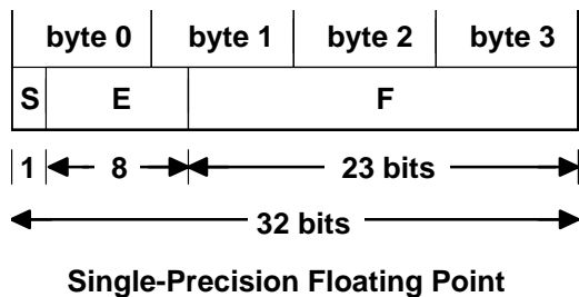
Figure 12. Single-Precision Floating-Point
