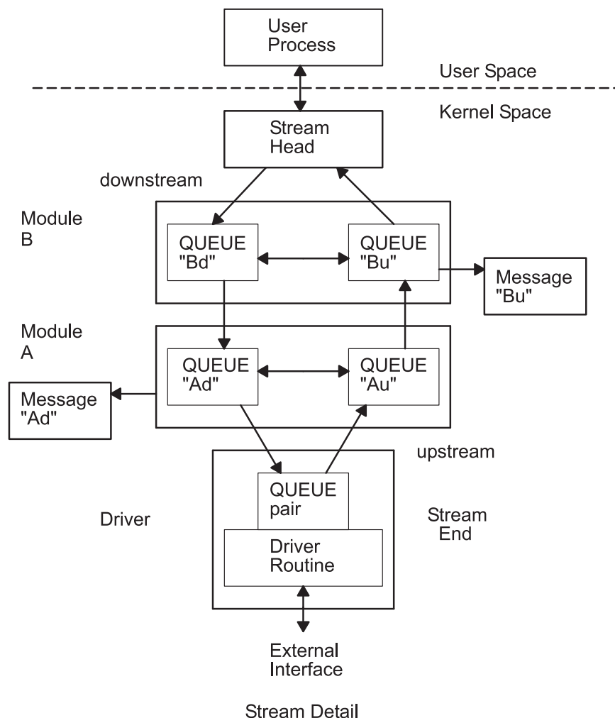
Figure 29. Stream Detail
