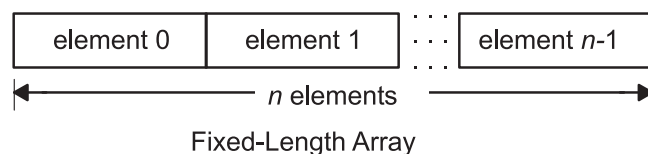
Figure 16. Fixed-Length Array.
