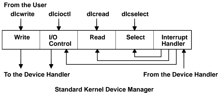
Figure 3. Standard Kernel Device Manager
