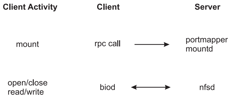
Figure 23. The Mount and NFS Process. This illustration is a three column table with Client Activity, Client, and Server as the three column headings. The first client activity is mount. An RPC call goes from the client to the server's portmapper mountd. The second client activity is open/close read/write. There is two-way interaction between the client's biod thread and the server's nfsd thread.
