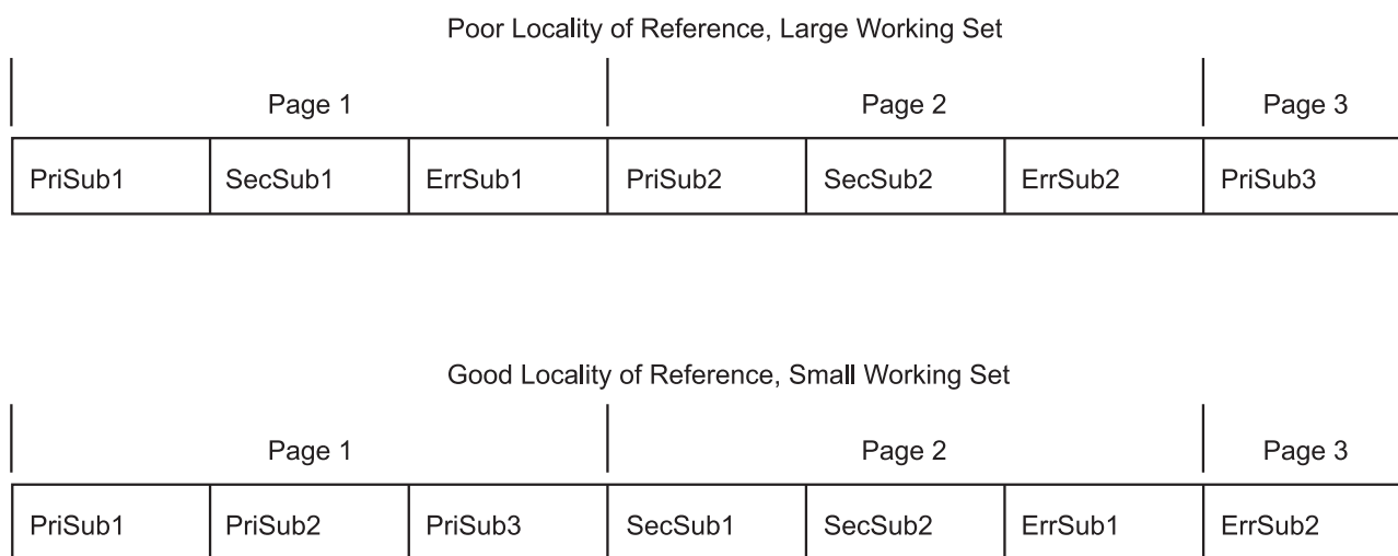
Figure 15. Locality of Reference. The top half of the figure describes how a binary program is packaged which shows low locality of reference. The instructions for PriSub1 is in the binary executable first, followed by the instructions for SecSub1 , ErrSub1 , PriSub2 , SecSub2 , ErrSub2 , and PriSub3 . In this executable, the instructions for PriSub1 , SecSub1 , and ErrSub1 occupy into the first page of memory. The instructions for PriSub2 , SecSub2 , ErrSub2 occupy the second page of memory, and the instructions for PriSub3 occupy the third page of memory. SecSub1 and SecSub2 are infrequently used; also ErrSub1 and ErrSub2 are rarely used, if ever. Therefore, the packaging of this program exhibits poor locality of reference and may use more memory than required. In the second half of the figure, PriSub1 , PriSub2 , and PriSub3 are located next to each other and occupy the first page of memory. Following PriSub3 is SecSub1 , SecSub2 , and ErrSub1 which all occupy the second page of memory. Finally, ErrSub2 is at the end and occupies the third page of memory. Because ErrSub2 may never be needed, it would reduce the memory requirements by one page in this case.
