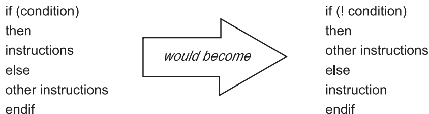
Figure 16. Example of Conditional Branch Recoding. The illustration shows how conditional branch recoding changes certain code. For example, the code If (condition) would become If (! condition) ; the code then stays then ; instructions becomes other instructions ; else stays else ; other instructions become instruction ; and endif stays endif .
