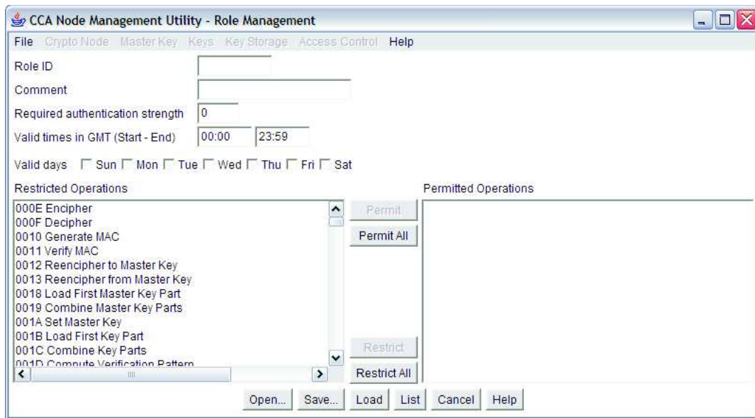
Figure 3. Role Management window
