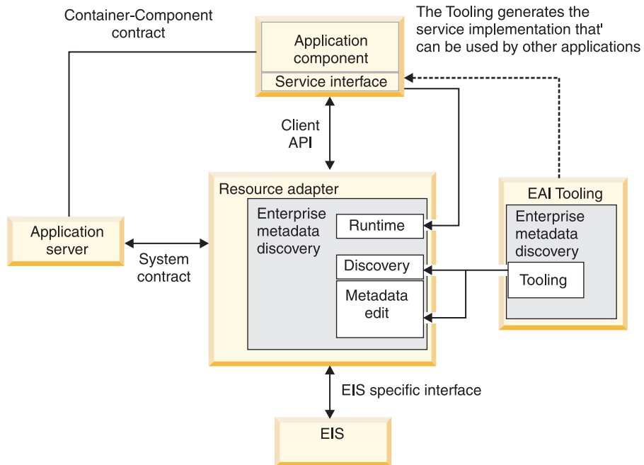
Enterprise metadata discovery architecture
