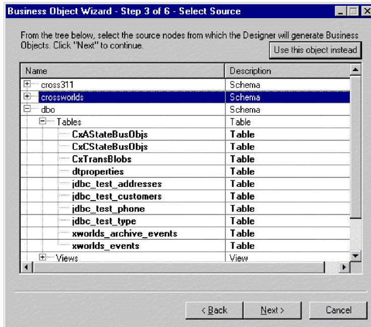
Figure 8. Tree of Schema with Expanded Nodes
