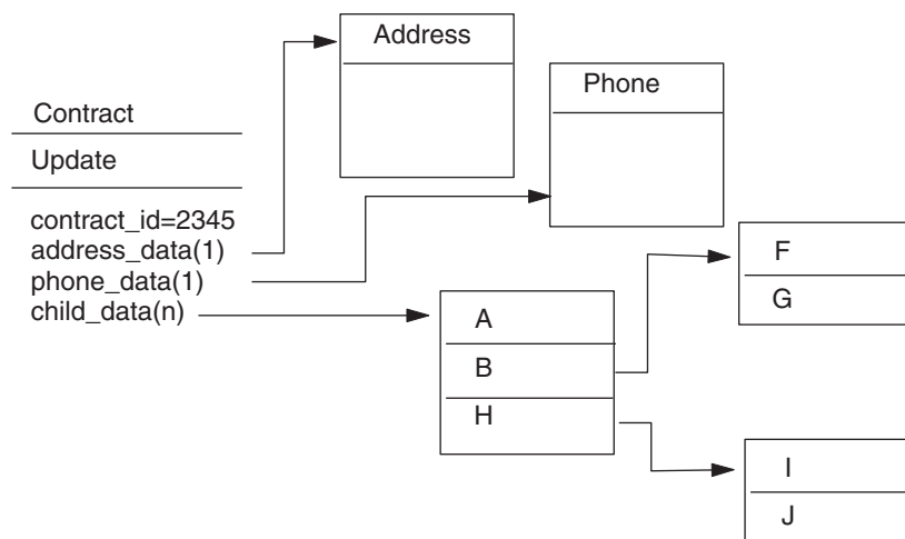
Figure 5. Example of relationships among business objects
