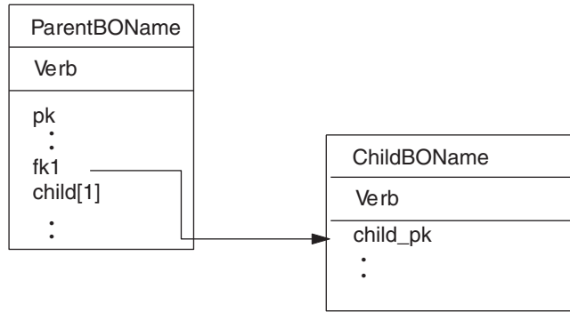
Figure 3. Multiple-cardinality business object relationship
