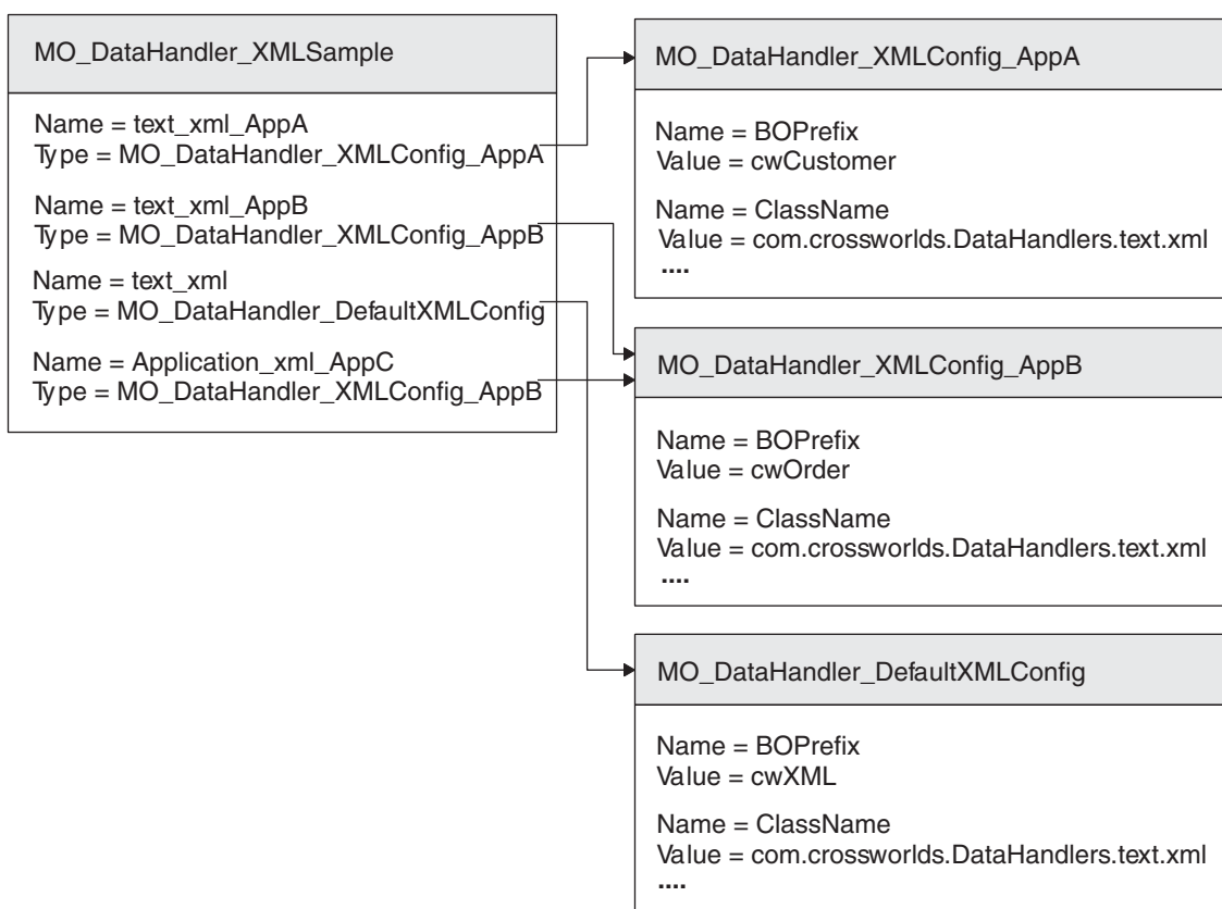
Figure 12. Example meta-object for multiple XML data handlers
