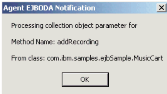
Figure 11. Verify class and method
