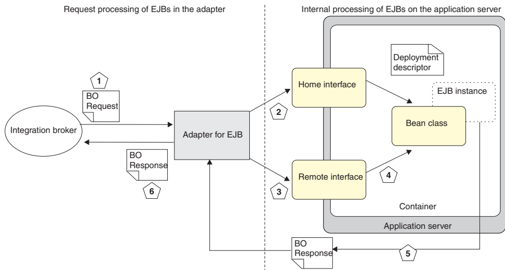
Figure 1. Request processing for the connector for EJB architecture
