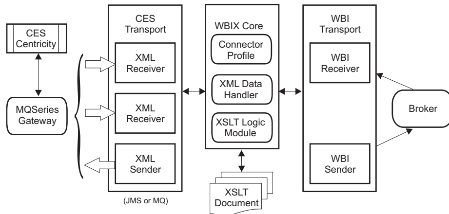
Figure 1. Detail view of the adapter for CES Centricity Gateway architecture
