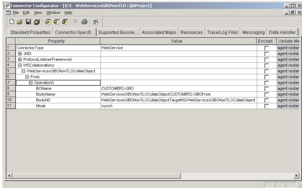
Figure 61. WSCollaborations
