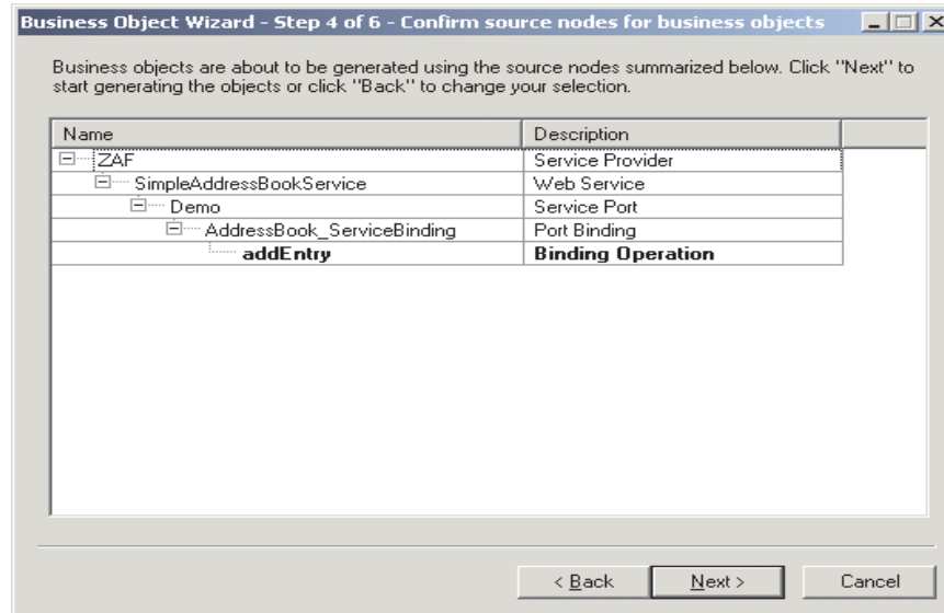
Figure 67. Confirm window
