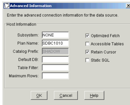
Figure 4–3. Advanced Information
