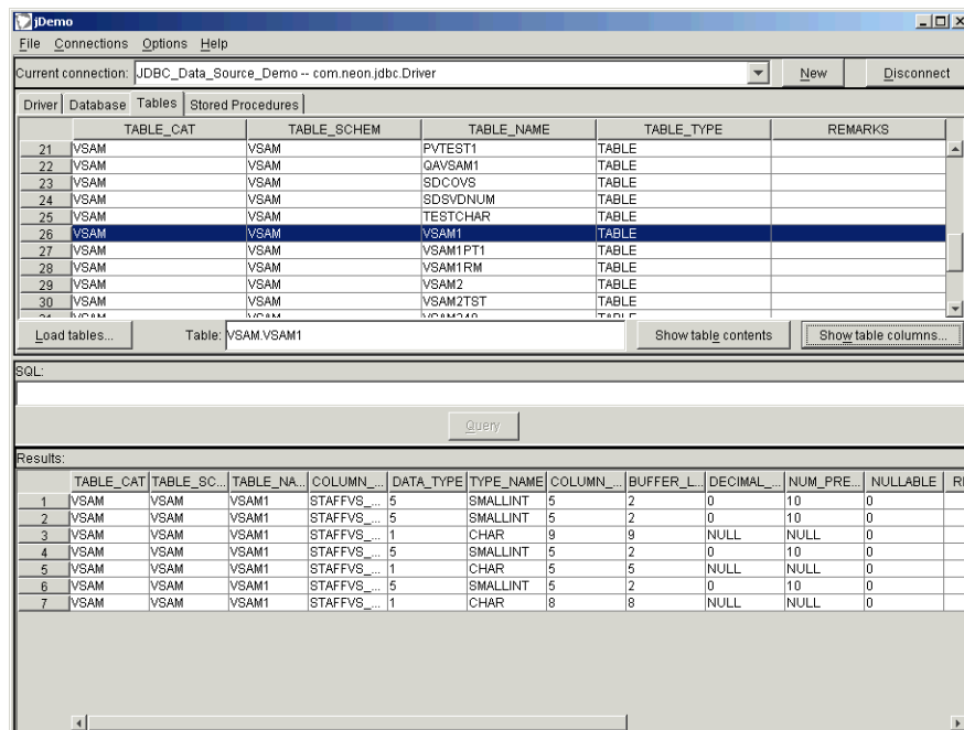
Figure 5–11. Table Columns
