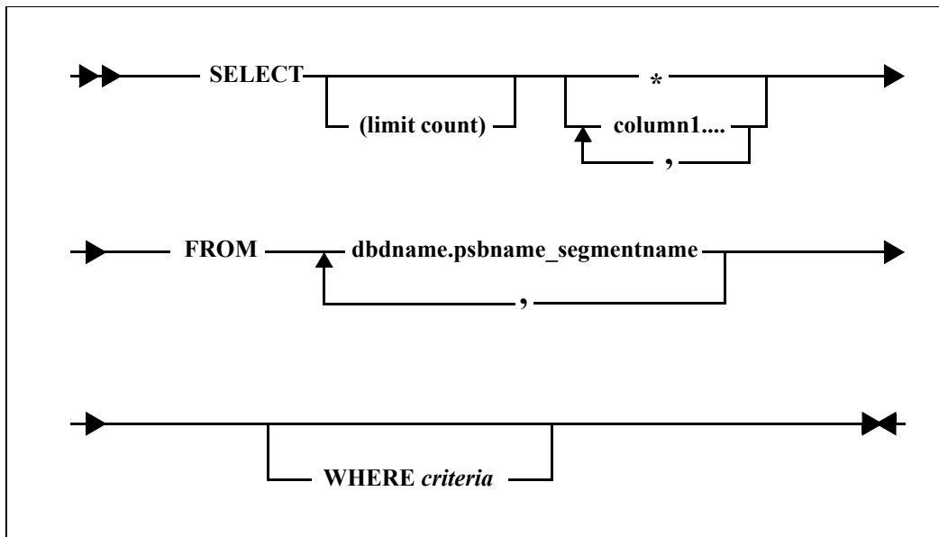
Figure 7-1. SELECT Statement Syntax
