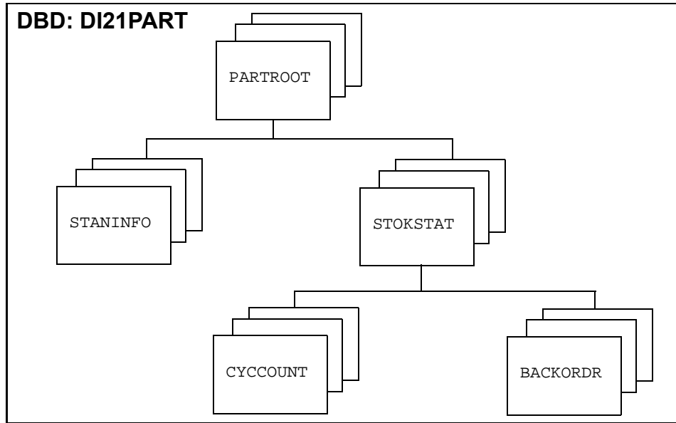
Figure 7–3. IMS Database Representation
