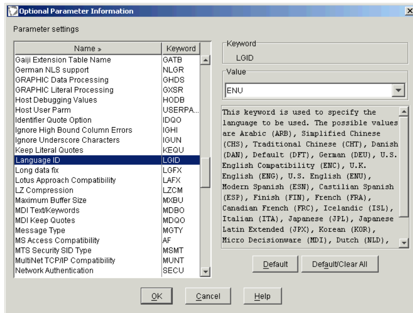
Figure B–1. Optional Parameters Information -- Setting the Language ID
