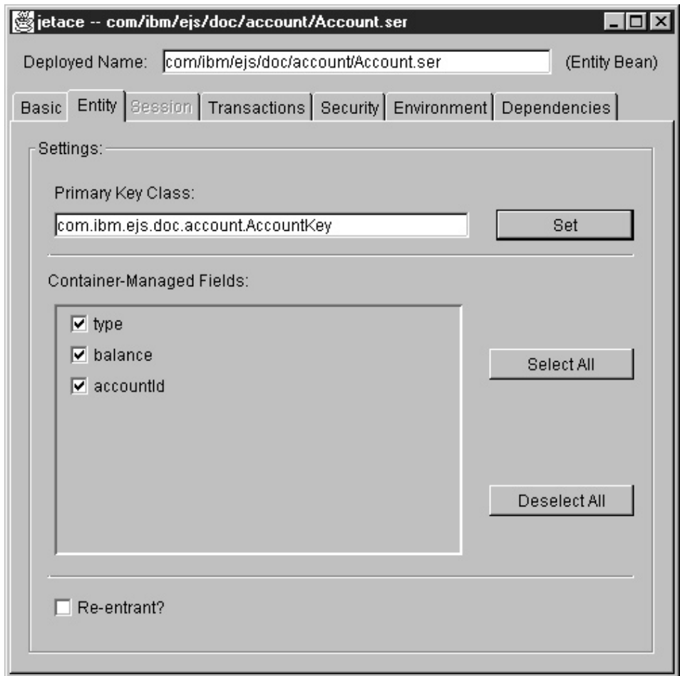
Figure 12. The Entity page of the jetace tool
