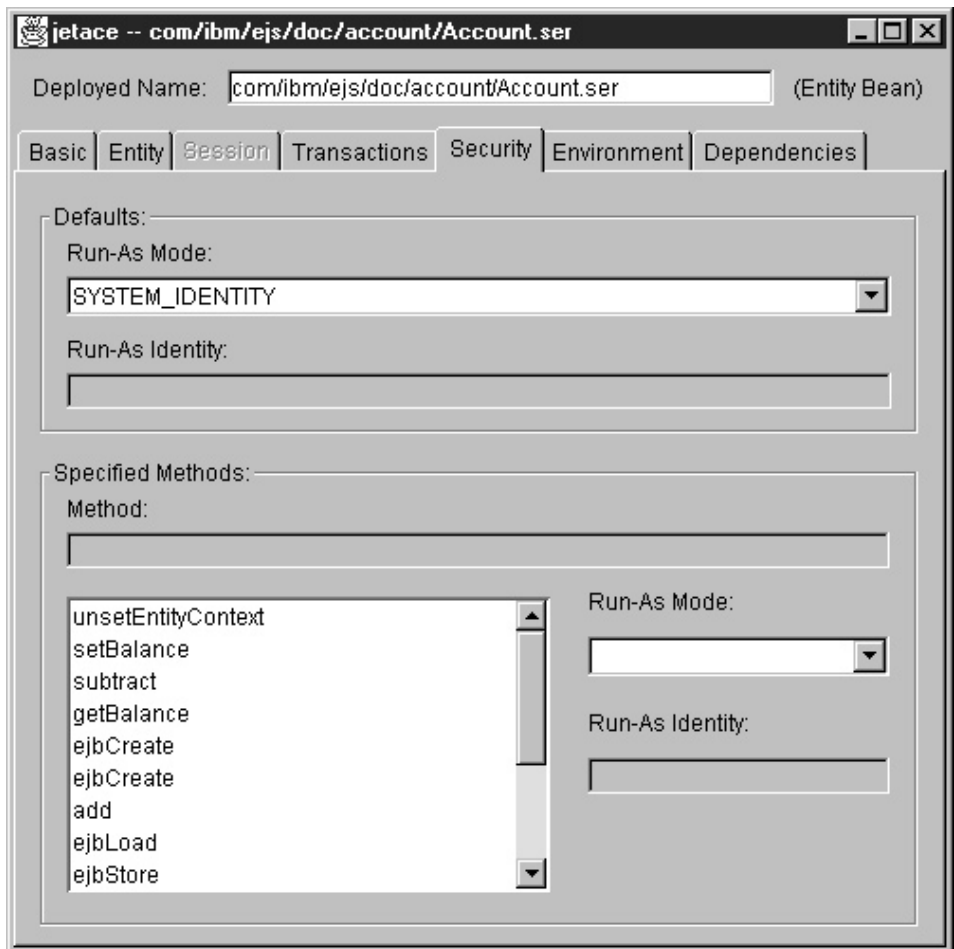
Figure 15. The Security page of the jetace tool
