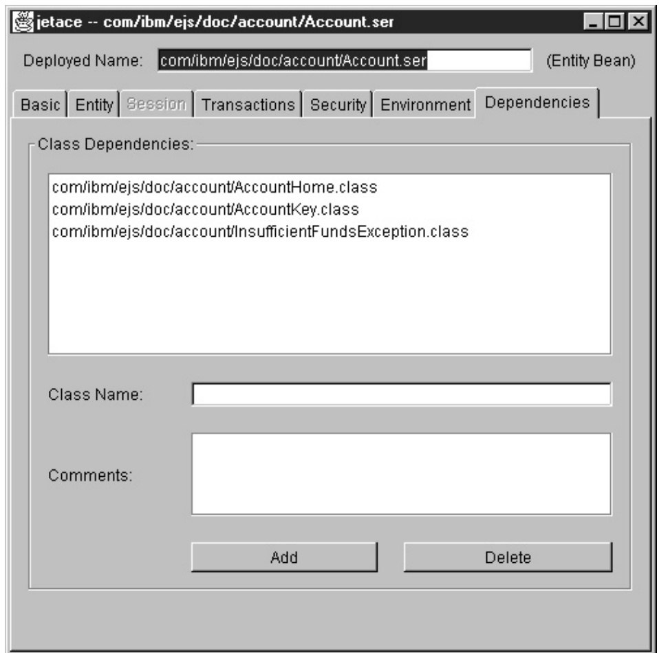
Figure 17. The Dependencies page of the jetace tool
