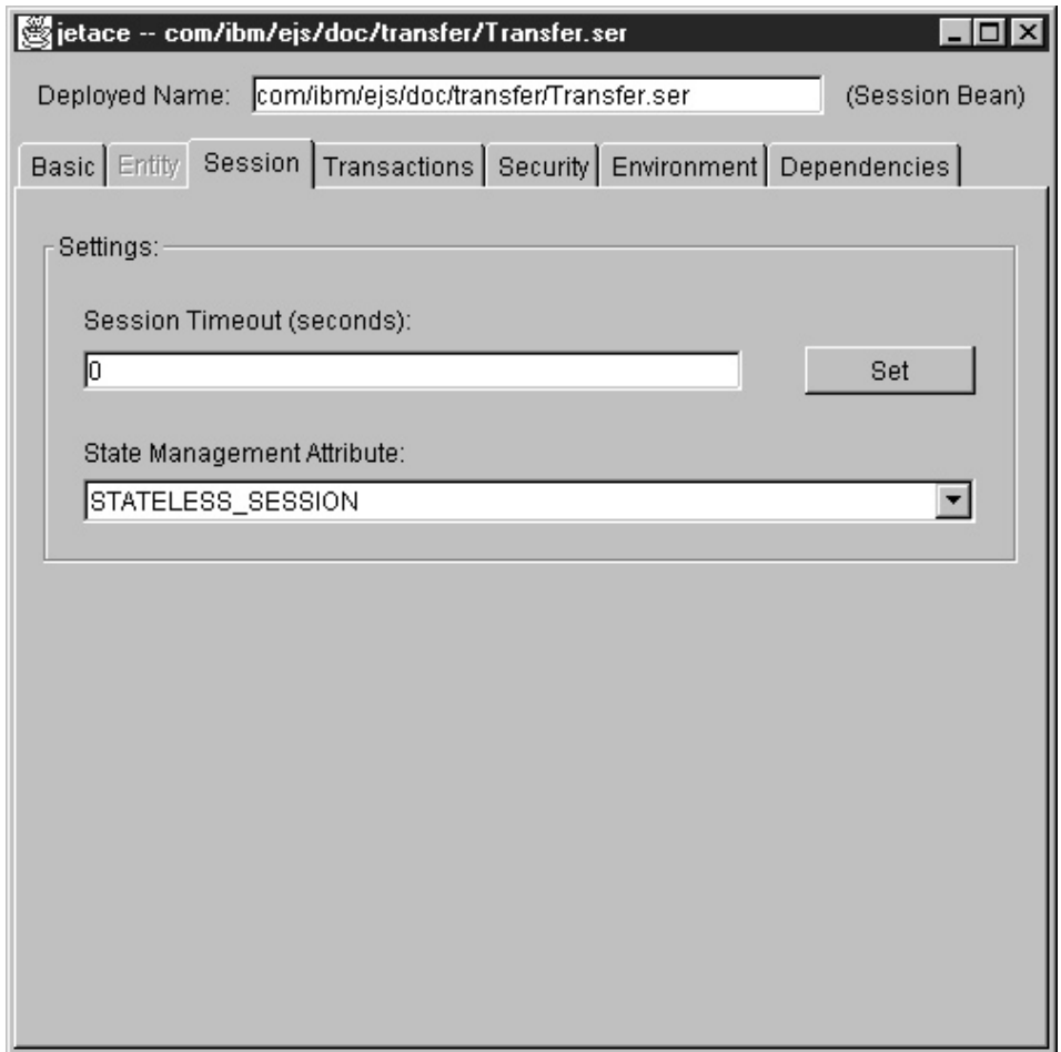
Figure 13. The Session page of the jetace tool
