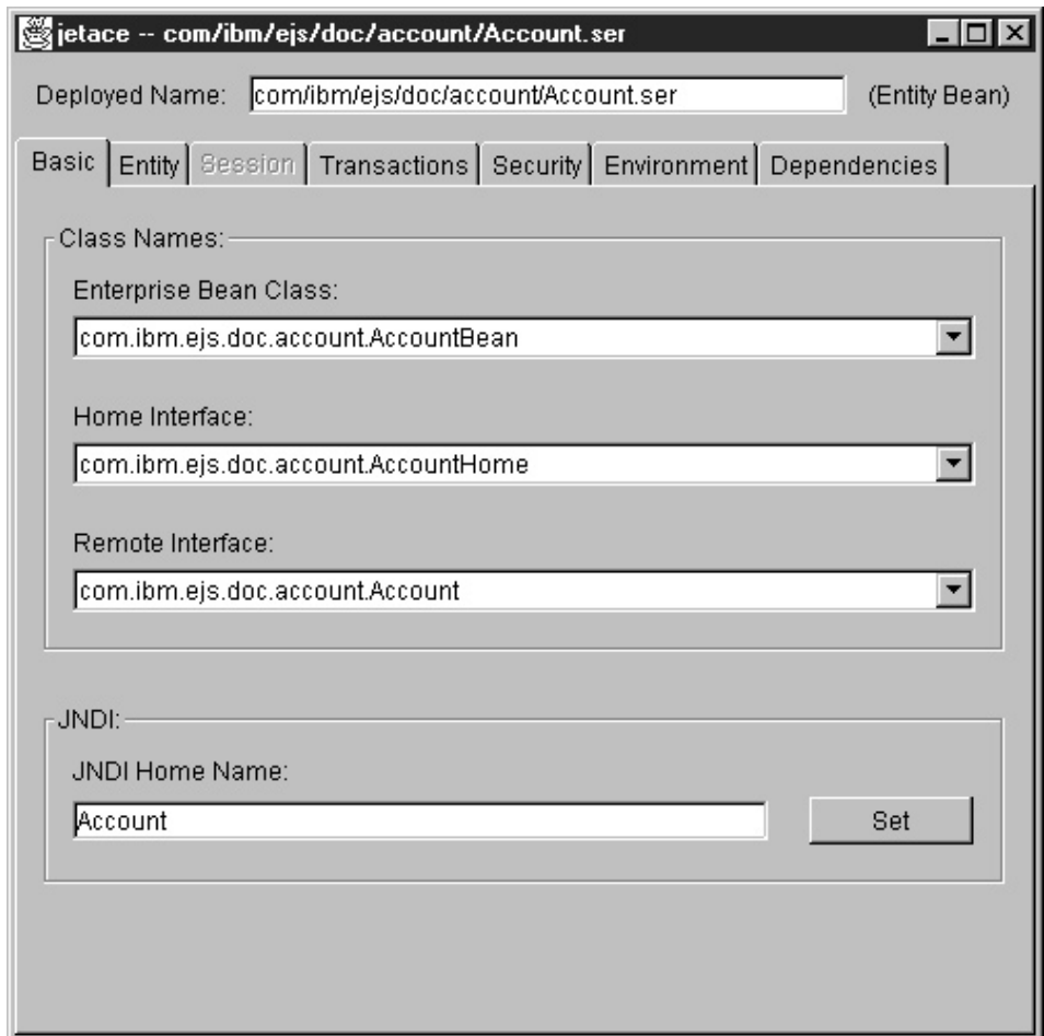
Figure 11. The Basic page of the jetace tool
