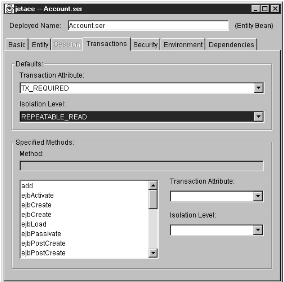
Figure 14. The Transactions page of the jetace tool
