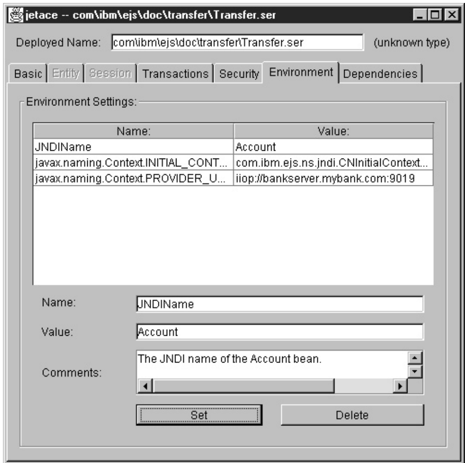
Figure 16. The Environment page of the jetace tool
