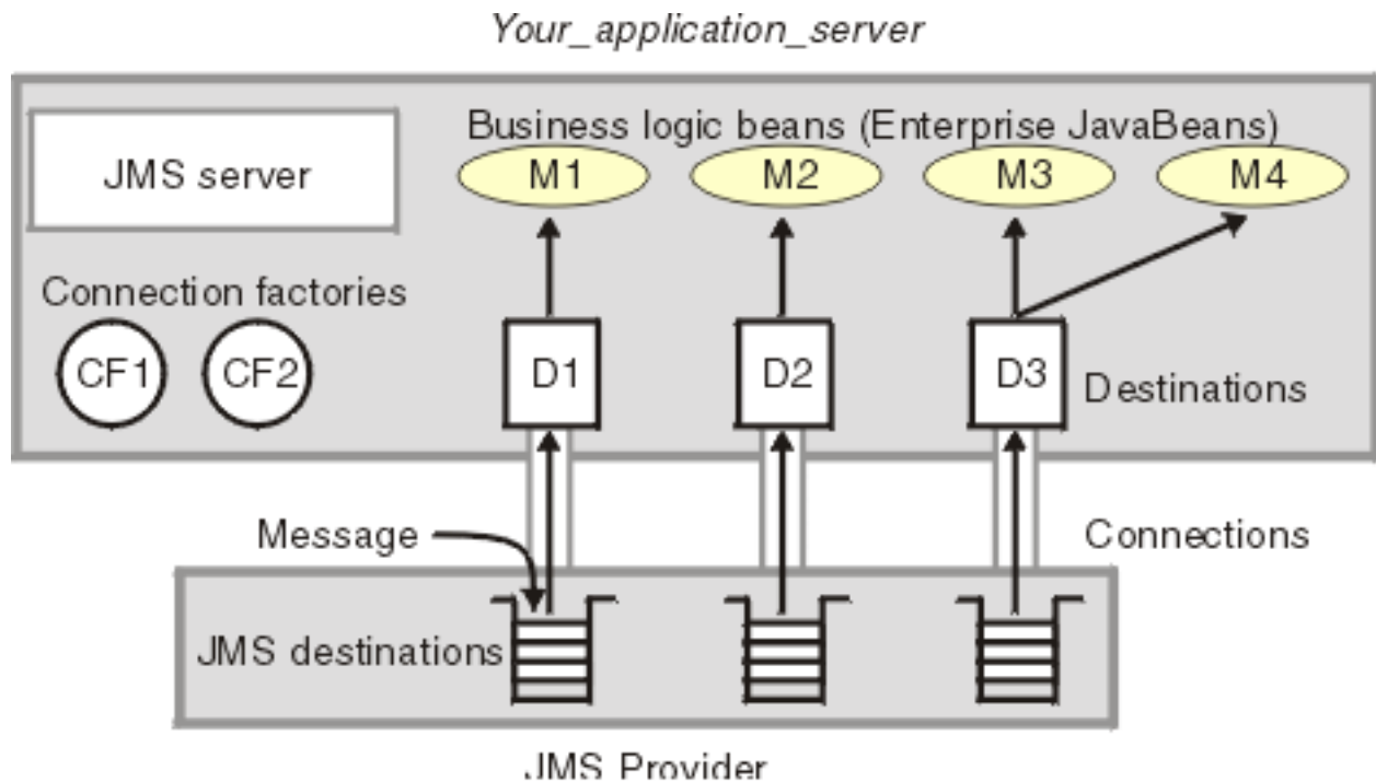
Figure 3. The main components of WebSphere JMS support (Application Server)
