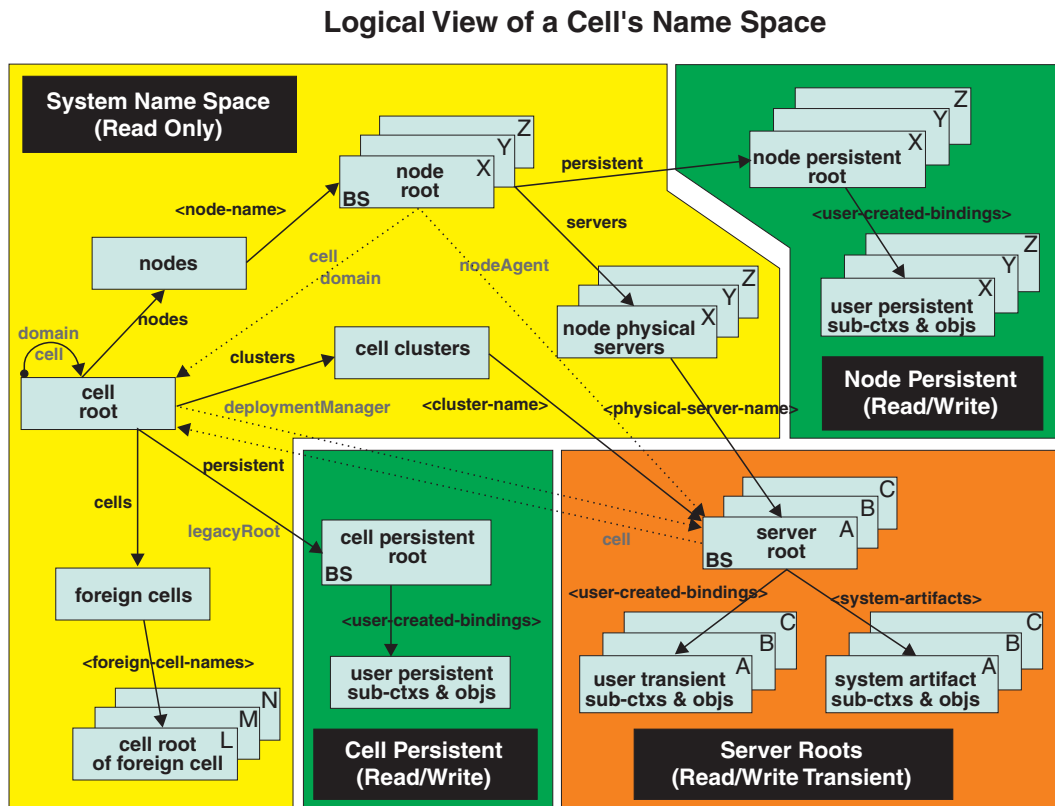
Figure 19. Name Space Logical View
