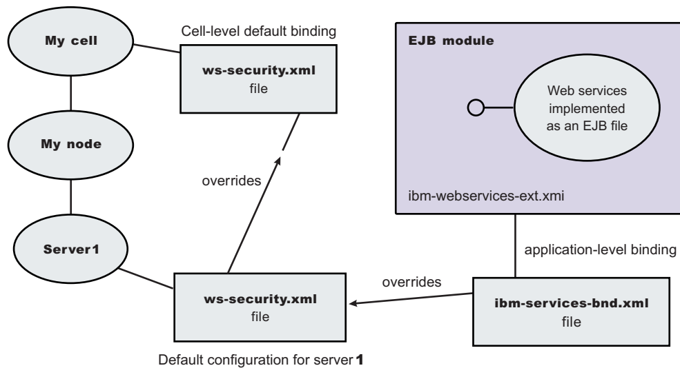
Figure 14. Run-time configuration
