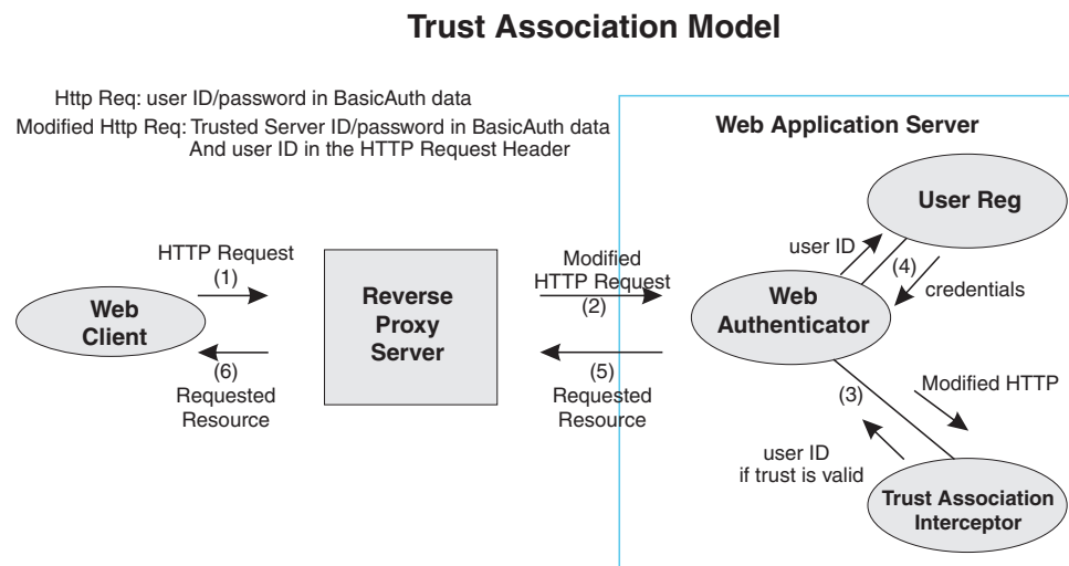
Figure 1. Trust association
