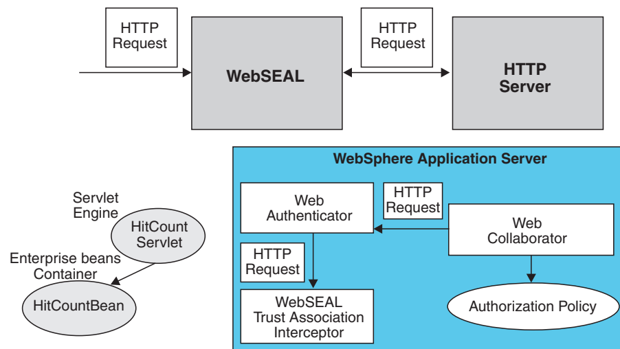
Figure 3. HTTP server
