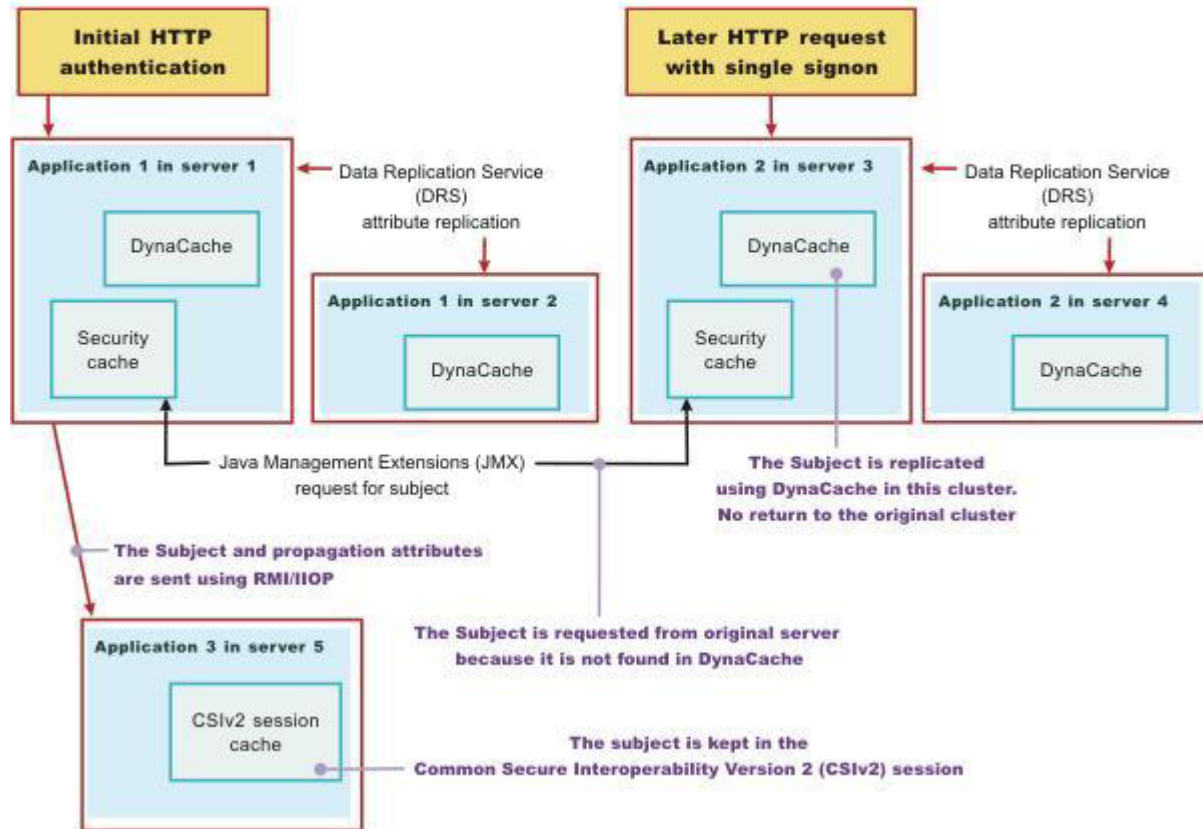
Figure 22. Horizontal propagation
