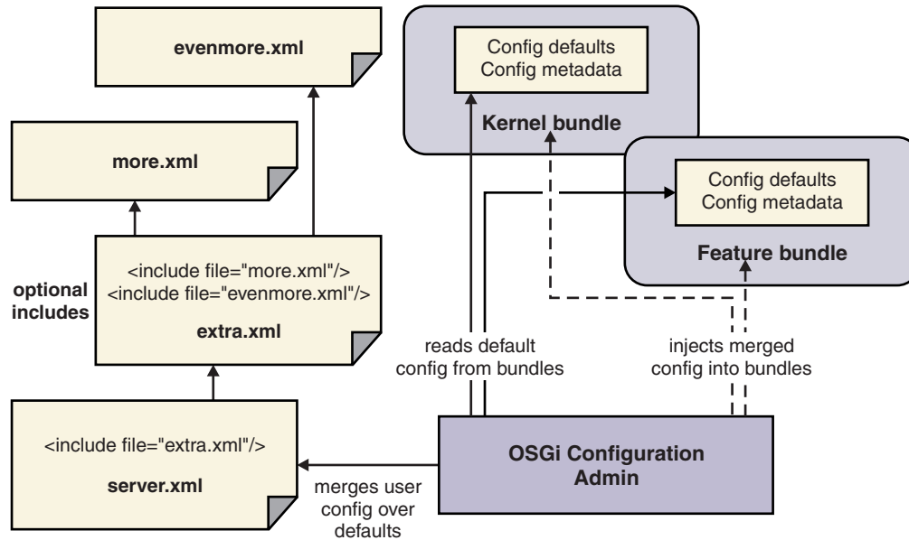
Figure 32. Configuration management
