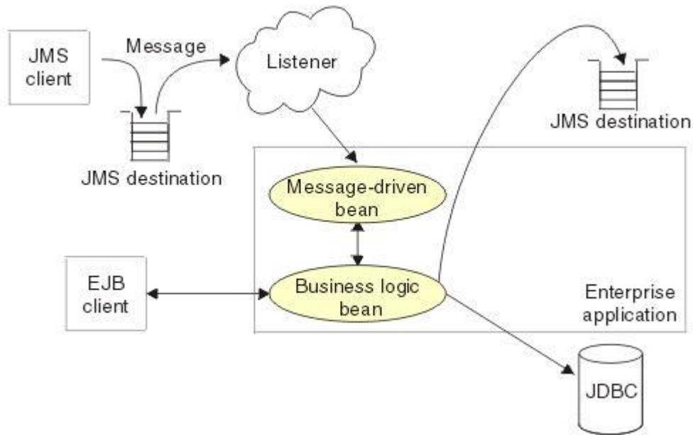
Figure 84. Messaging with message-driven beans
