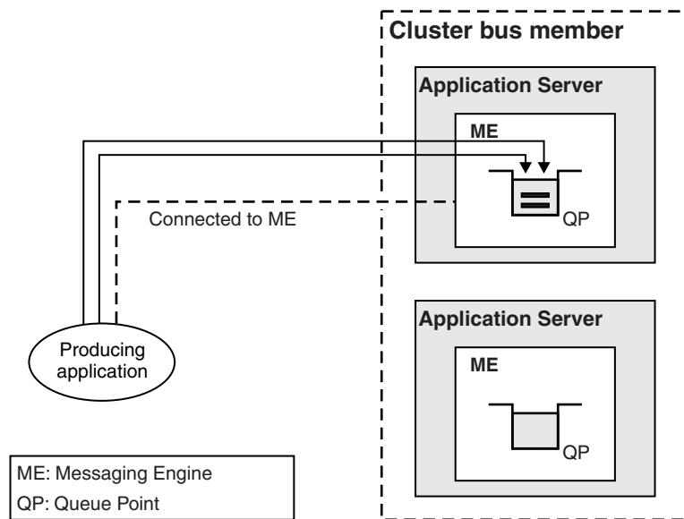
Figure 113. Default behavior: messages are sent to the local queue point
