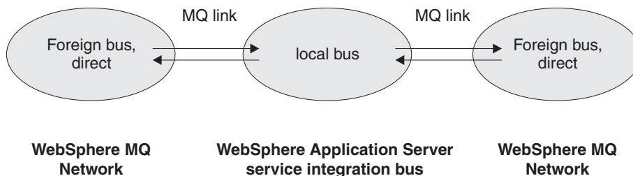
Figure 77. Exchanging messages between two WebSphere MQ networks through an intermediate application server.
