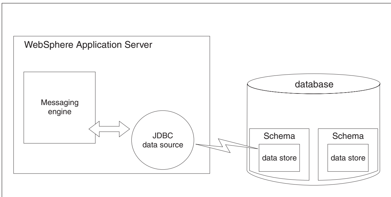
Figure 110. The relationship between a messaging engine and its data store.
