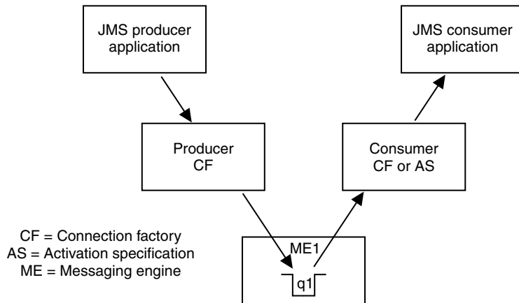
Figure 46. Producing and consuming messages
