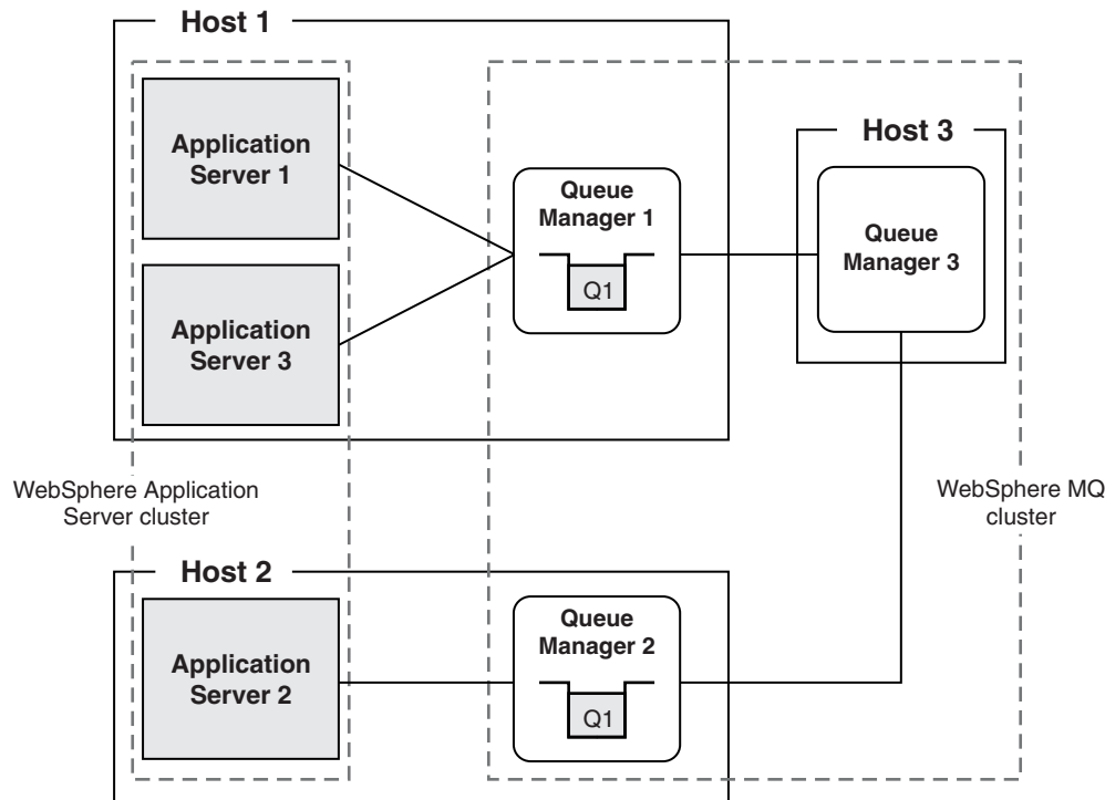
Figure 53. WebSphere Application Server clustering: bindings mode attachment to queue managers
