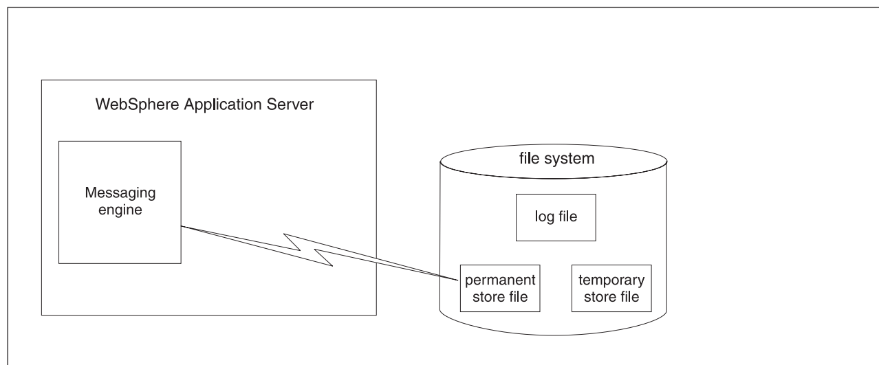
Figure 109. The relationship between a messaging engine and its file store
