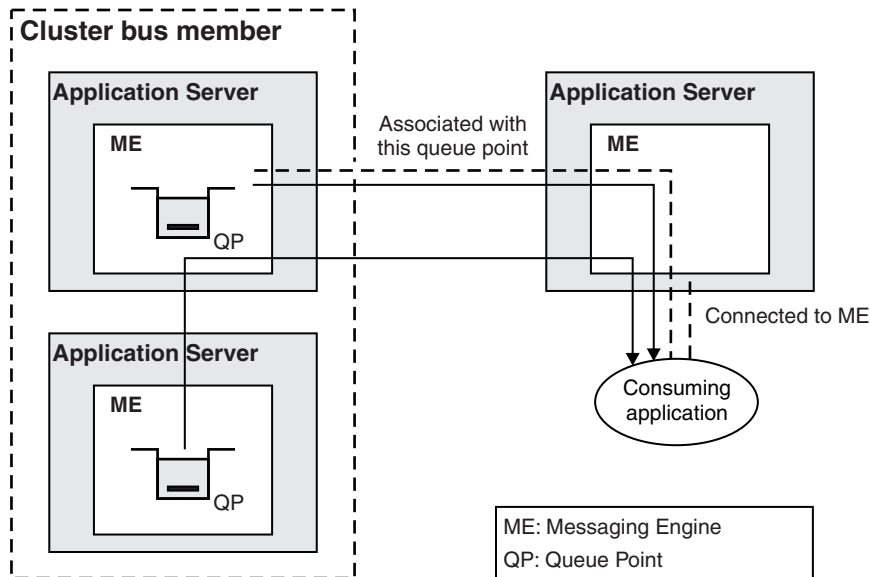
Figure 118. Message gathering: messages are consumed from all queue points
