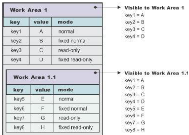
Figure 182. Defining new properties in nested work areas
