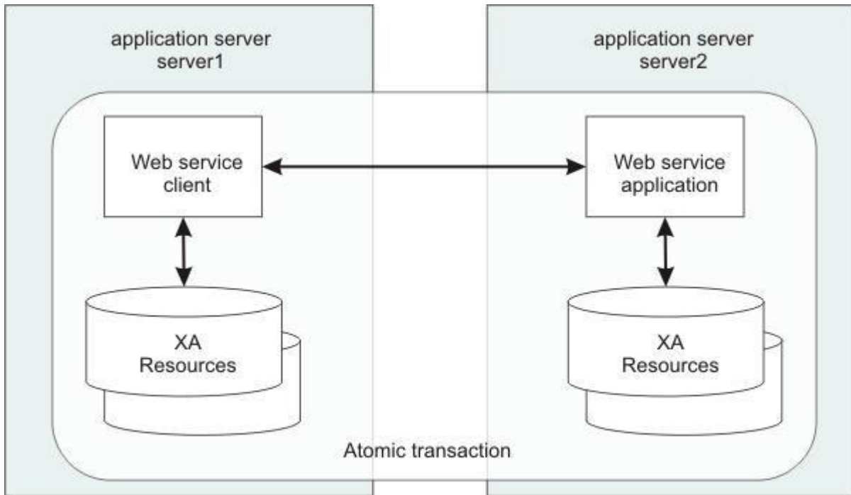
Figure 192. Transaction context shared between two application servers
