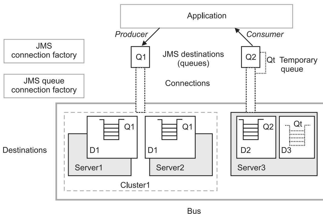
Figure 36. JMS point-to-point messaging and the default messaging provider
