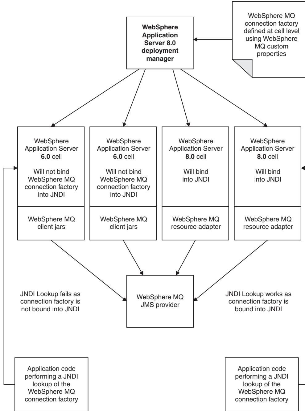
Figure 57. Mixed node scenario
