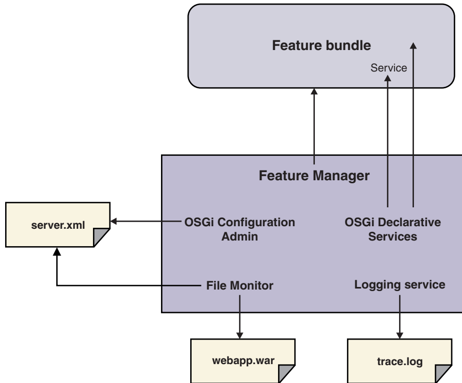
Figure 30. Liberty profile kernel
