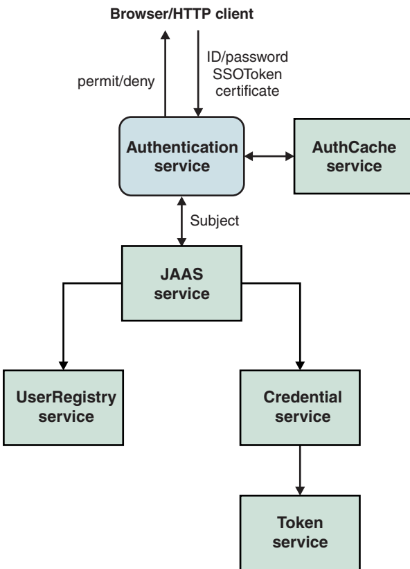
Figure 34. Overview of authentication process
