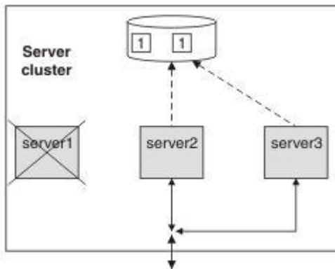
Figure 24. Server 1 fails. Servers 2 and 3 become blocked as a result
