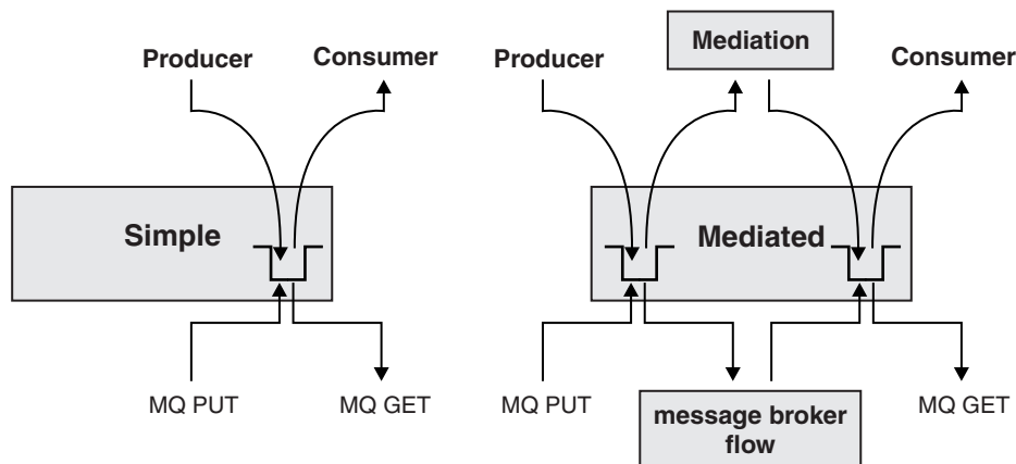
Figure 83. Queue-type destinations assigned to a WebSphere MQ server bus member. Queue points and mediation points can be queues of WebSphere MQ messages held in WebSphere MQ. A WebSphere Message Broker, or other WebSphere MQ application, can run mediations externally.
