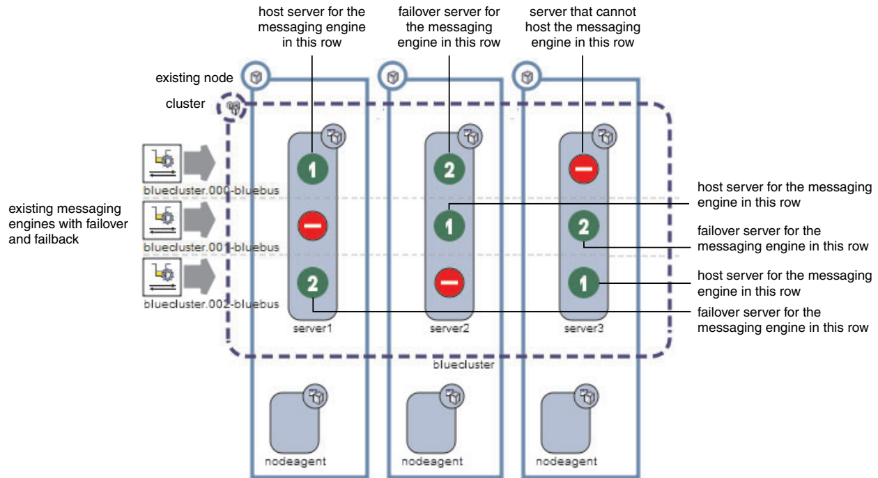
Figure 147. Scalability with high availability policy selected with a suitable system configuration
