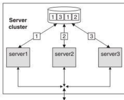
Figure 23. Server cluster up and running, just before server failure
