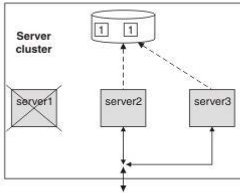
Figure 13. Server 1 fails. Servers 2 and 3 become blocked as a result
