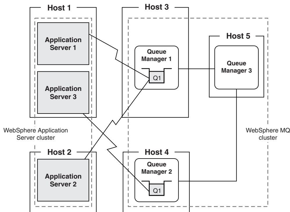
Figure 52. WebSphere Application Server clustering: client mode attachment to queue managers
