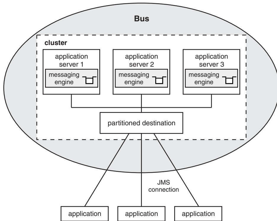
Figure 153. Service integration bus with partitioned destinations
