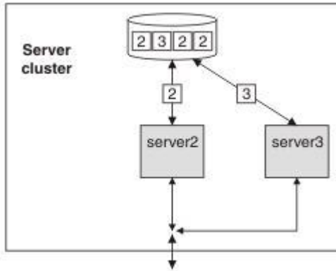
Figure 15. Server cluster stable again with just two servers: server 2 and server 3
