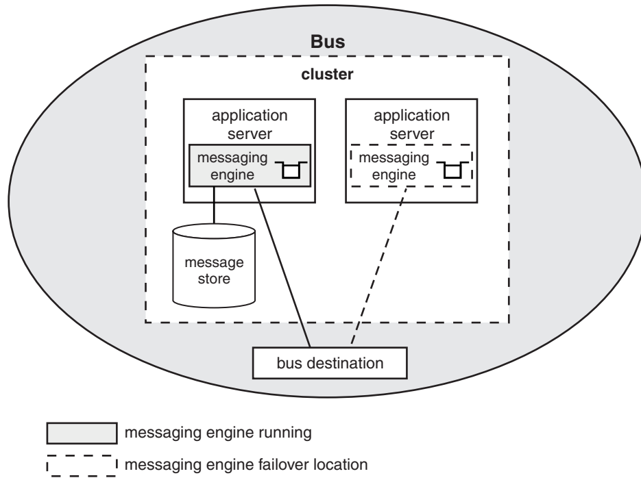
Figure 152. Service integration bus with clustered server
