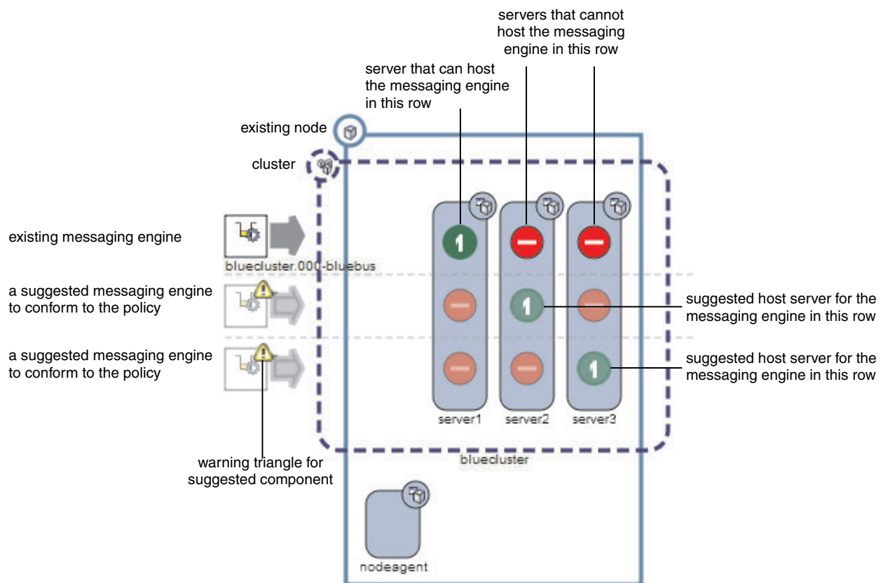
Figure 144. Scalability policy selected without a suitable messaging engine configuration
