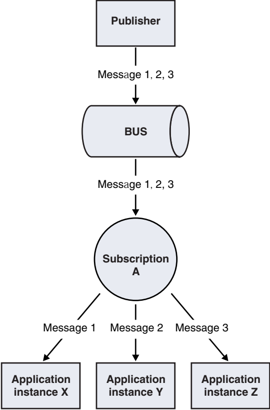
Figure 100. Application instances that share a single subscription (workload sharing)
