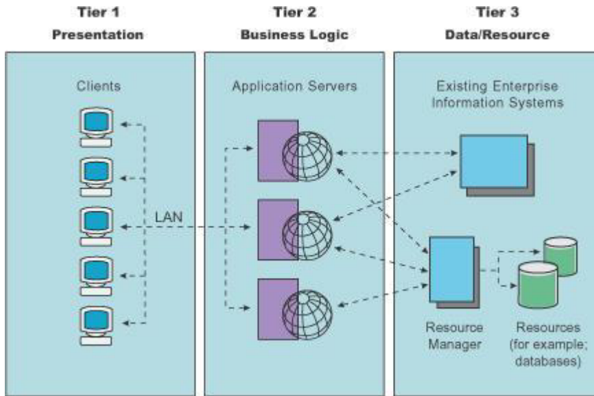
Figure 193. Three tier architecture
