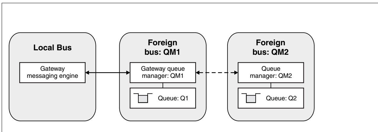
Figure 61. Addressing a WebSphere MQ queue in an indirectly connected foreign bus
