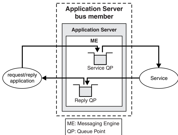
Figure 120. A service integration bus queue destination defined to an application server bus member
