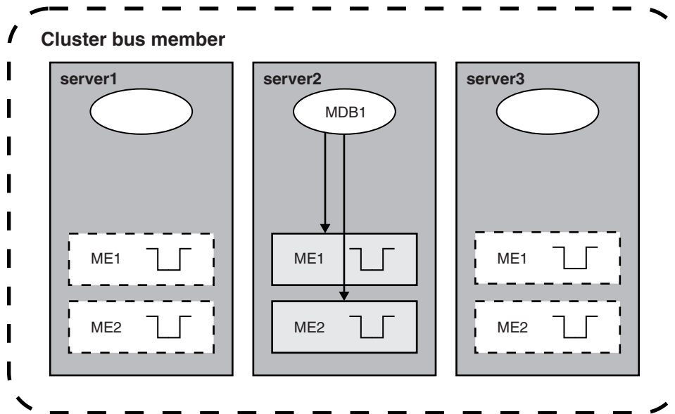
Figure 42. MDB is driven by servers in the cluster bus member that hosts a started messaging engine (setup 2)
