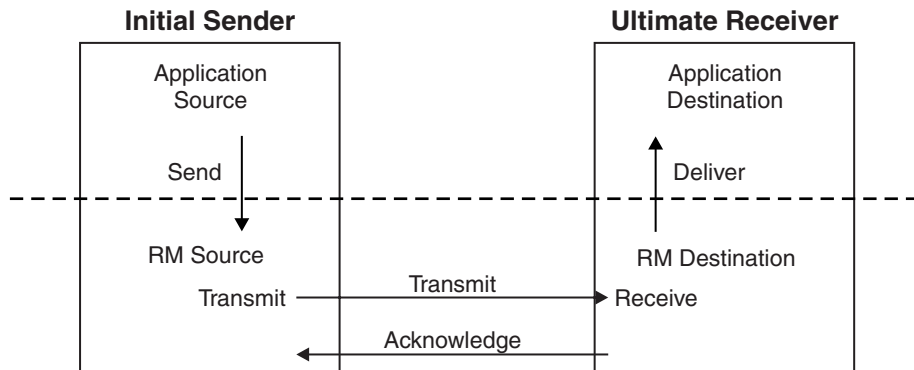
Figure 190. The interactions used to exchange web services messages reliably.
