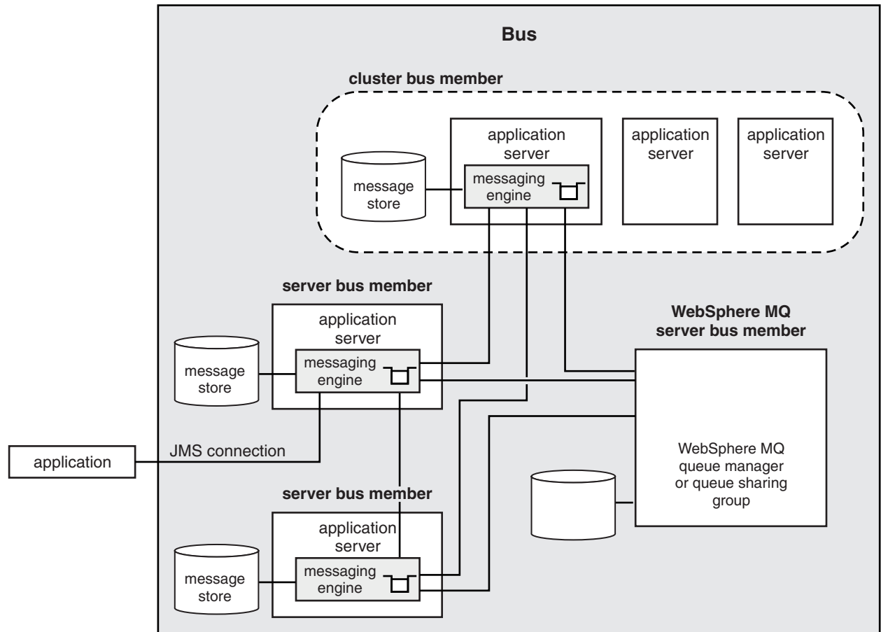
Figure 95. Bus members
