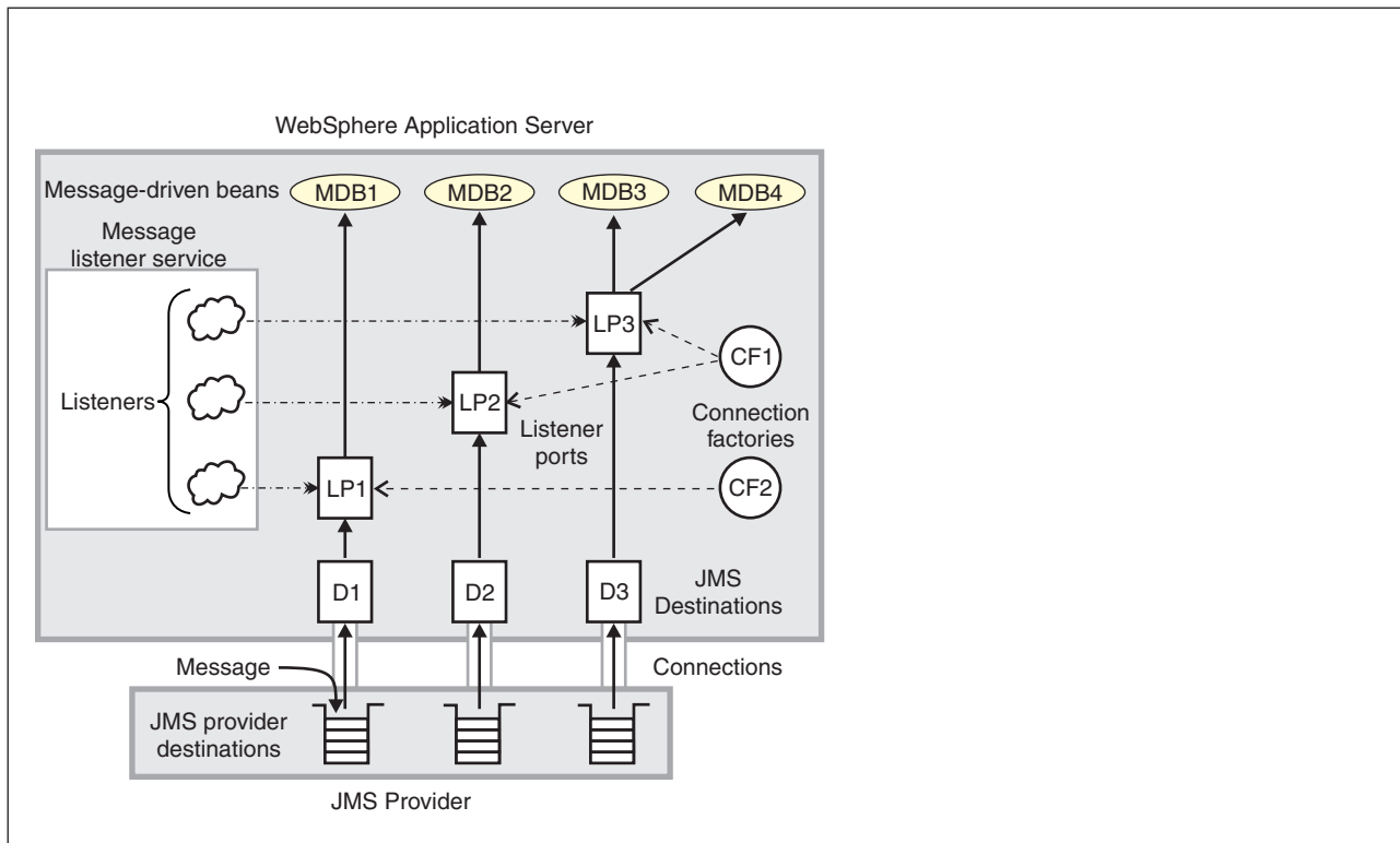
Figure 87. The main components for message-driven beans
