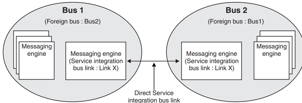
Figure 168. Direct connection between two service integration buses by using a service integration bus link
