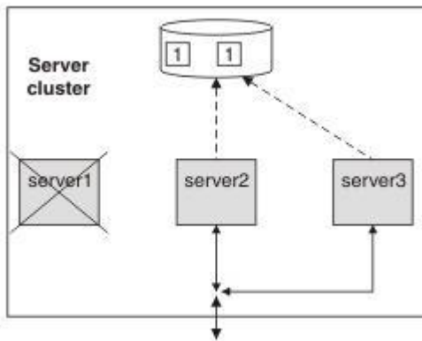
Figure 177. Server 1 fails. Servers 2 and 3 become blocked as a result
