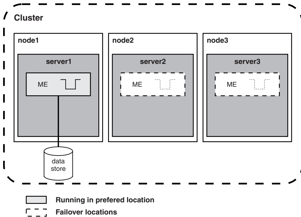
Figure 132. Highly available messaging engine configuration
