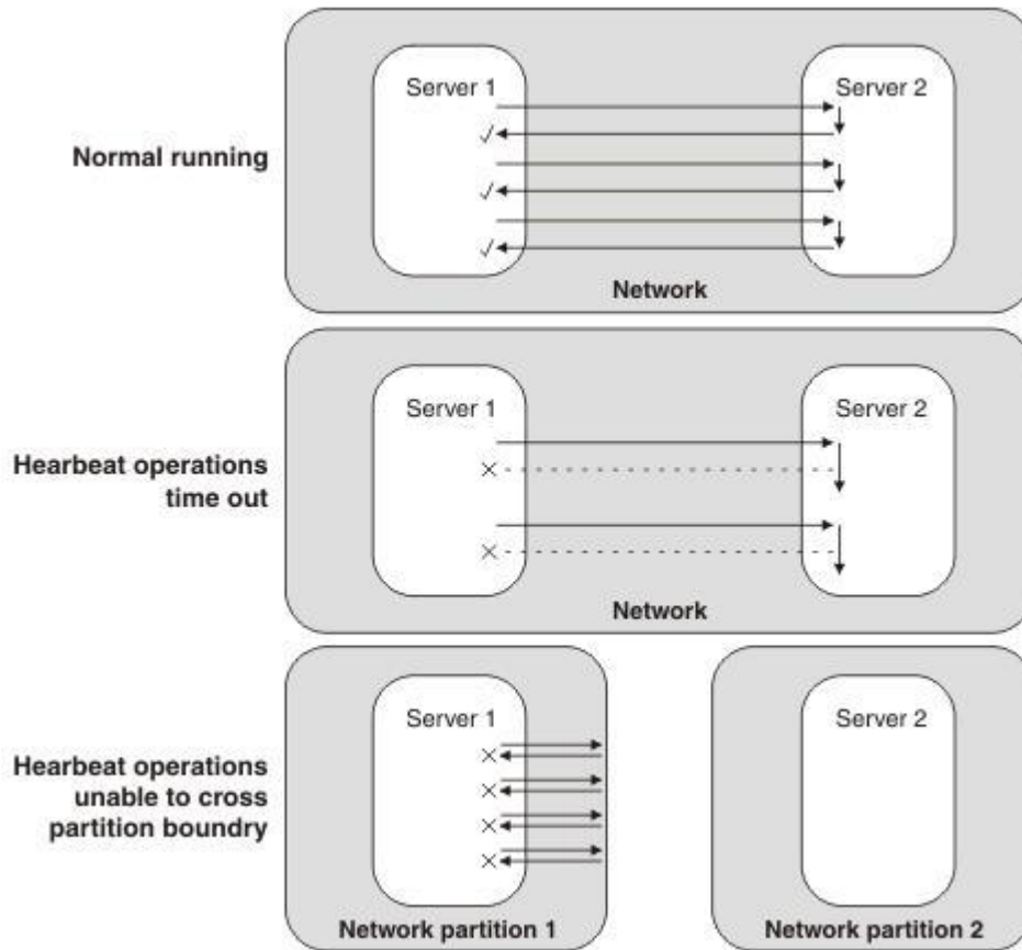
Figure 28. Heartbeats in a system running normally, compared to heartbeats after the apparent server failures of system overloading and network partitioning
