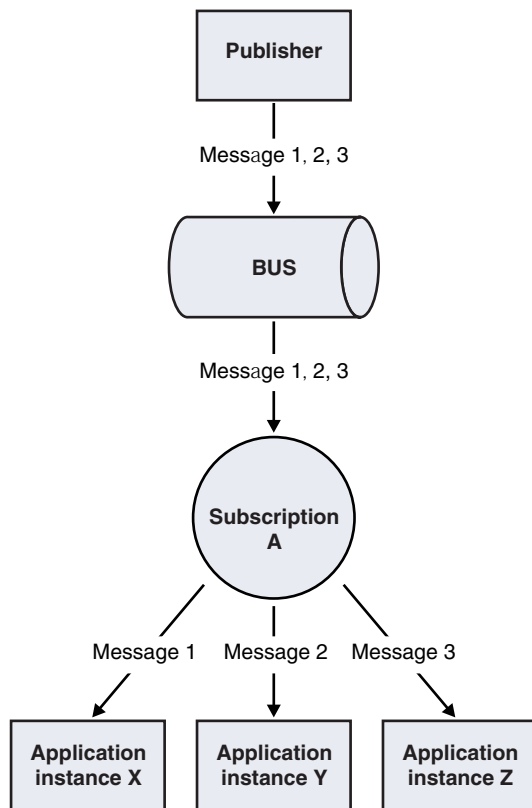
Figure 128. Application instances that share a single subscription (workload sharing)
