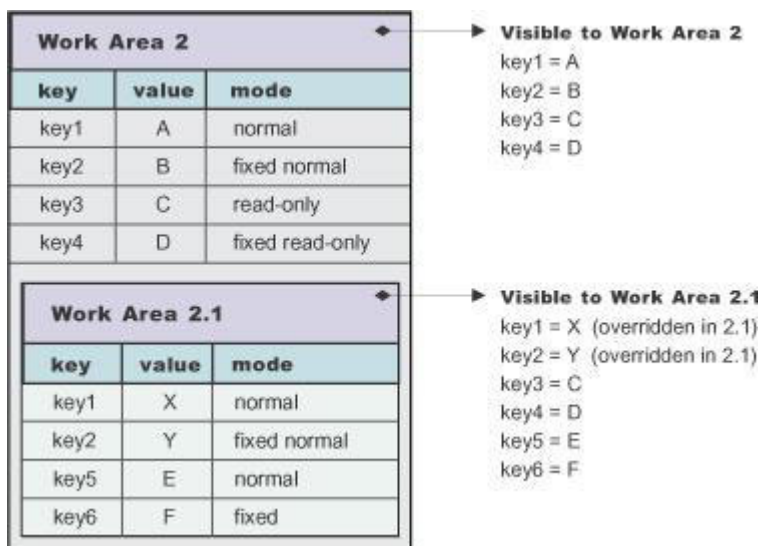
Figure 183. Redefining existing properties in nested work areas
