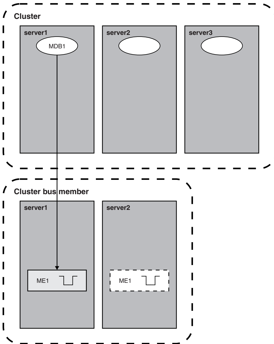
Figure 45. One server receiving messages from messaging engine in a cluster bus member
