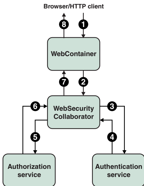
Figure 33. Typical security flow for web resources
