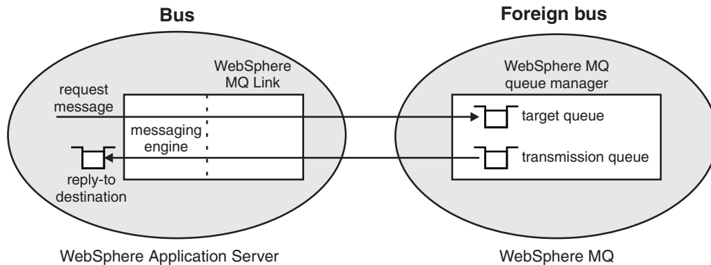
Figure 71. Paths taken by a message and response exchanged between a messaging engine on a bus and a queue manager in WebSphere MQ
