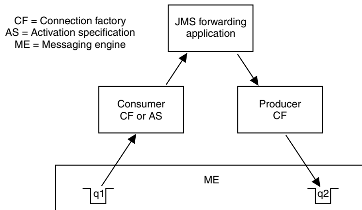
Figure 47. Forwarding messages
