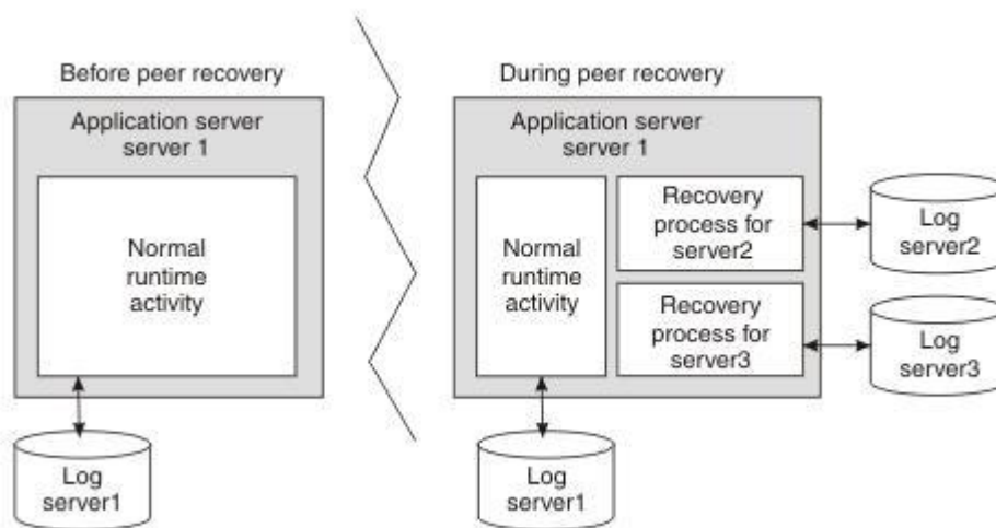
Figure 11. Peer recovery
