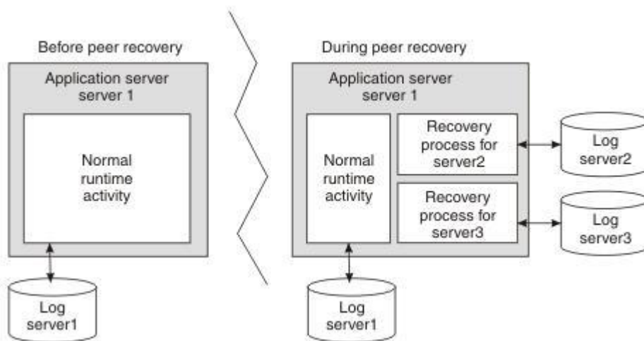
Figure 22. Peer recovery
