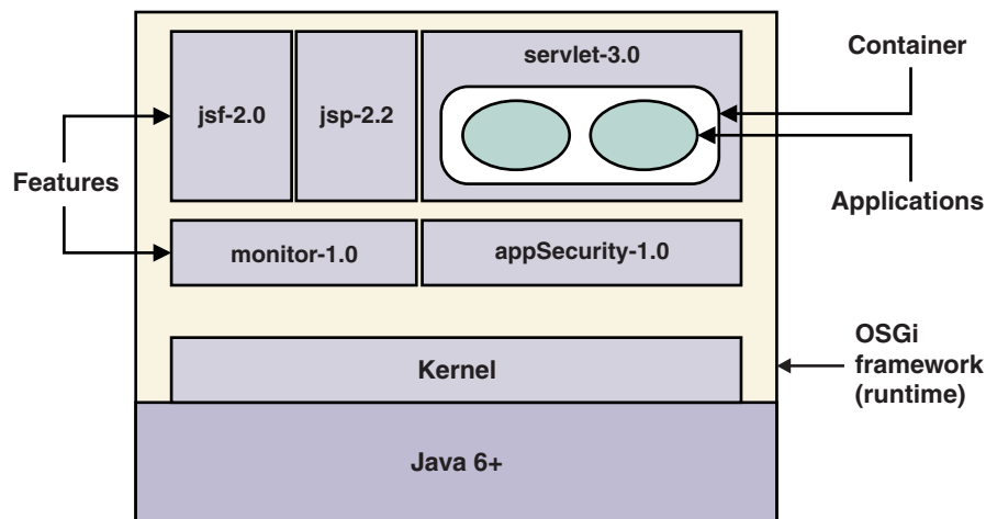
Figure 29. Liberty profile architecture
