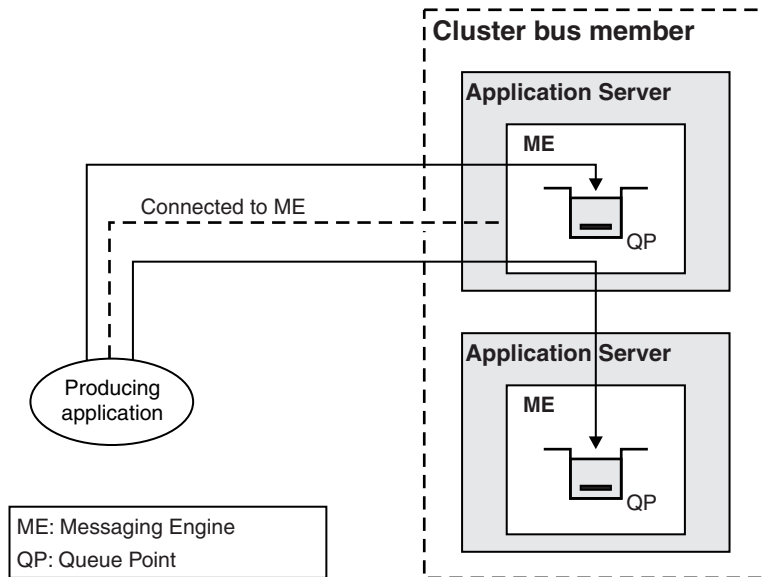
Figure 115. Disable Prefer local queue point: messages are workload balanced across all queue points
