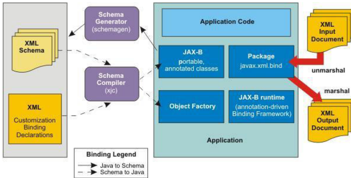
Figure 184. JAXB architecture
