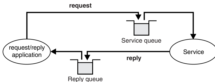
Figure 119. Typical JMS messaging pattern
