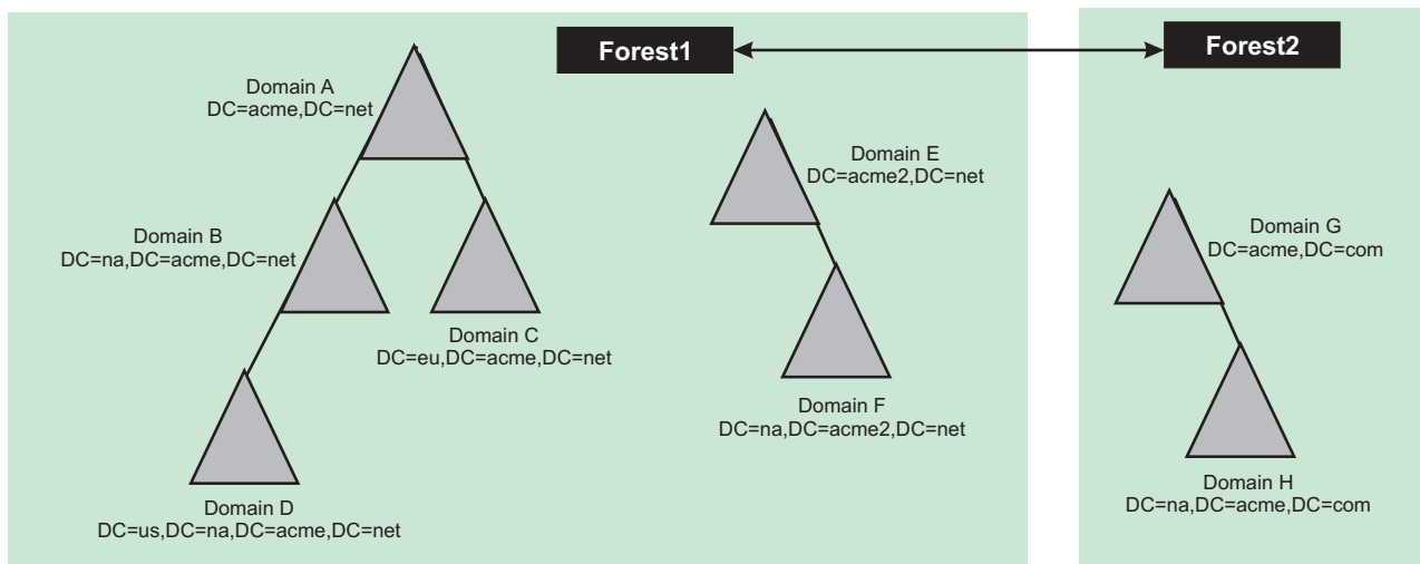
Figure 24. Microsoft Active Directory forests. An illustration of Microsoft Active Directory forests.
