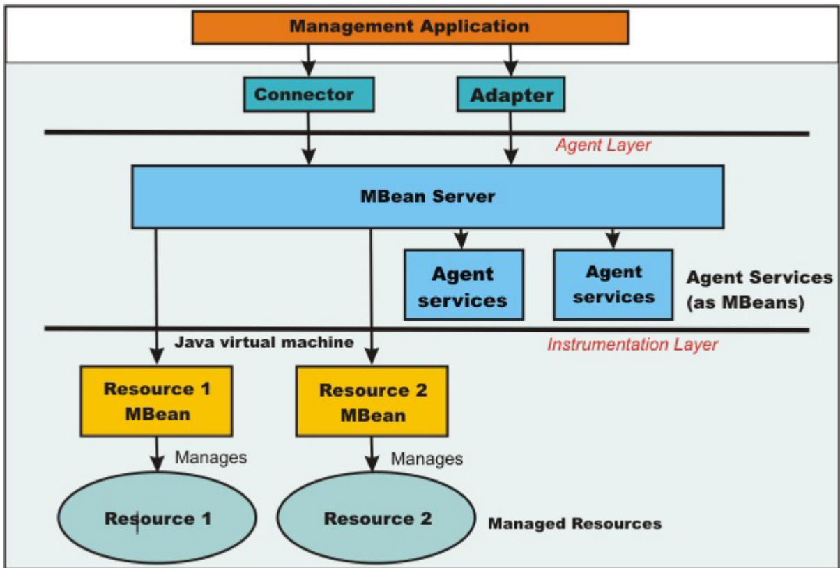
Figure 1. JMX architecture
