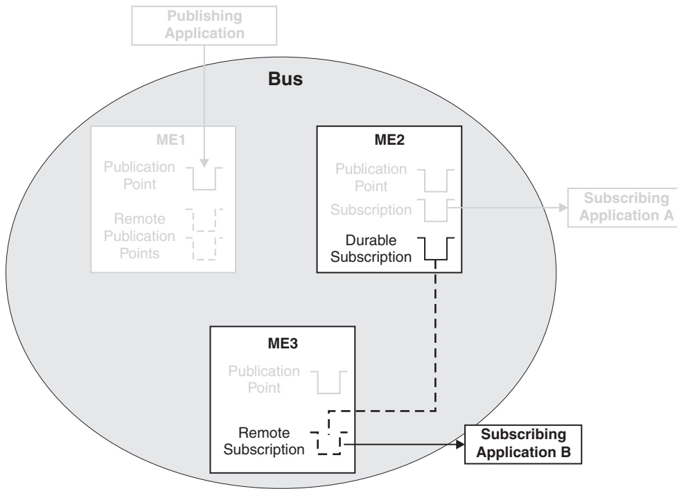
Figure 5. Publish/subscribe messaging by using a remote message point
