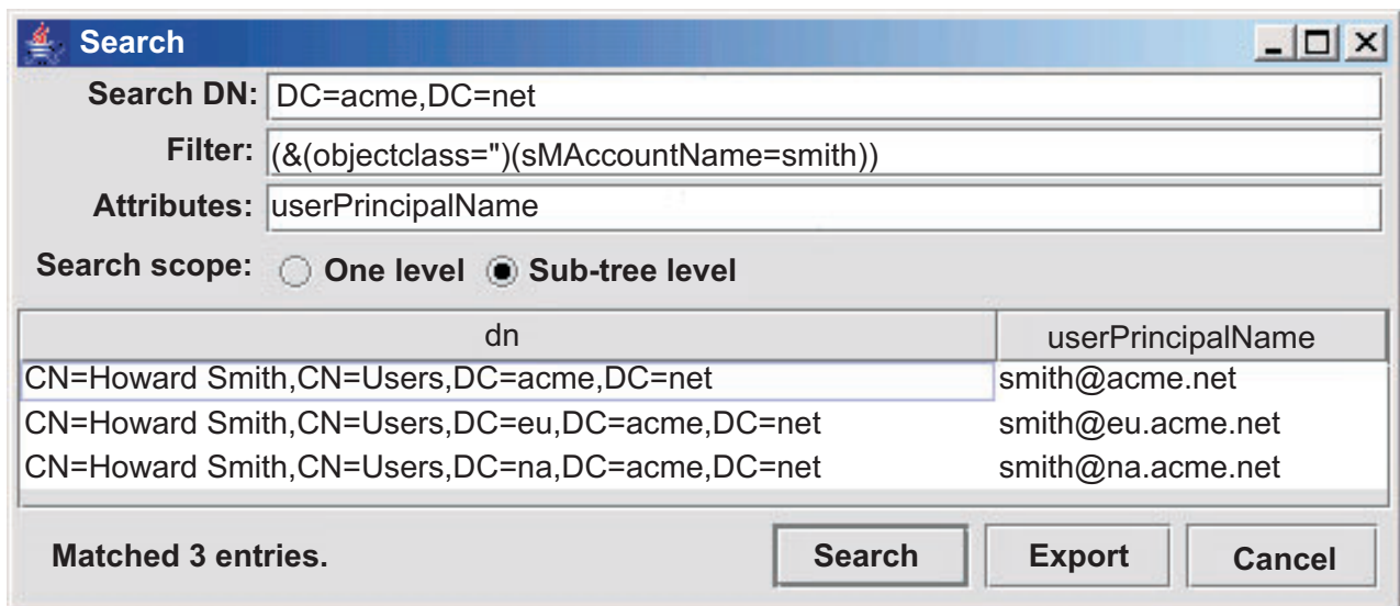
Figure 25. Forest search strategy.. Search illustration of a non-unique sMAccountName across the entire forest.
