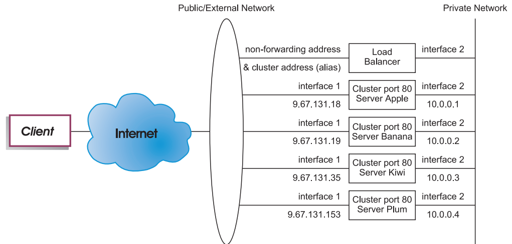
Figure 36. Example of a private network using Dispatcher
