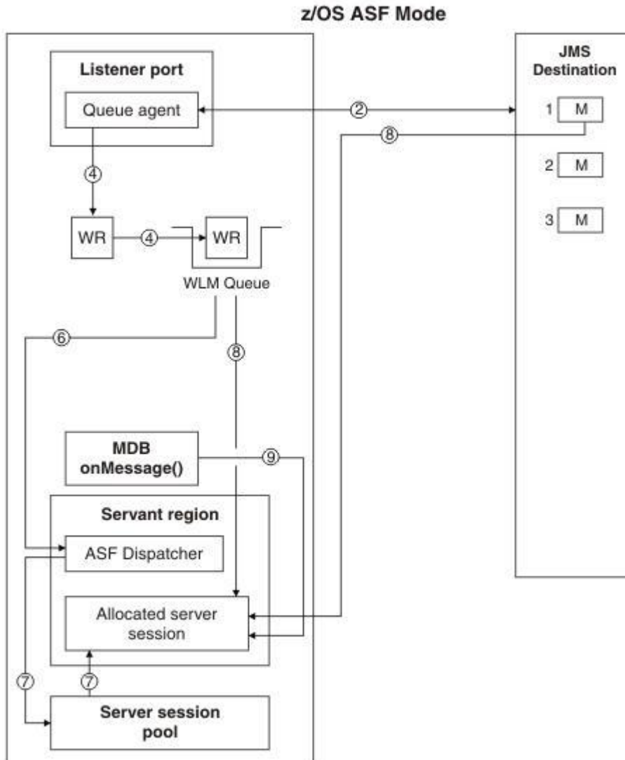
Figure 91. Message processing in ASF mode on z/OS systems
