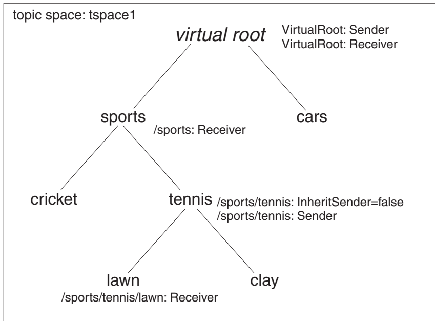
Figure 124. Example of a topic space with topic-level authorization
