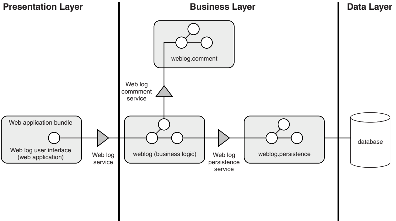
Figure 102. Example application for a weblog service
