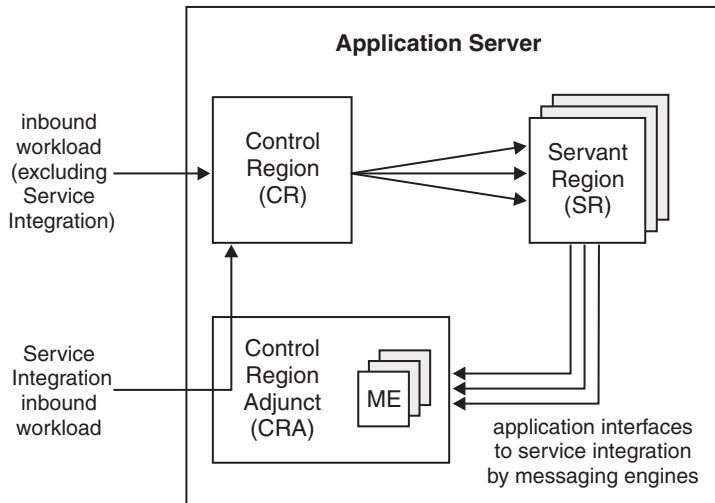
Figure 21. WebSphere Application Server running on z/OS has a multi-process structure
