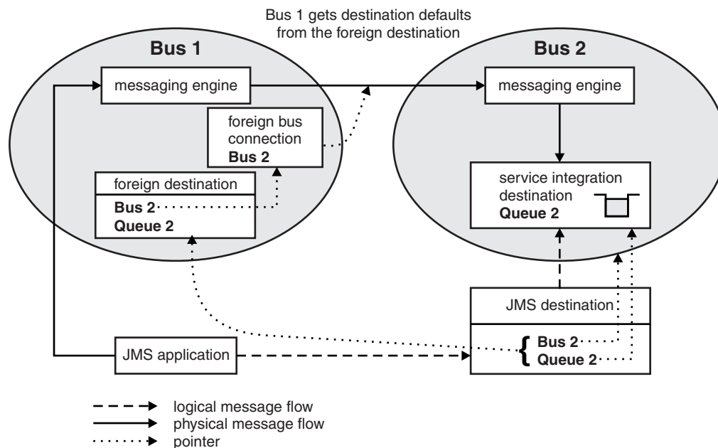
Figure 115. Point-to-point messaging between two buses with a foreign destination configured on the local bus
