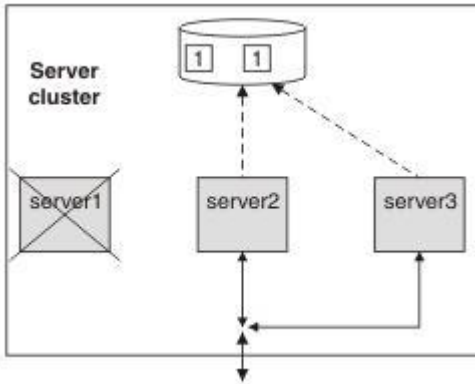
Figure 186. Server 1 fails. Servers 2 and 3 become blocked as a result
