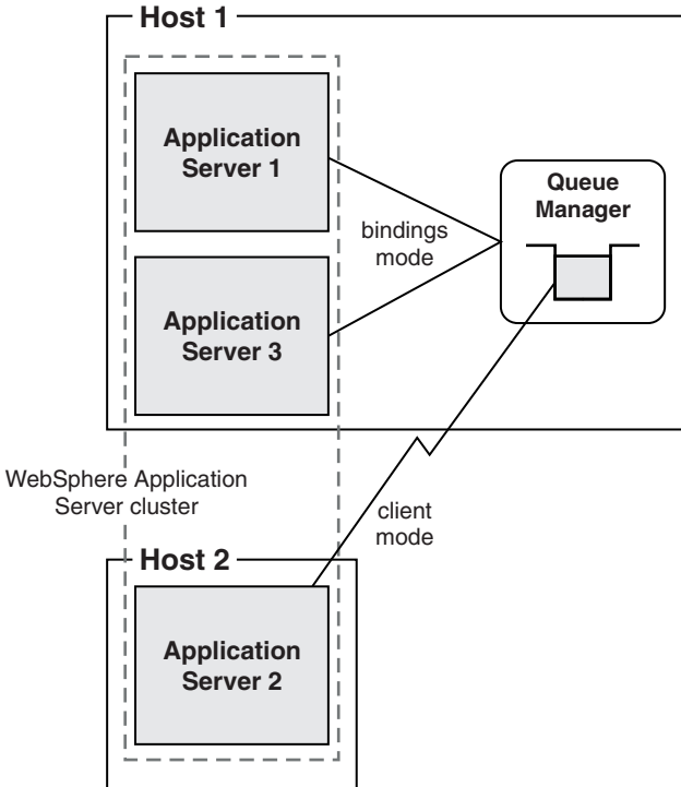
Figure 57. WebSphere Application Server clustering: bindings then client mode attachment to queue manager
