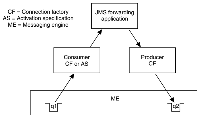
Figure 53. Forwarding messages
