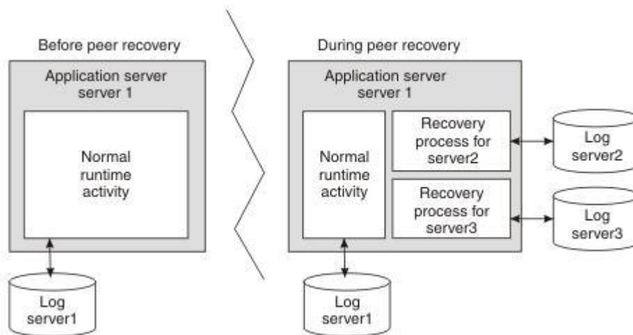
Figure 28. Peer recovery
