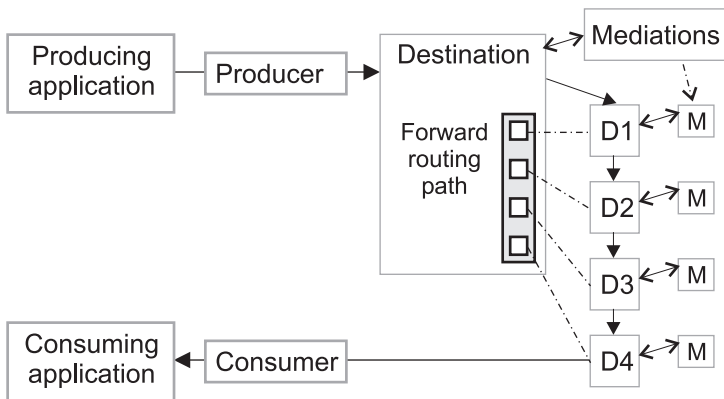
Figure 117. Routing paths
