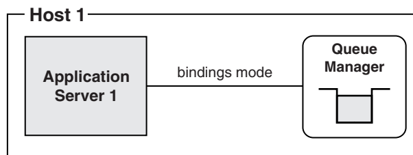
Figure 55. No clustering: bindings mode attachment to queue manager
