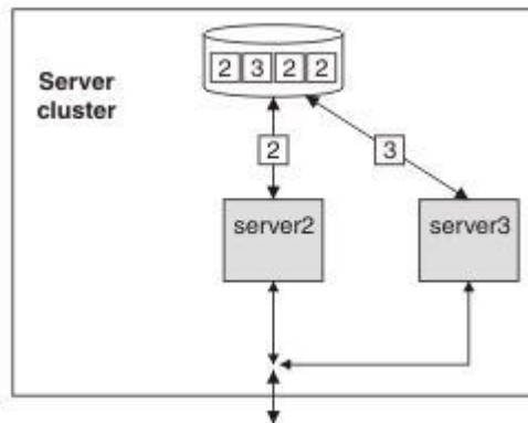
Figure 32. Server cluster stable again with just two servers: server 2 and server 3
