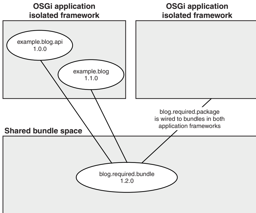
Figure 104. Application frameworks and the shared bundle space
