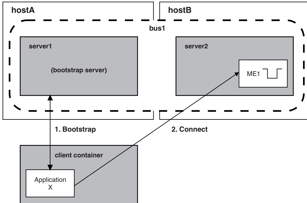
Figure 45. Connection to a messaging engine - Applications running outside an application server
