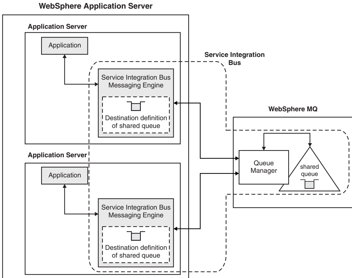
Figure 85. Two applications running within separate application servers connecting to a WebSphere MQ queue manager over a WebSphere MQ server connection
