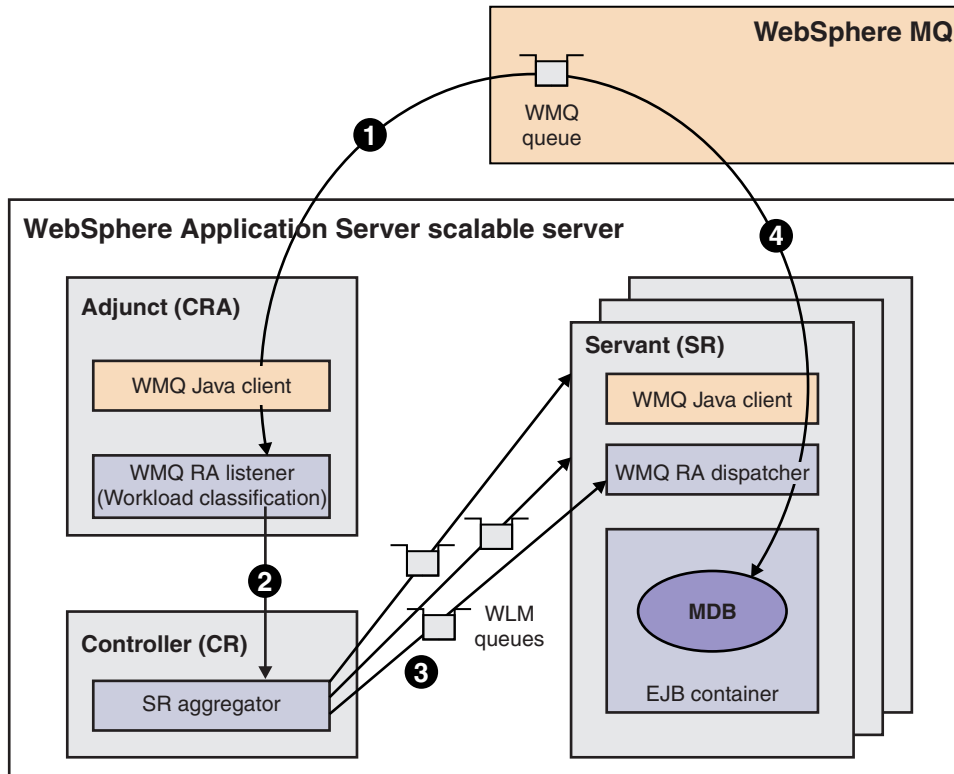
Figure 23. WebSphere MQ: message-driven bean processing
