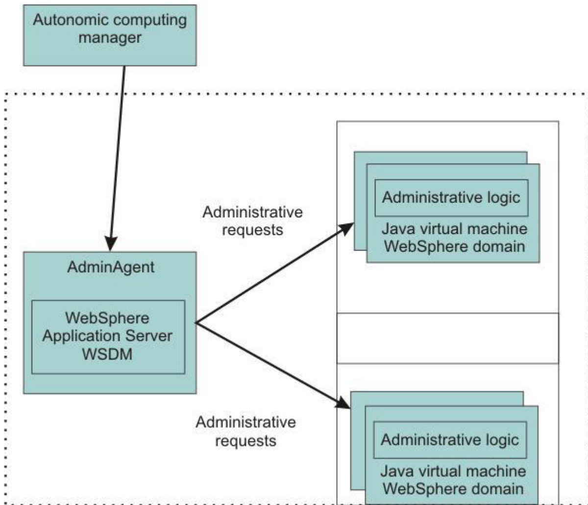
Figure 198. WSDM application in an AdminAgent environment
