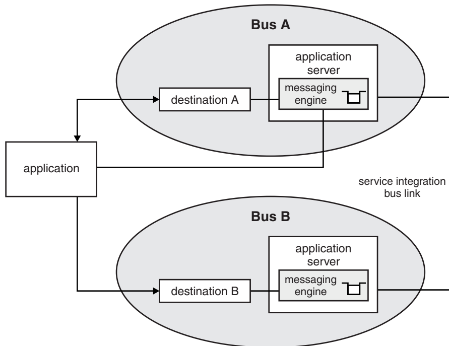
Figure 105. An application that is connected to bus A
