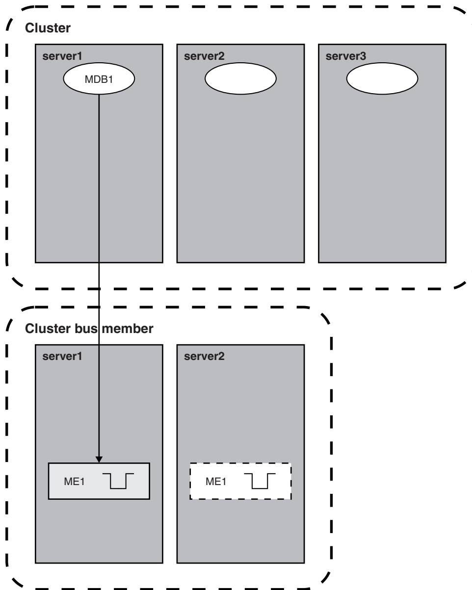
Figure 51. One server receiving messages from messaging engine in a cluster bus member
