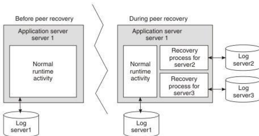
Figure 184. Peer recovery
