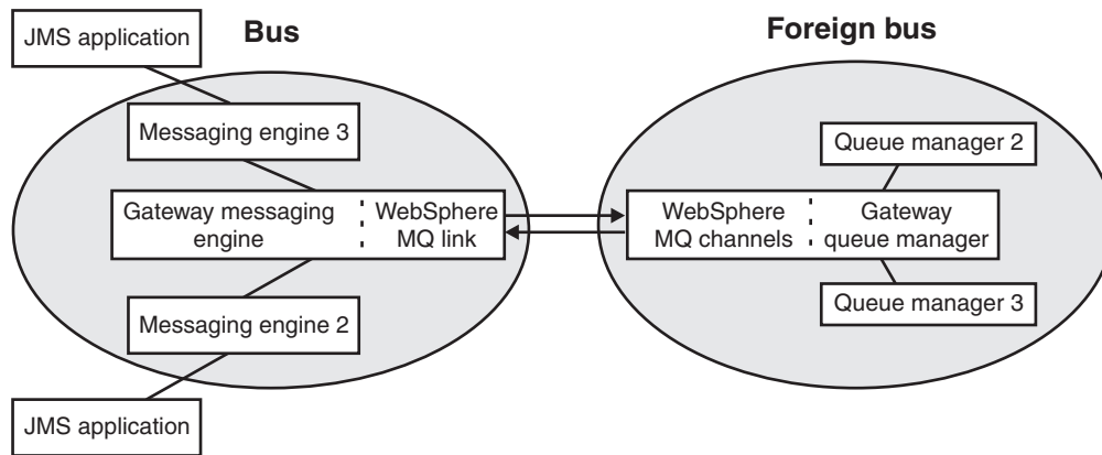
Figure 79. Exchanging messages between messaging engines on a bus that has a WebSphere MQ link that is connected to a gateway queue manager on a foreign bus.
