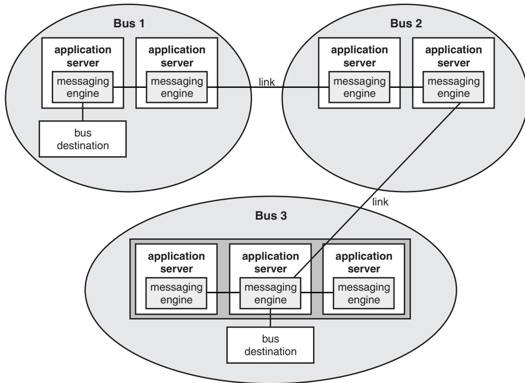
Figure 170. Linking service integration buses.
