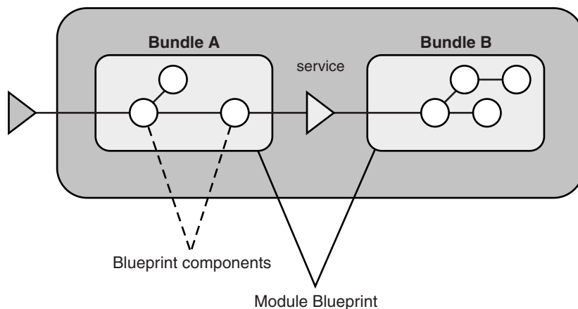
Figure 101. OSGi application with two bundles
