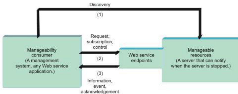
Figure 195. Relationship between the different parts of WSDM
