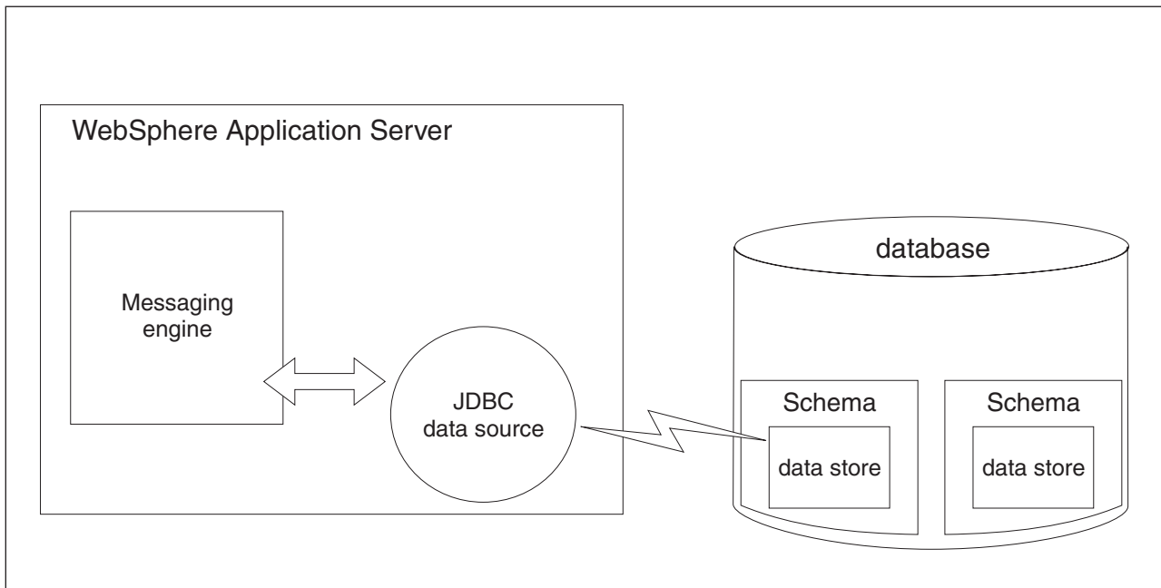
Figure 122. The relationship between a messaging engine and its data store.
