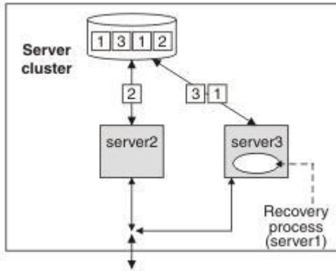
Figure 14. Peer recovery process started in server 3
