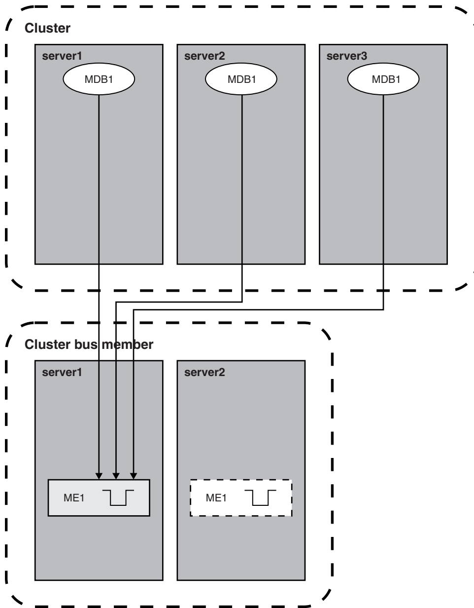
Figure 50. All servers in cluster receive messages from messaging engines in a cluster bus member
