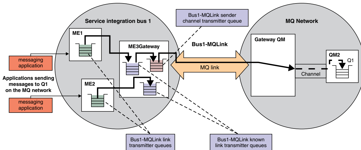
Figure 172. Message flow between a service integration bus and a WebSphere MQ network
