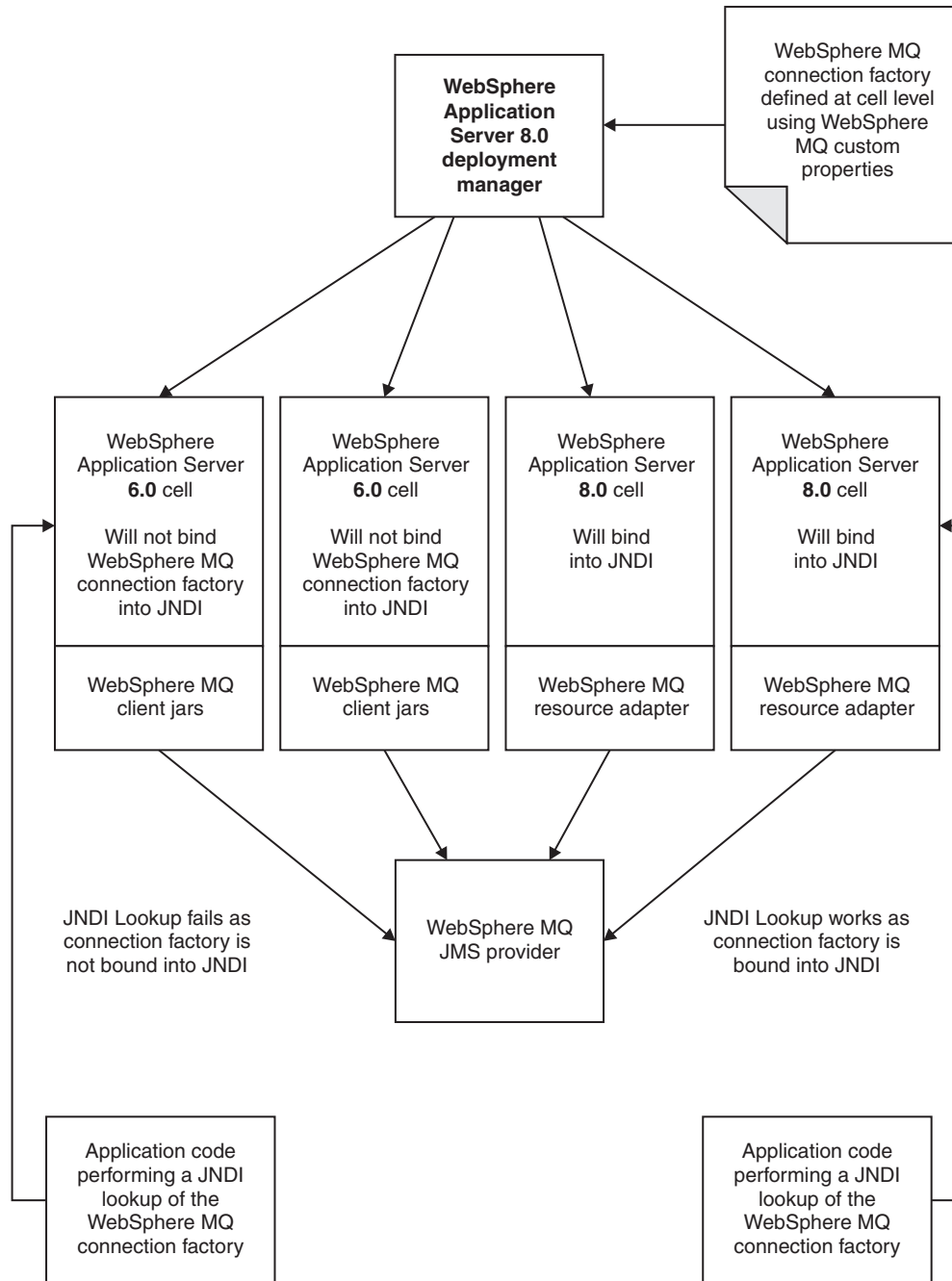
Figure 63. Mixed node scenario
