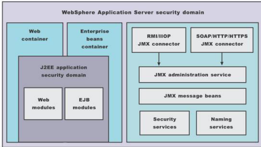
WebSphere Application Server process
