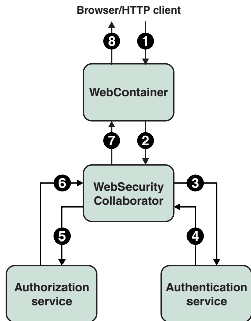
Figure 39. Typical security flow for web resources
