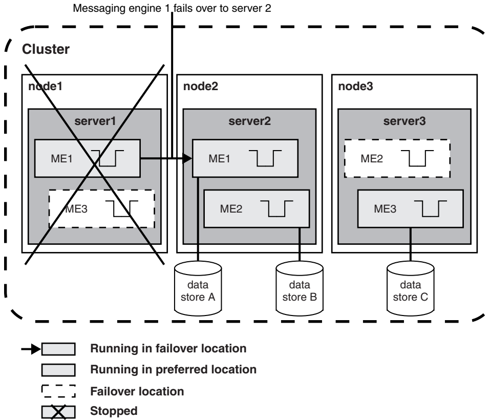
Figure 151. High availability with workload sharing or scalability configuration after server1 fails
