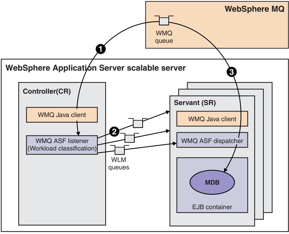
Figure 25. WebSphere MQ ASF - listening in the controller
