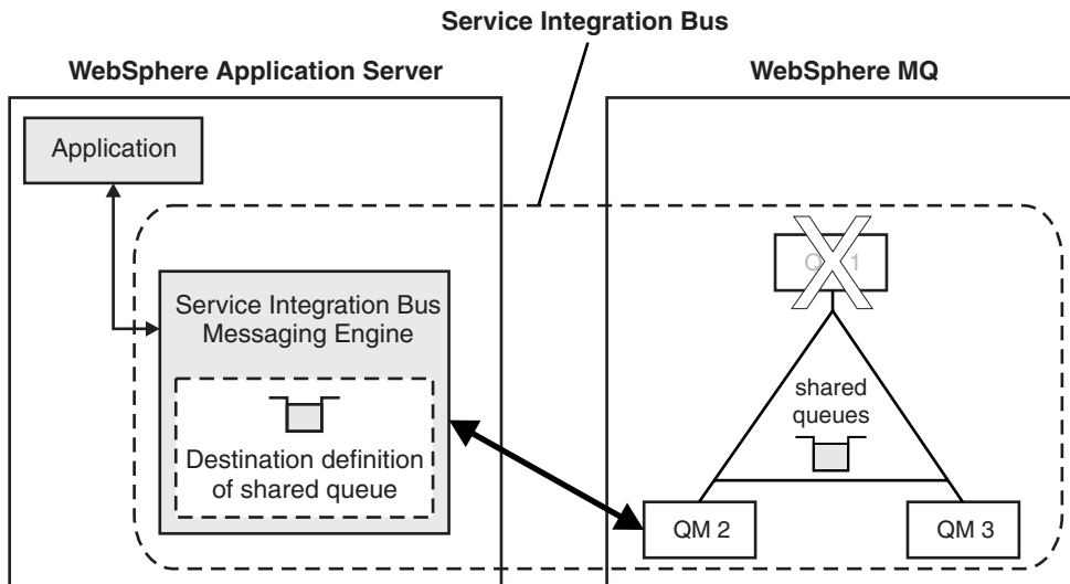
Figure 87. A messaging engine connecting to a second queue manager to access a queue sharing group, after the original queue manger it was using failed
