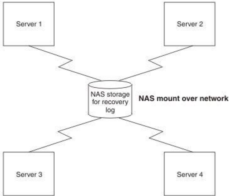
Figure 189. Recovery logs on NAS storage are available to all servers
