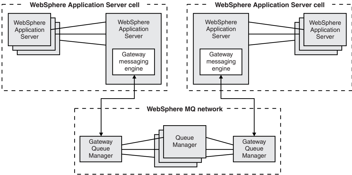
Figure 72. Geographically separated application servers connected to the same WebSphere MQ network
