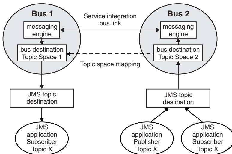
Figure 174. Publish/subscribe messaging across Bus 1 and Bus 2
