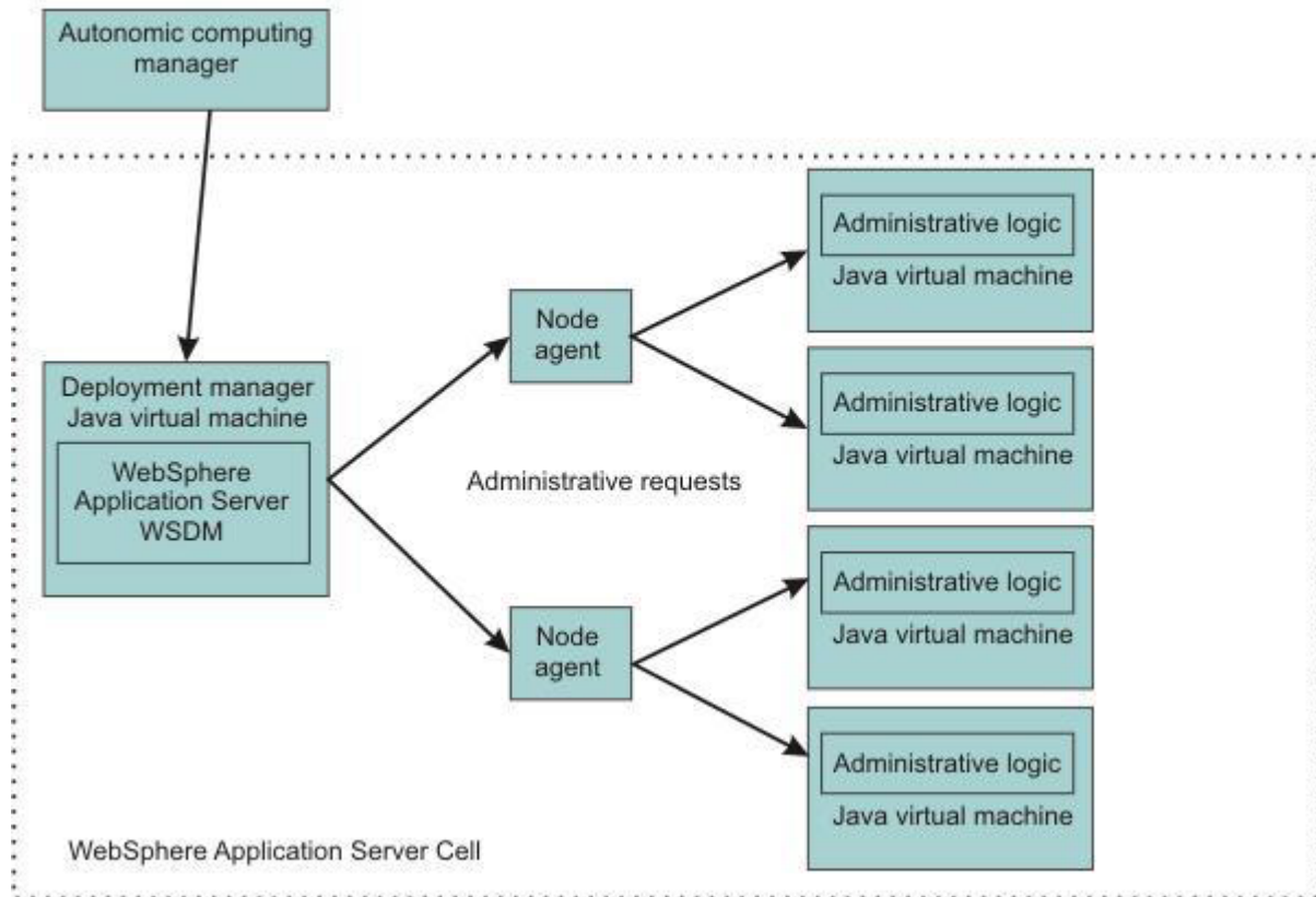
Figure 197. WSDM application in a WebSphere Application Server, Network Deployment cell
