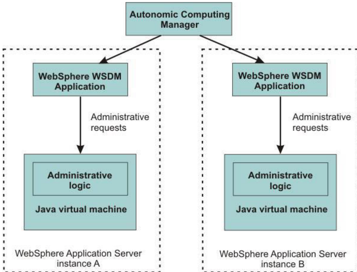
Figure 196. WSDM application in a stand-alone server instance
