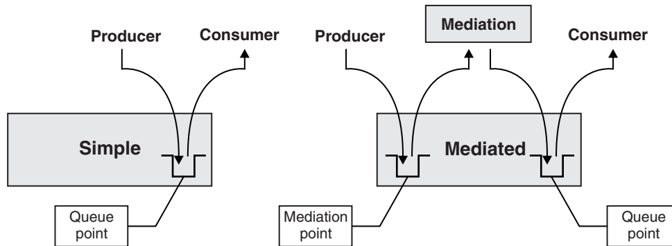
Figure 88. Queue-type destinations assigned to a service integration bus member. Queue points and mediation points are queues of service integration messages held in service integration
