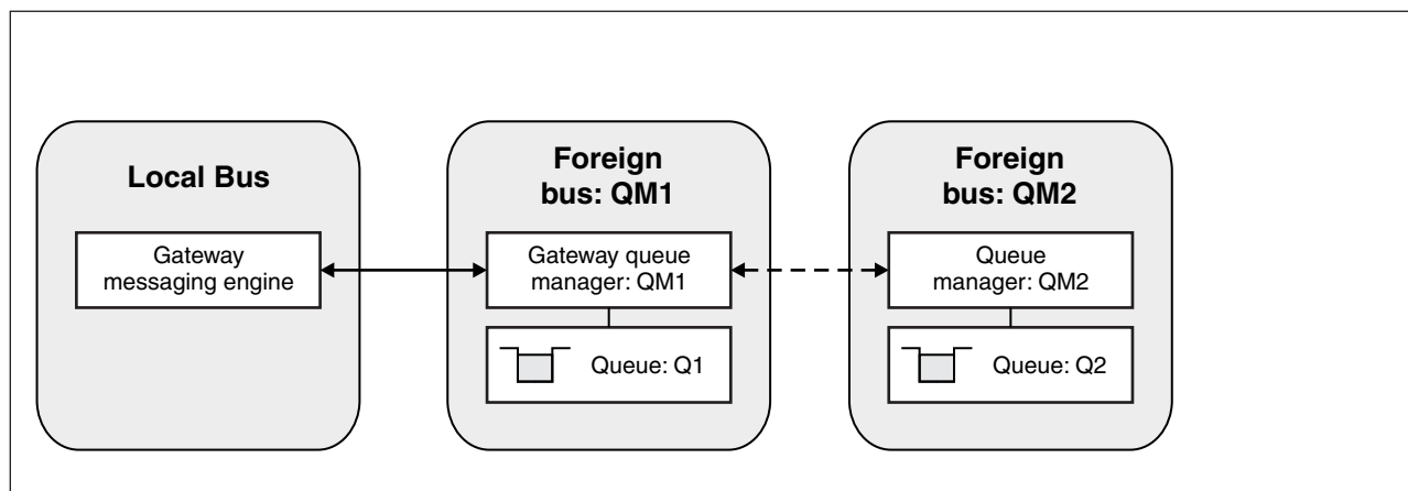
Figure 67. Addressing a WebSphere MQ queue in an indirectly connected foreign bus
