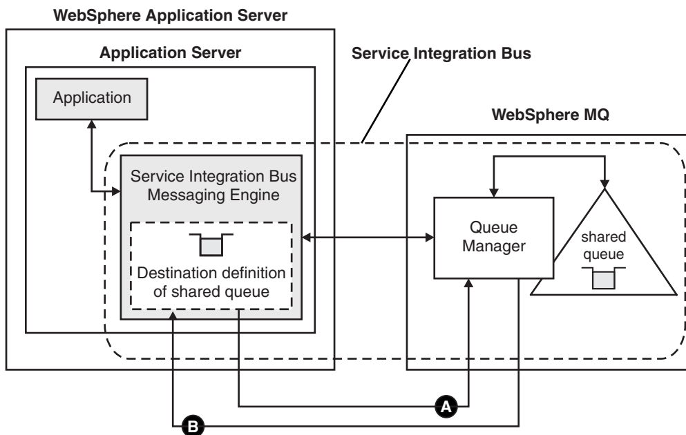
Figure 84. Single application running within WebSphere Application Server and connecting to WebSphere MQ using a WebSphere MQ server connection.
