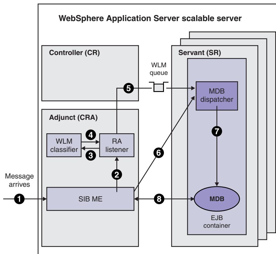
Figure 22. Service integration bus: message-driven bean processing
