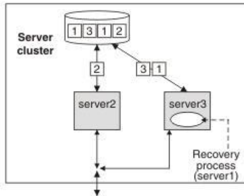
Figure 31. Peer recovery process started in server 3
