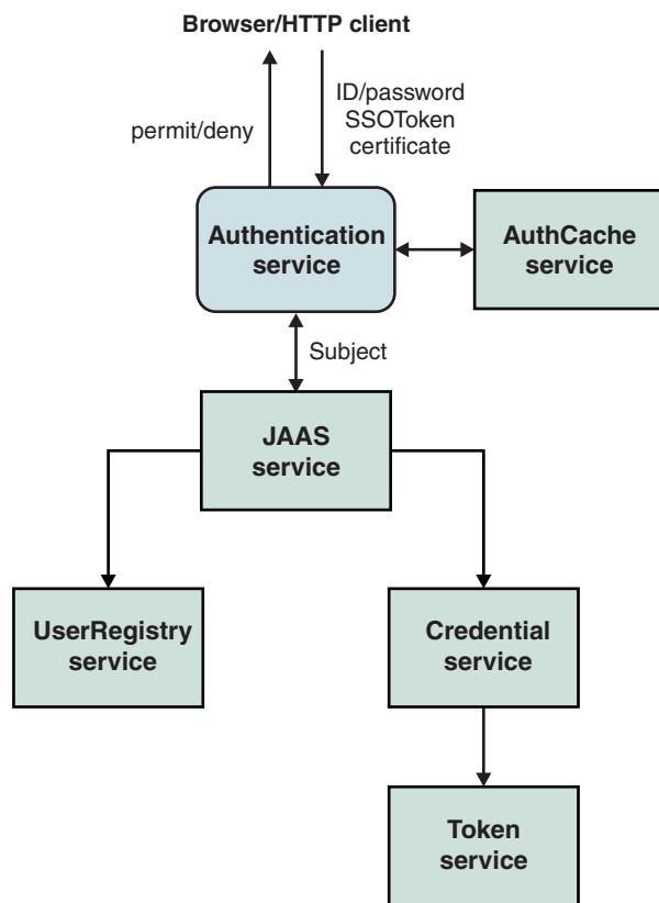
Figure 40. Overview of authentication process
