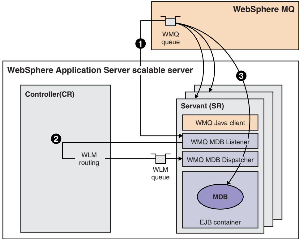
Figure 26. WebSphere MQ ASF - listening in the servant
