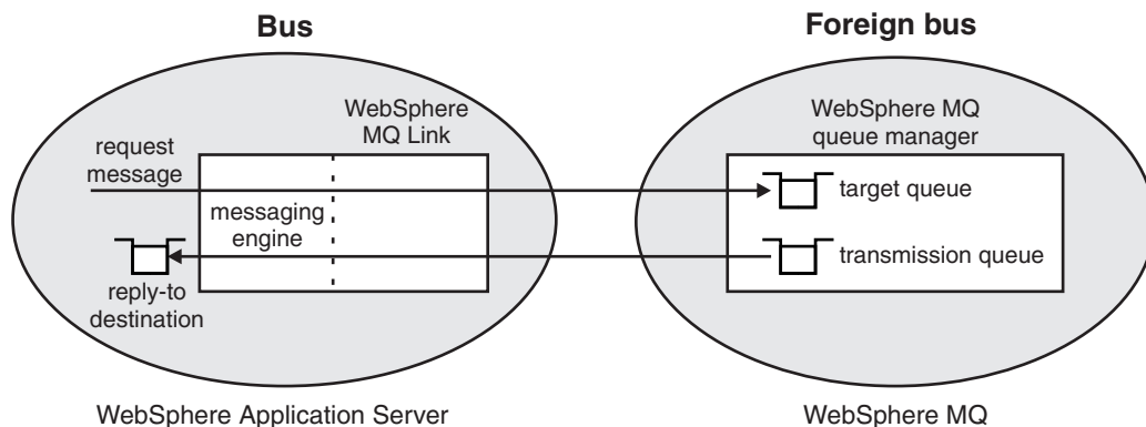
Figure 77. Paths taken by a message and response exchanged between a messaging engine on a bus and a queue manager in WebSphere MQ
