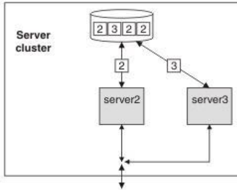
Figure 188. Server cluster stable again with just two servers: server 2 and server 3
