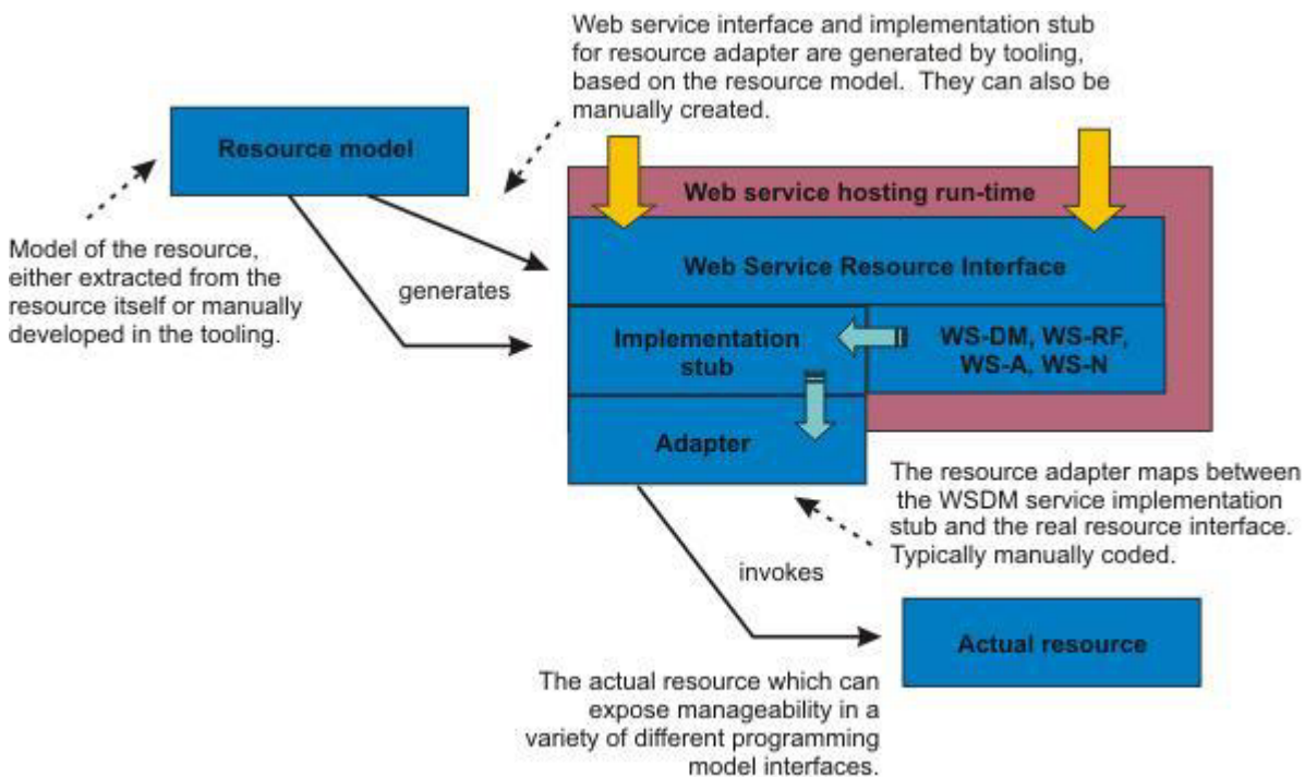
Figure 194. Generic WSDM Concept
