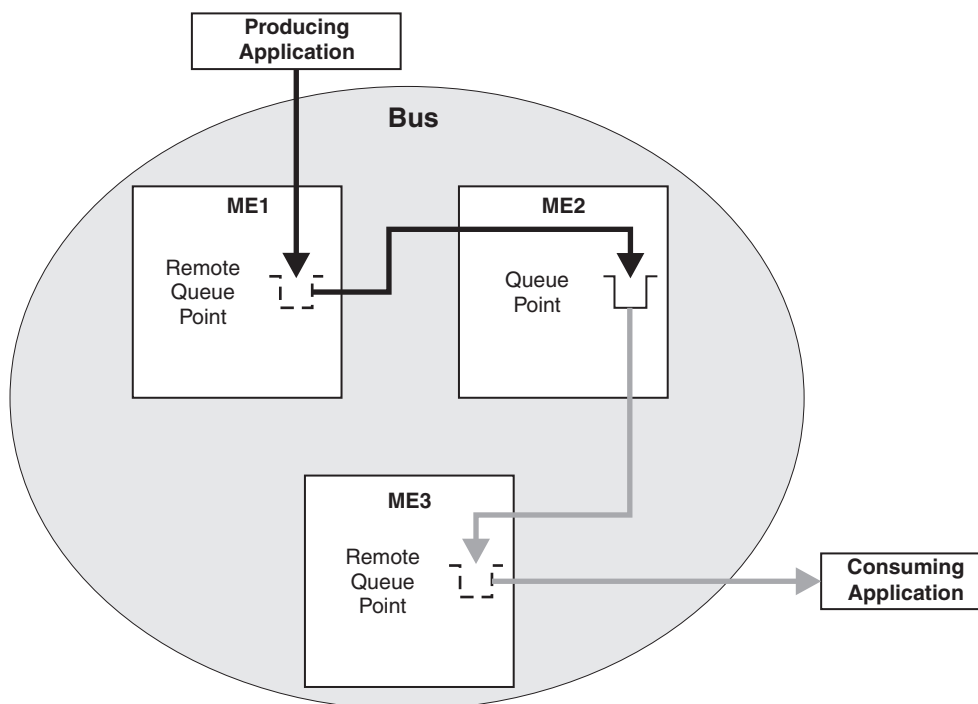
Figure 108. Point-to-point message production and consumption by using remote queue points.
