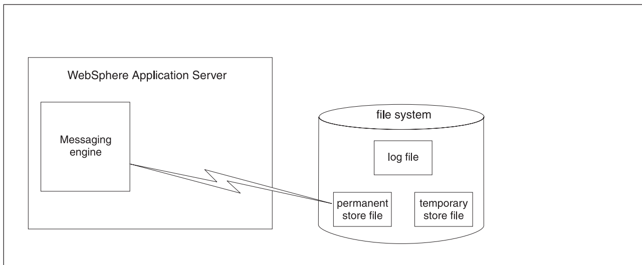
Figure 121. The relationship between a messaging engine and its file store
