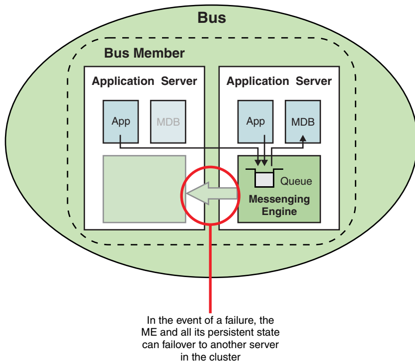
Figure 166. Application server cluster with single messaging engine bus configuration
