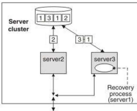
Figure 187. Peer recovery process started in server 3
