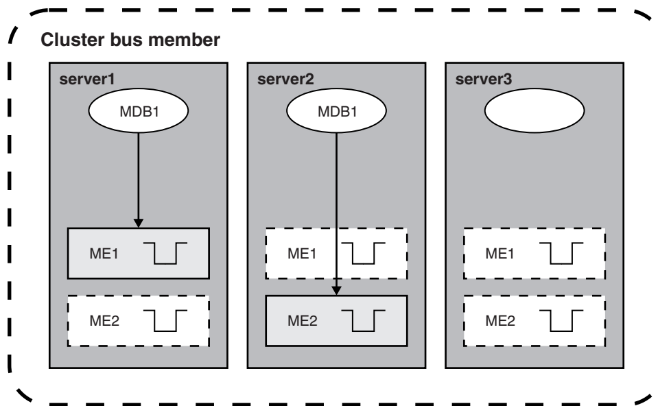
Figure 47. MDB is driven by servers in the cluster bus member that hosts a started messaging engine (setup 1)
