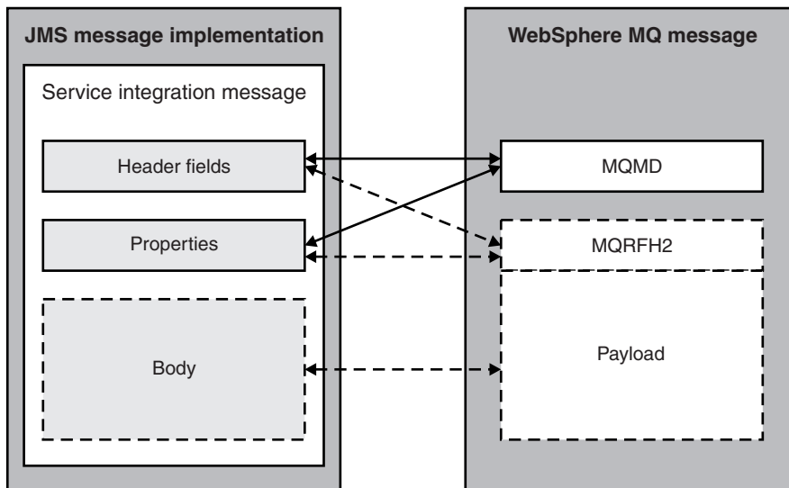
Figure 66. Message conversion to and from WebSphere MQ format
