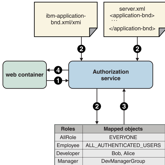
Figure 41. Overview of authorization process
