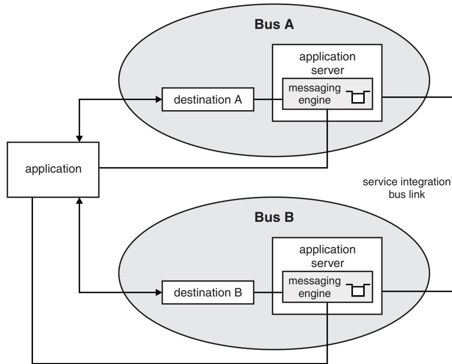
Figure 106. An application that is connected to bus A and bus B
