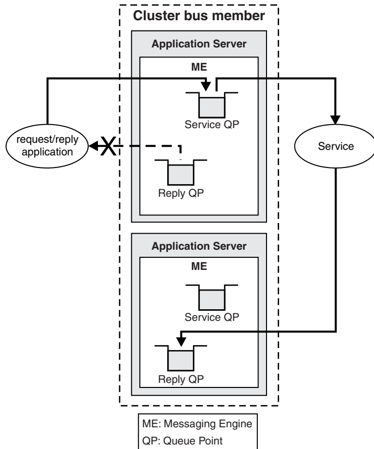
Figure 133. A service integration bus queue destination that is defined to a cluster bus member with two messaging engines
