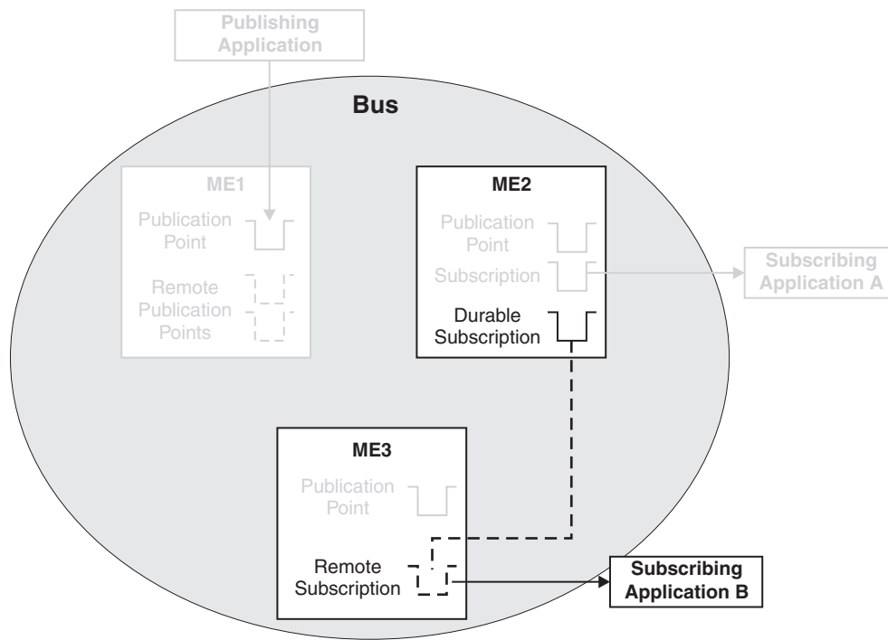
Figure 120. Publish/subscribe messaging using a remote subscription
