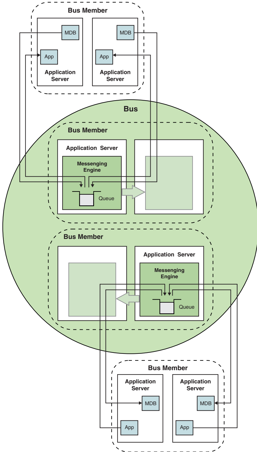
Figure 168. Multiple bus member bus configuration
