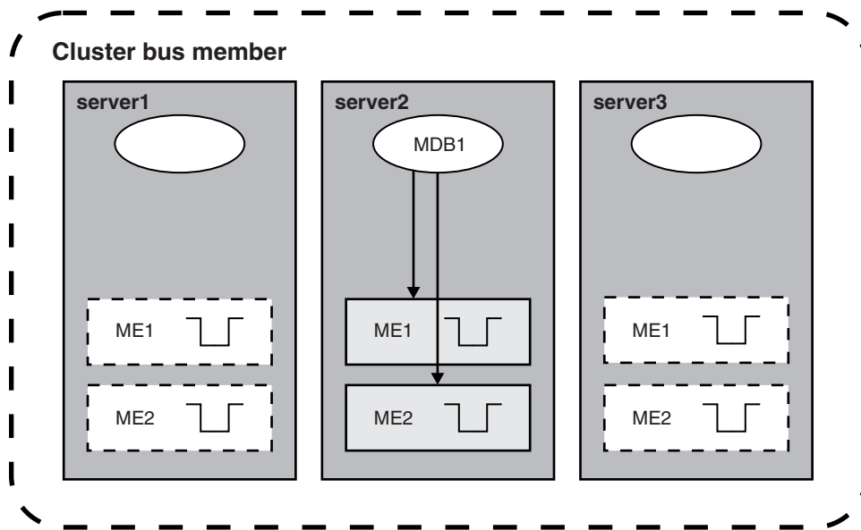
Figure 48. MDB is driven by servers in the cluster bus member that hosts a started messaging engine (setup 2)
