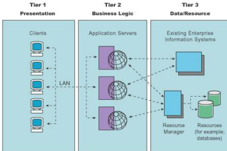
Figure 202. Three tier architecture
