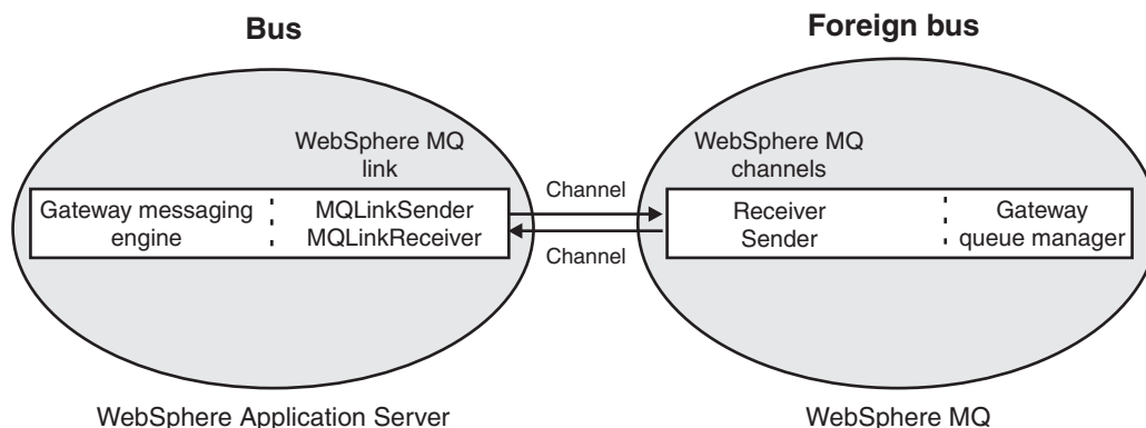
Figure 78. Exchanging messages between WebSphere MQ link sender and receiver channels, and a gateway queue manager with receiver and sender channels.
