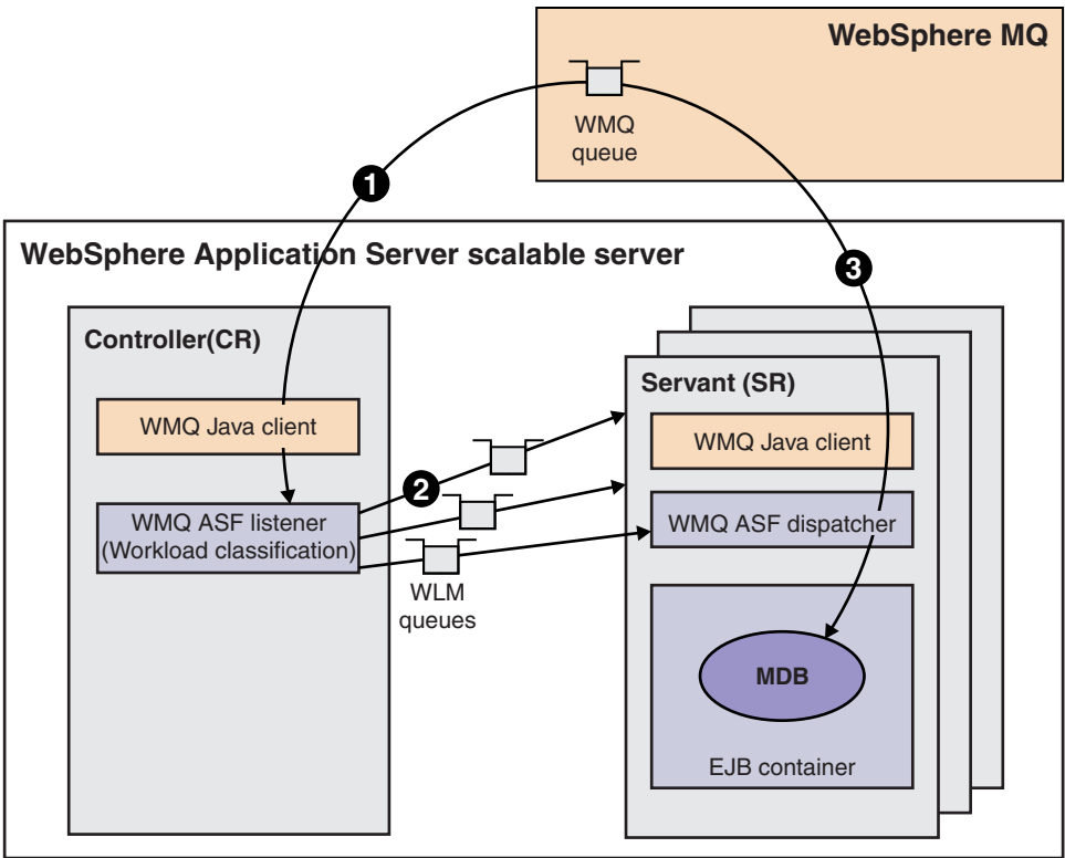
Figure 27. Controlling processing of the WMQ queue and WLM queues
