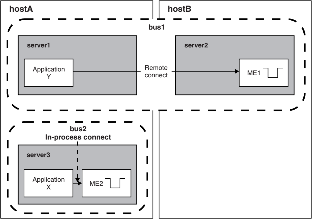
Figure 44. Default connection to a messaging engine - Applications running in an application server
