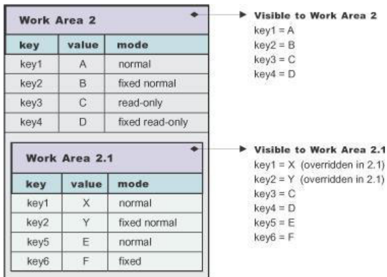
Figure 192. Redefining existing properties in nested work areas
