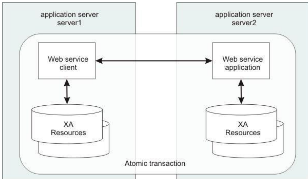
Figure 201. Transaction context shared between two application servers
