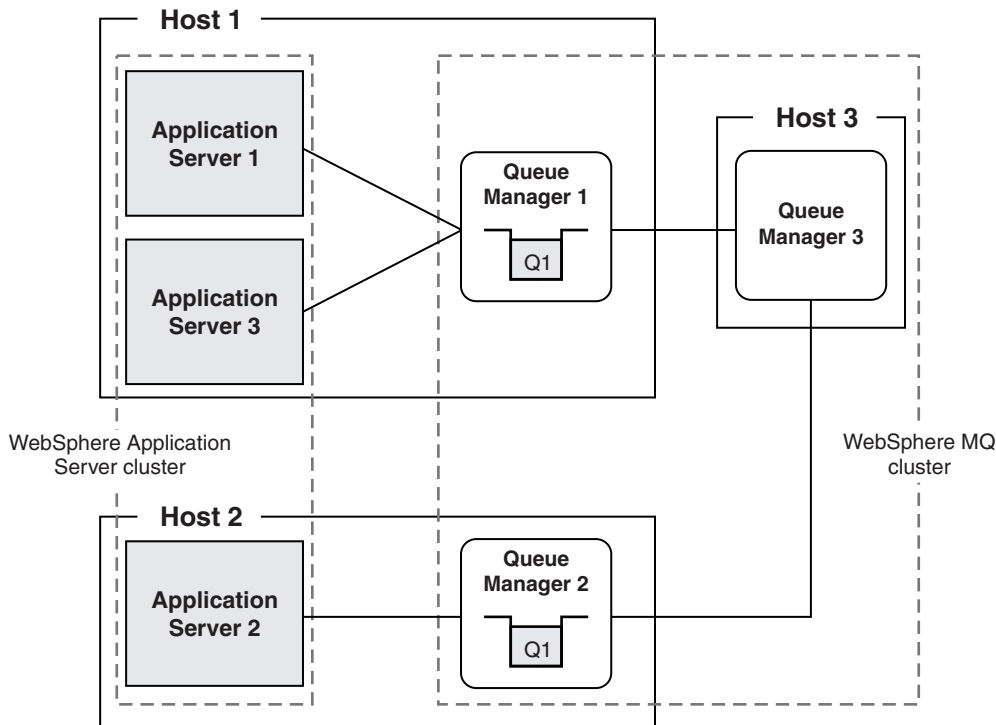
Figure 59. WebSphere Application Server clustering: bindings mode attachment to queue managers
