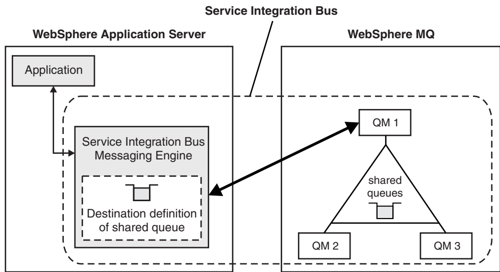
Figure 86. A messaging engine connecting to a queue manager to access a queue sharing group, using a WebSphere MQ server connection
