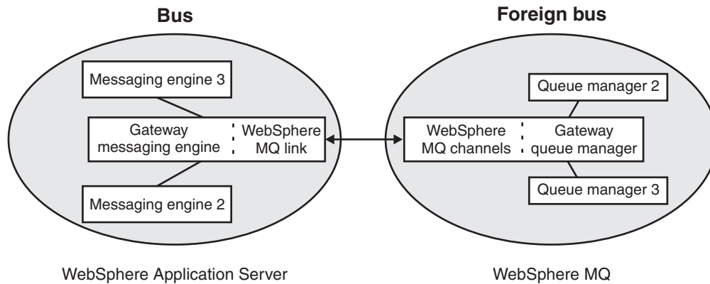
Figure 75. Exchanging messages between messaging engines on a bus and queue managers connected to the gateway queue manager on a foreign bus.
