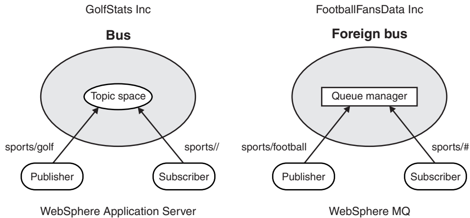
Figure 80. Two separate businesses that publish information to their respective audiences.
