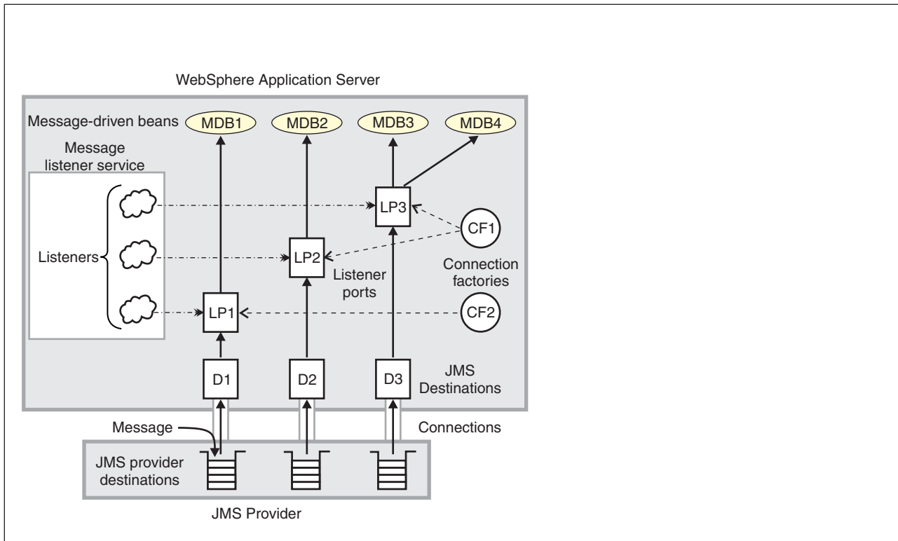
Figure 20. The main components for message-driven beans
