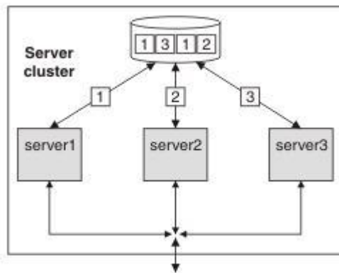
Figure 185. Server cluster up and running, just before server failure
