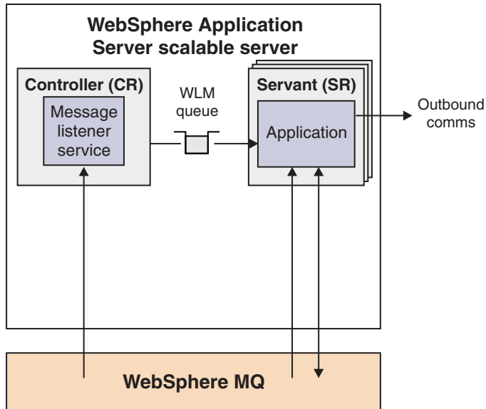
Figure 96. WebSphere MQ connections - Message Listener Service (ASF)
