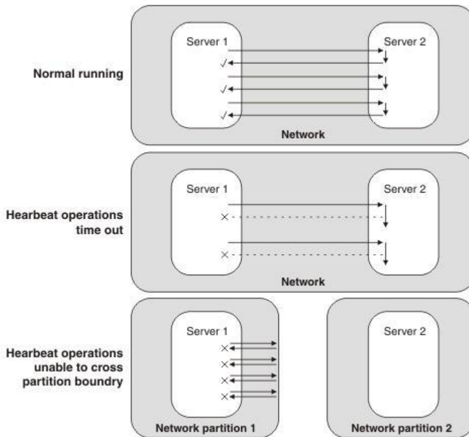
Figure 34. Heartbeats in a system running normally, compared to heartbeats after the apparent server failures of system overloading and network partitioning
