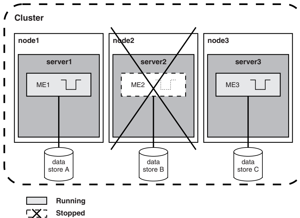
Figure 149. Workload sharing or scalability configuration after server1 recovers and server2 fails
