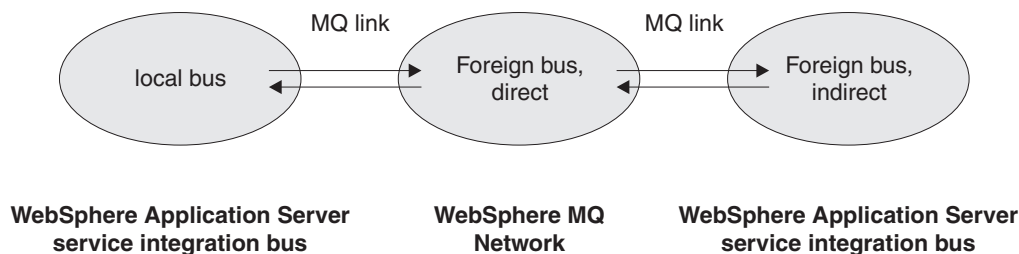
Figure 82. Exchanging messages between two application servers through an intermediate WebSphere MQ network.
