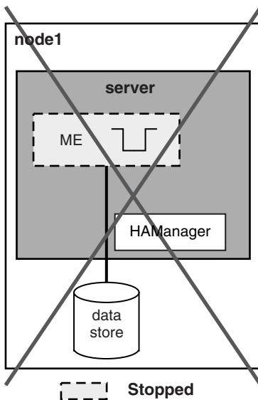
Figure 143. Simple configuration after the server fails
