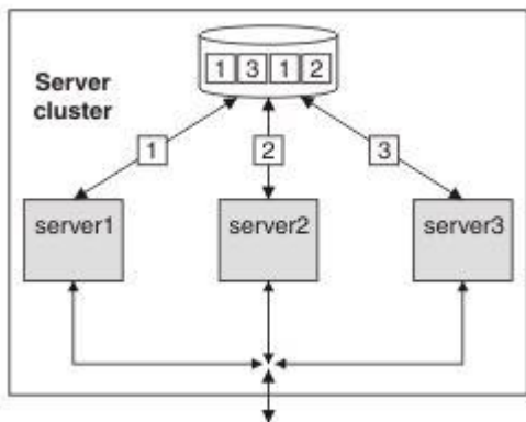
Figure 29. Server cluster up and running, just before server failure
