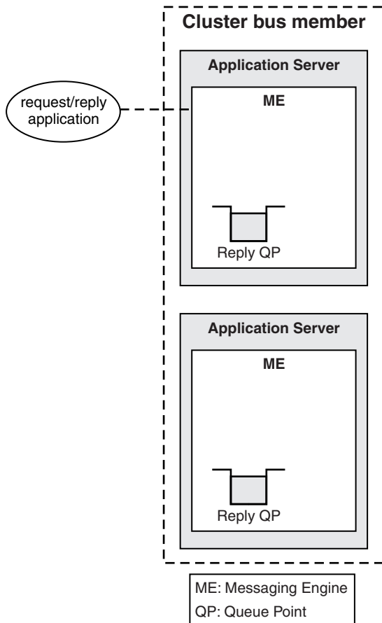
Figure 136. A requesting JMS application connects to one of the messaging engines in the cluster bus member
