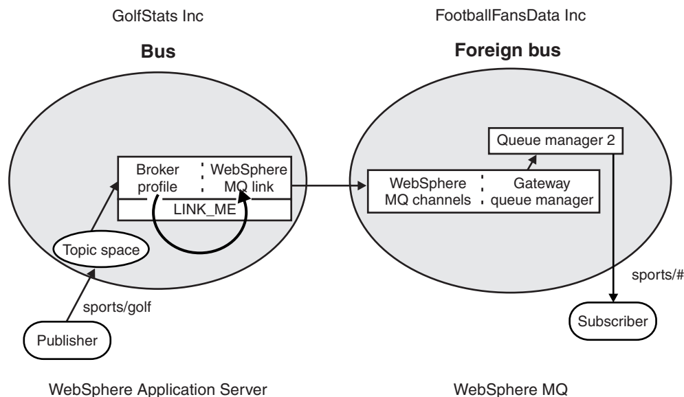
Figure 81. Two linked businesses with one of them publishing to the other.
