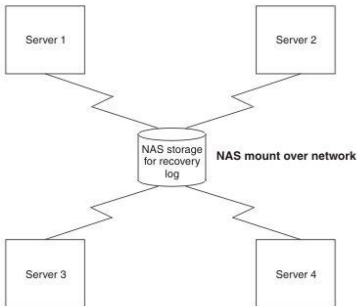
Figure 33. Recovery logs on NAS storage are available to all servers
