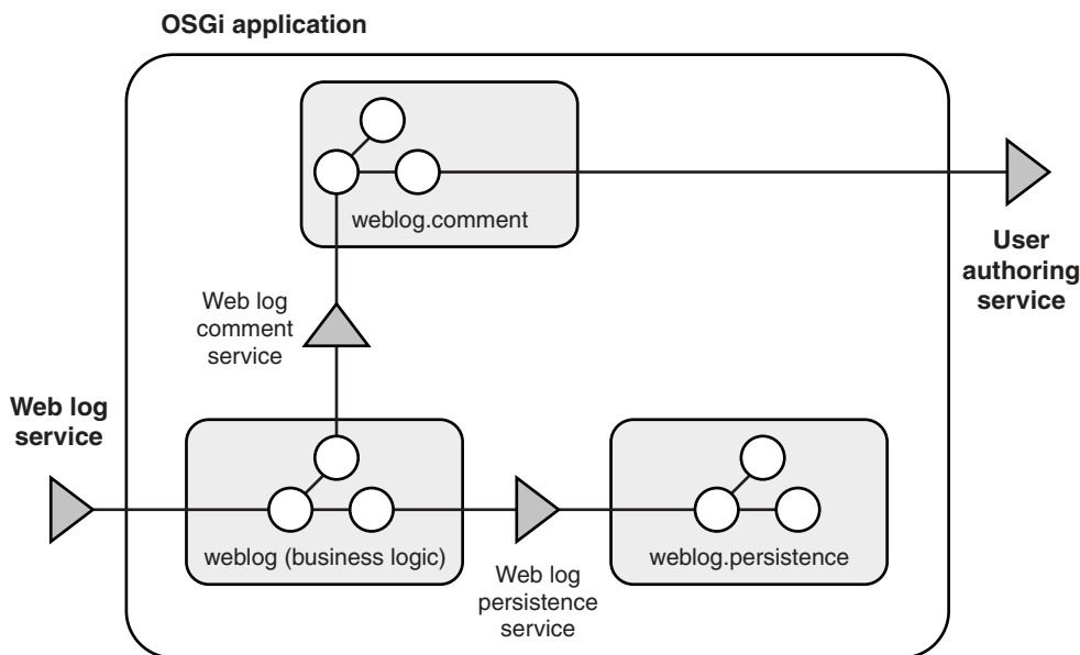
Figure 103. Bundles and services in an example application for a weblog service
