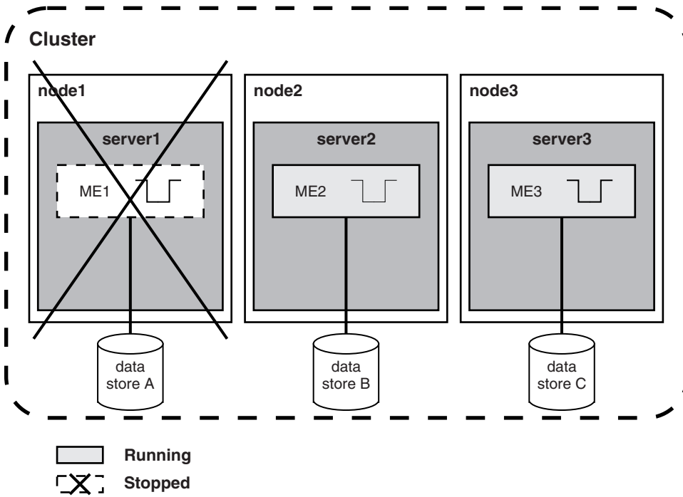
Figure 148. Workload sharing or scalability configuration after server1 fails
