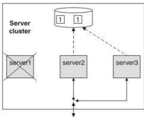
Figure 30. Server 1 fails. Servers 2 and 3 become blocked as a result
