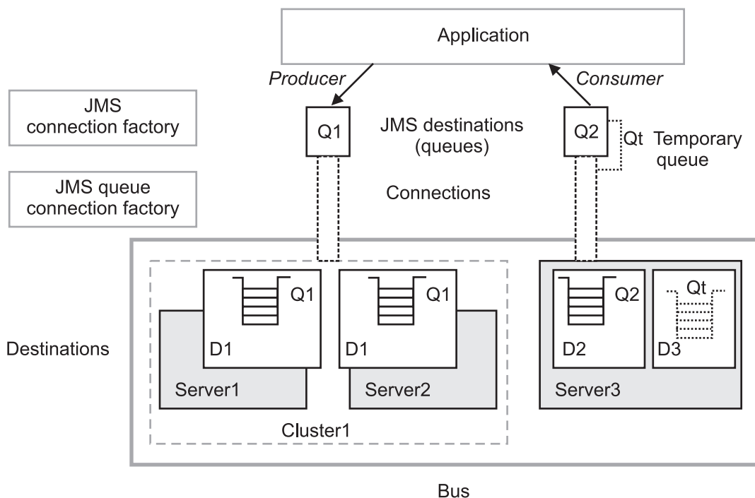
Figure 42. JMS point-to-point messaging and the default messaging provider
