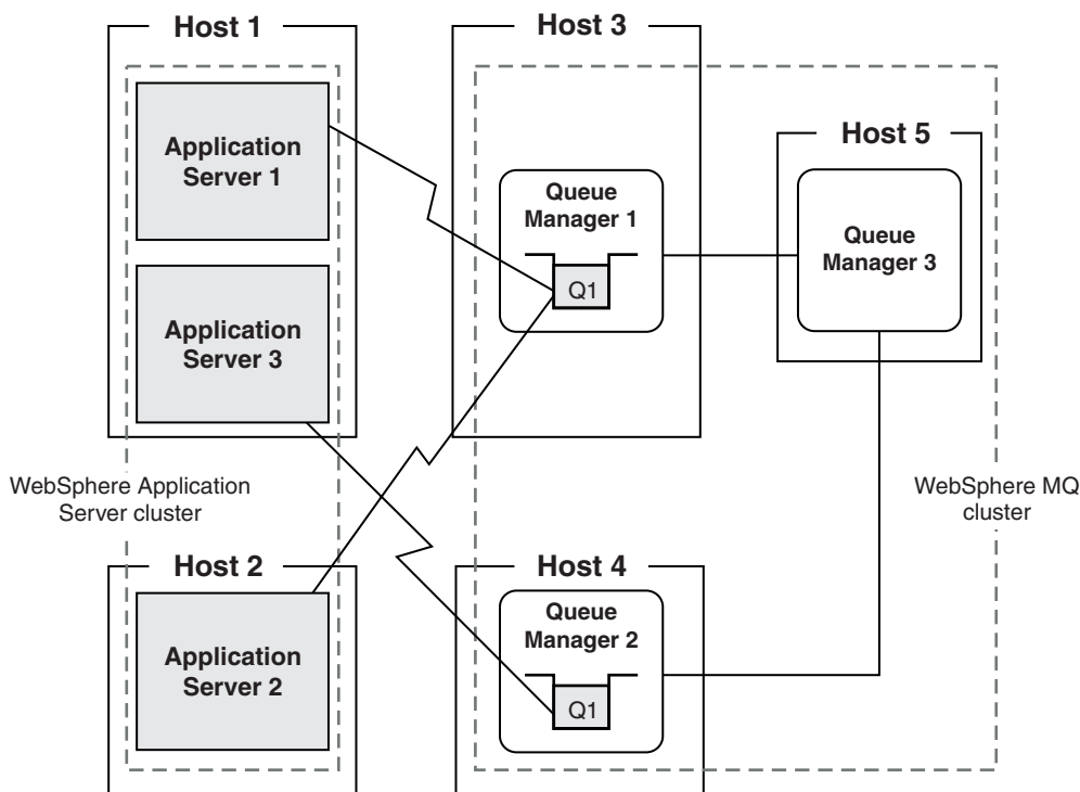
Figure 58. WebSphere Application Server clustering: client mode attachment to queue managers
