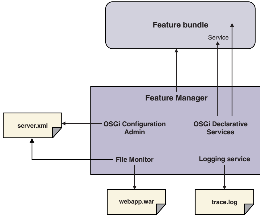
Figure 36. Liberty profile kernel
