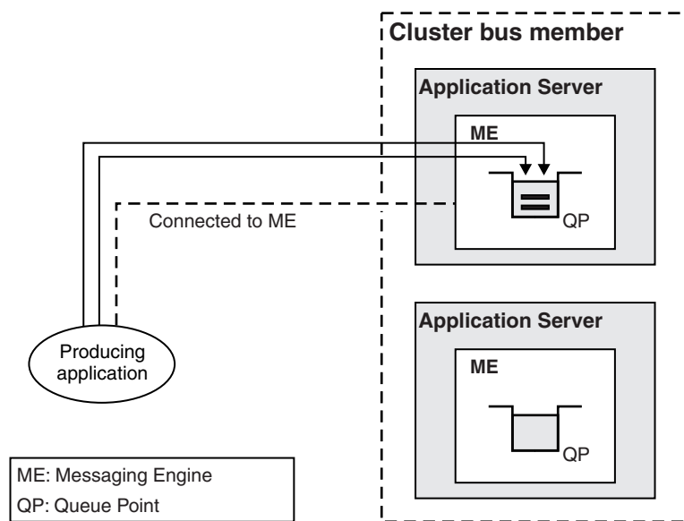
Figure 125. Default behavior: messages are sent to the local queue point
