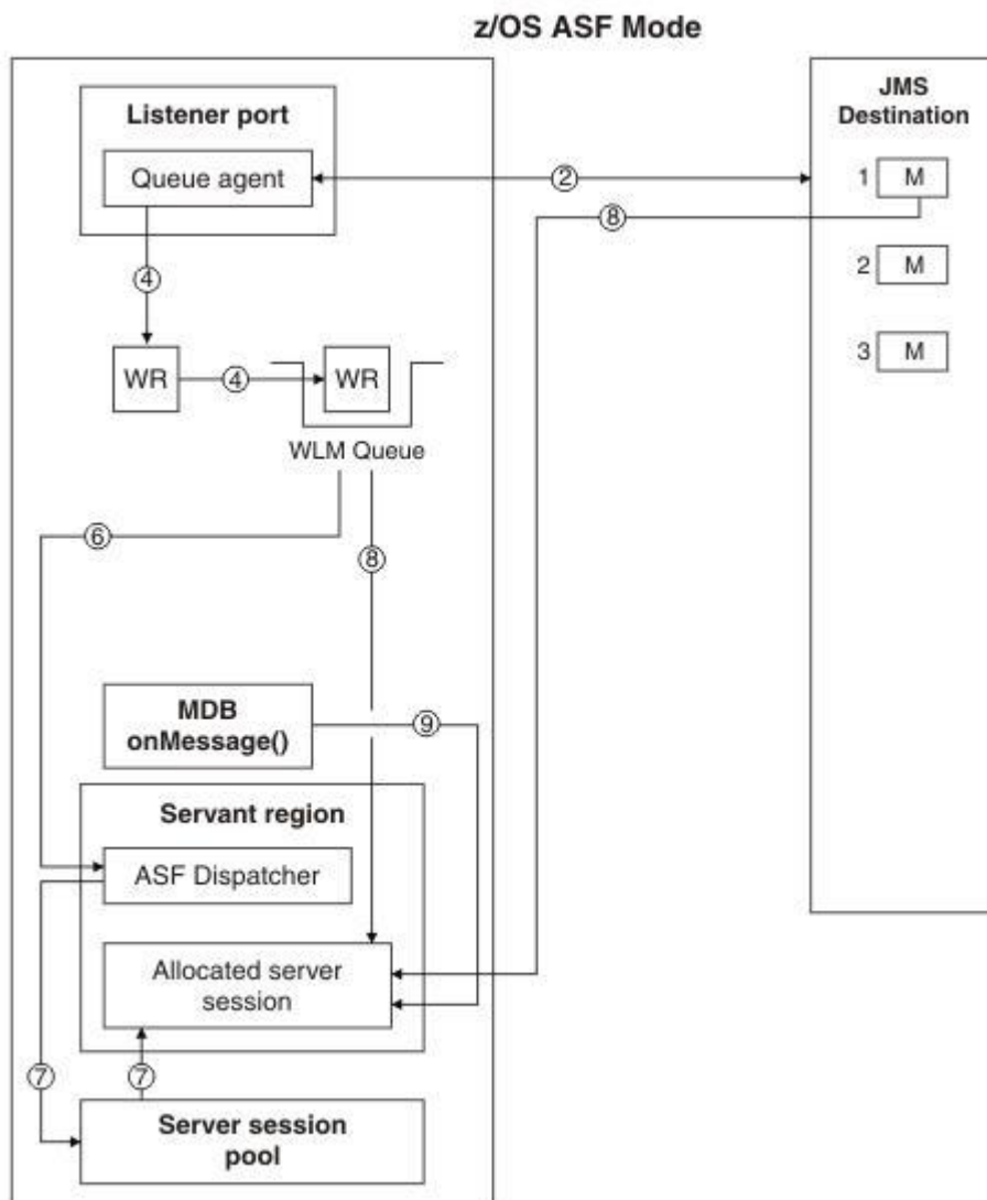
Figure 19. Message processing in ASF mode on z/OS systems
