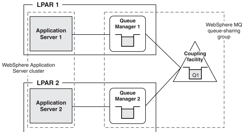
Figure 60. WebSphere Application Server with bindings mode connection to WebSphere MQ for z/OS
