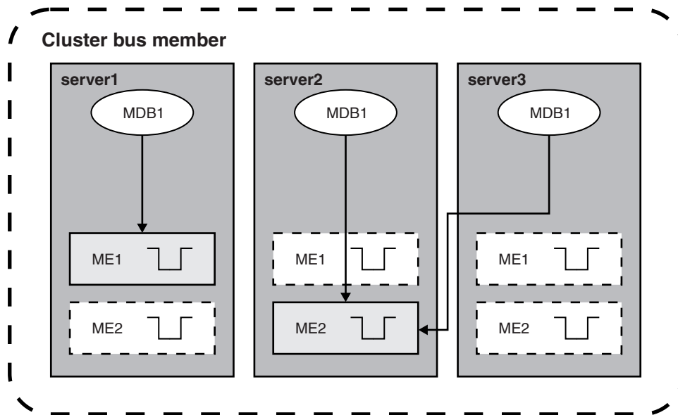
Figure 49. Servers in a cluster bus member receive messages from a message-driven bean
