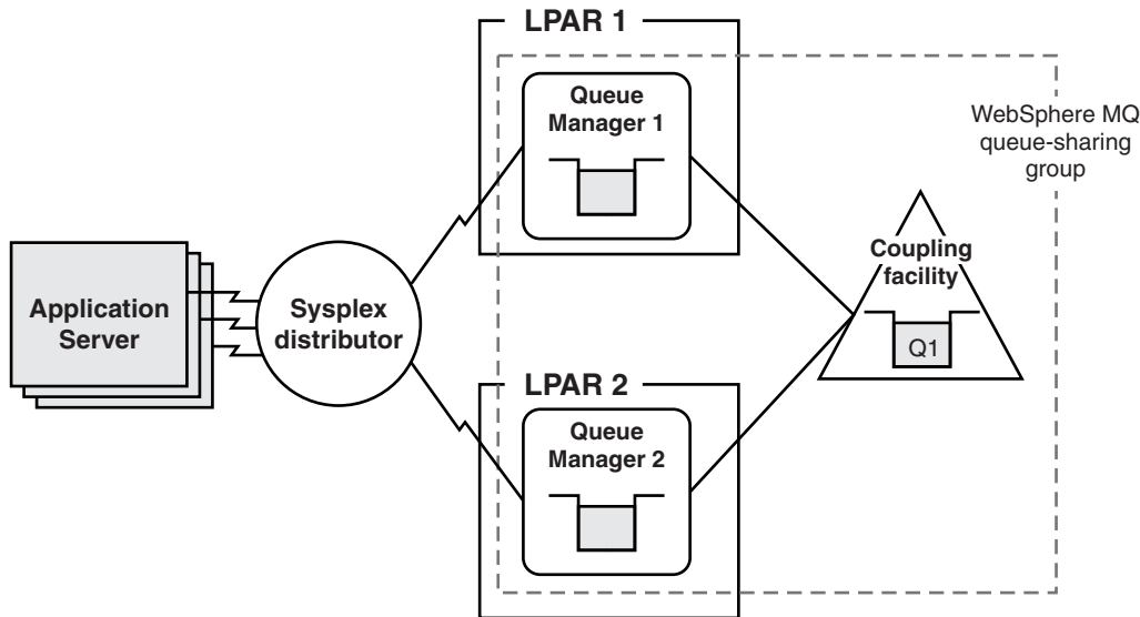
Figure 61. WebSphere Application Server with client mode connection to WebSphere MQ for z/OS
