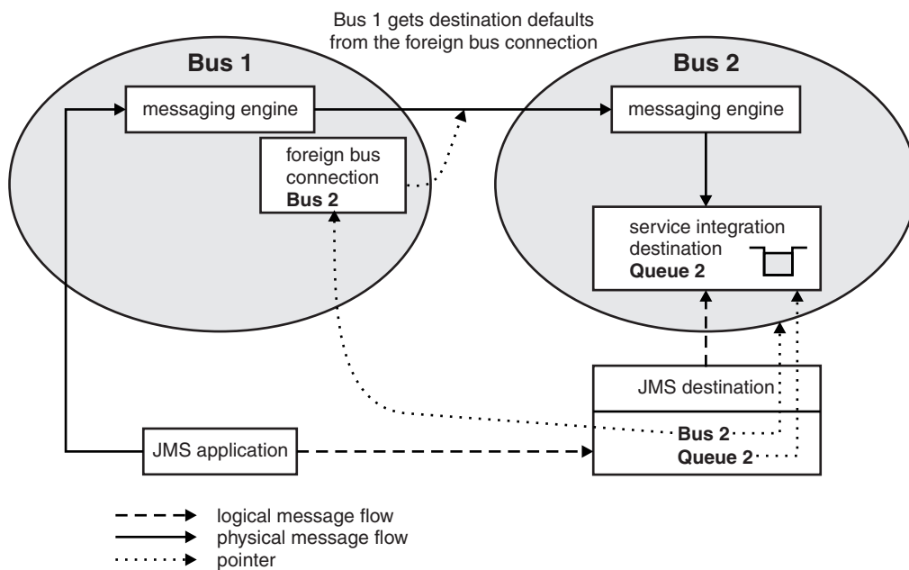
Figure 114. Point-to-point messaging between two buses with no foreign destination configured
