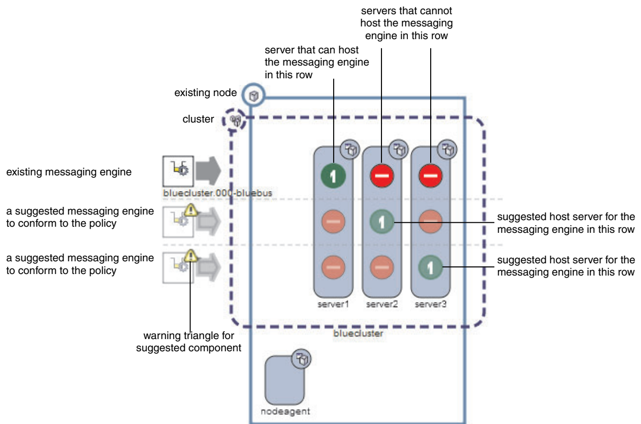
Figure 156. Scalability policy selected without a suitable messaging engine configuration
