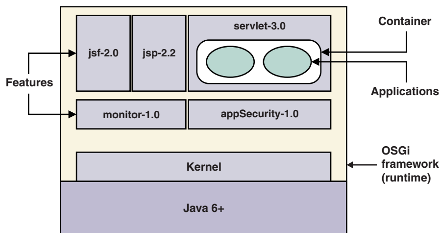
Figure 35. Liberty profile architecture
