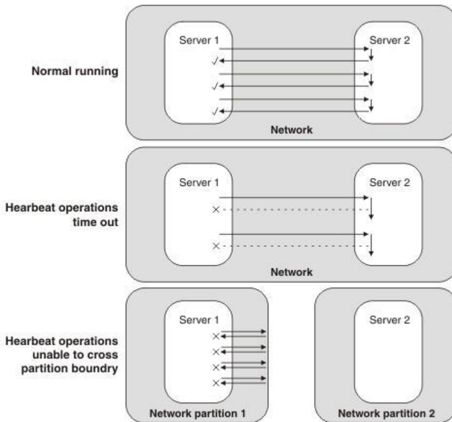
Figure 17. Heartbeats in a system running normally, compared to heartbeats after the apparent server failures of system overloading and network partitioning
