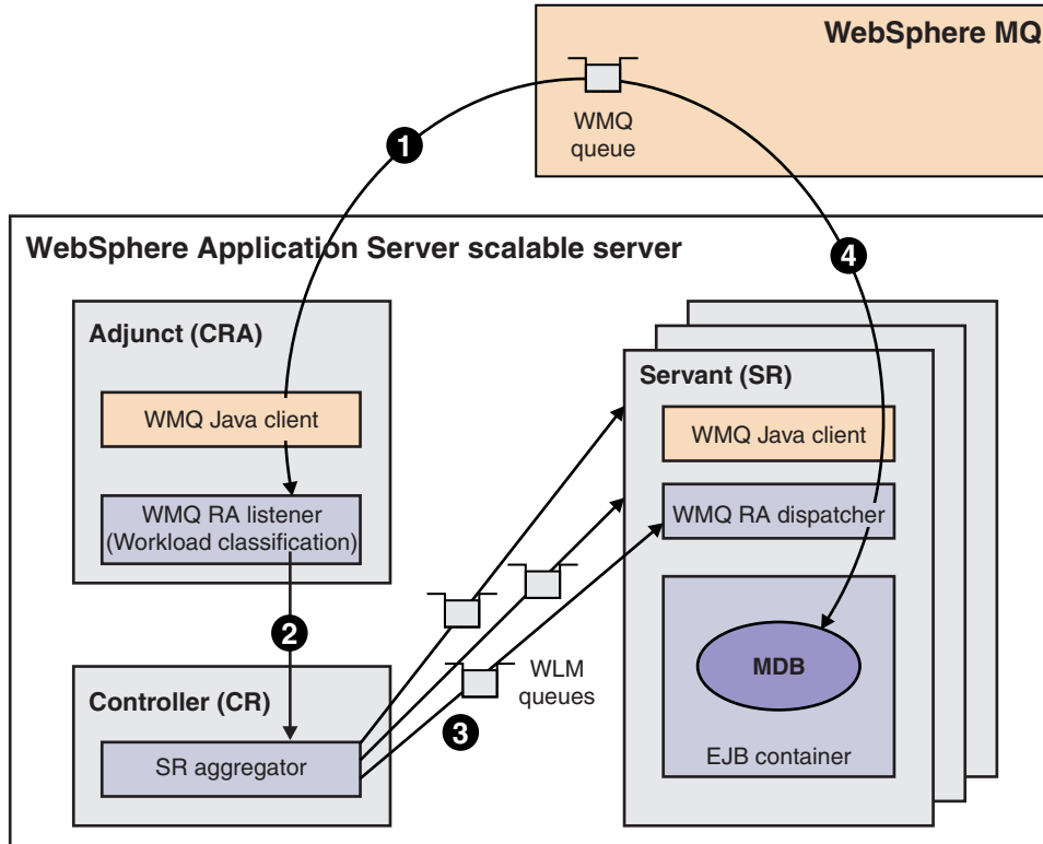
Figure 95. WebSphere MQ: message-driven bean processing
