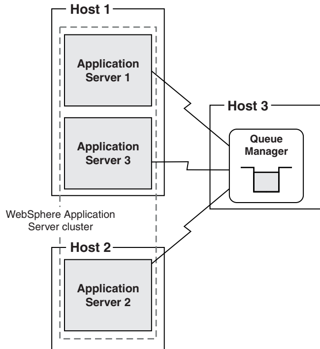
Figure 56. WebSphere Application Server clustering: client mode attachment to queue manager
