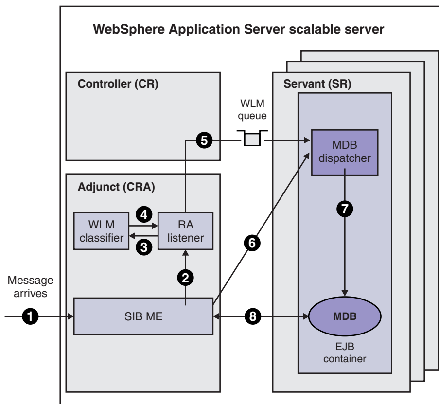
Figure 94. Service integration bus: message-driven bean processing
