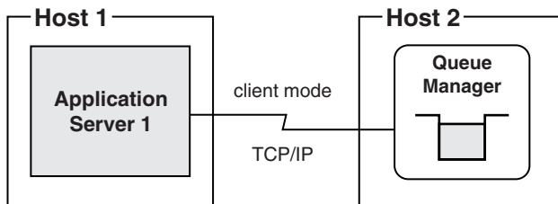
Figure 54. No clustering: client mode attachment to queue manager
