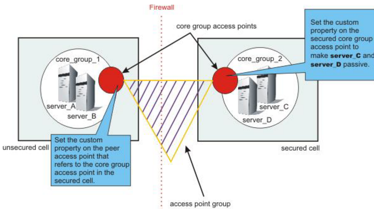
Figure 10. Configuring the FW_PASSIVE_MEMBER custom property
