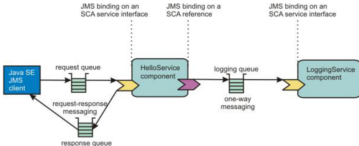
Figure 2. SCA JMS binding example
