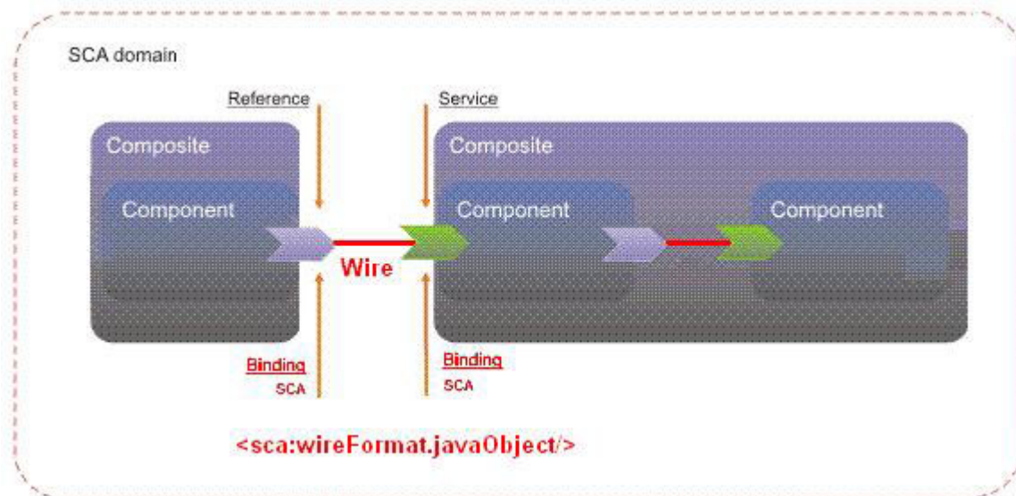
Figure 1. For non-JAXB serializable objects, use the wire format javaObject for the SCA default binding
