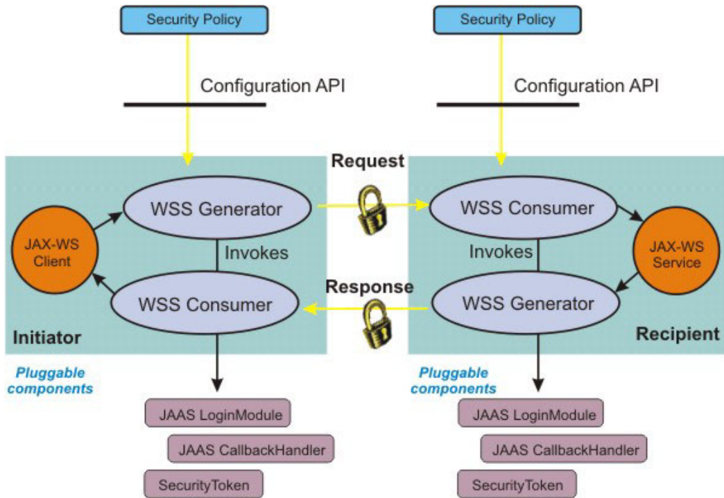
Figure 5. Pluggable token architecture using the JAX-WS programming model
