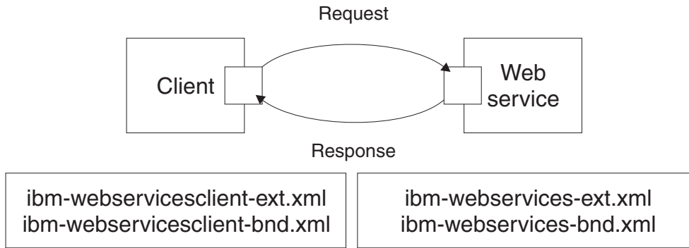
Figure 104. Message flows
